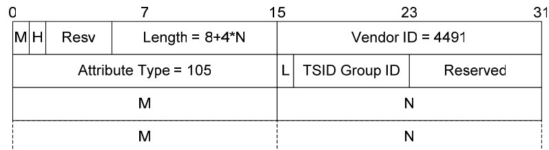
Figure 7–40 - Symbol Rate AVP
