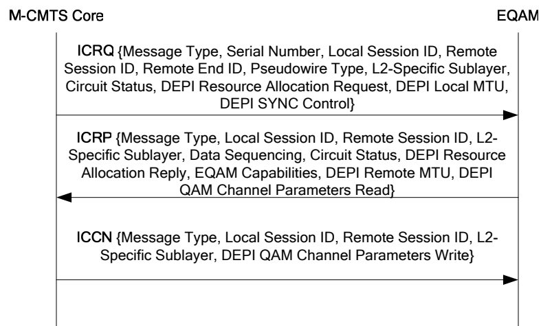
Figure 7-9 - DEPI Session Setup 11
