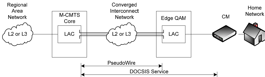
Figure 7-1 - L2TP Topology for Modular CMTS
