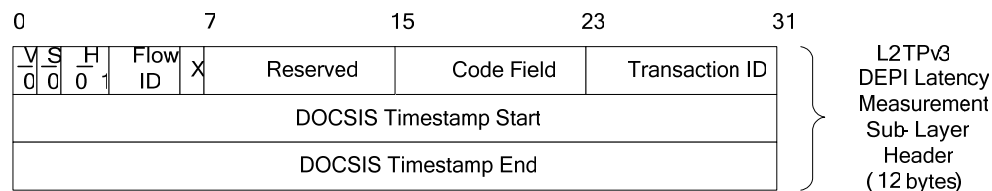
Figure 8–5 - DLM Sub-Layer Header 23
