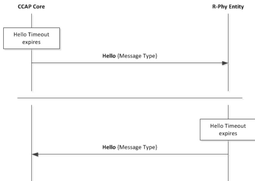
Figure 14 - R-PHY L2TP Keep-alive
