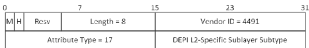
Figure 48 - DEPI L2-Specific Sublayer Subtype AVP
