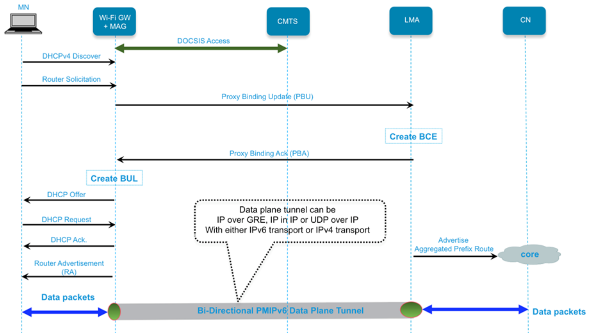
Figure 4 - Sample PMIPv6 Signaling Call Flow
