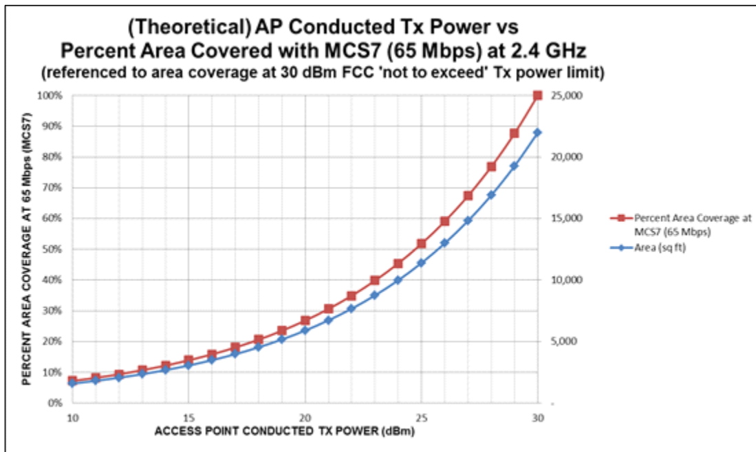
Figure 2 - Theoretical AP Conducted Tx Power vs Percent Area Covered with MCS7 (65 Mbps) at 2.4 GHz
