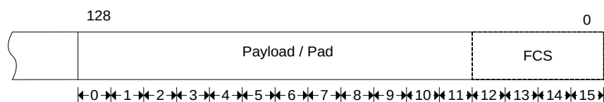
Figure 26 - Octet Order within the Initial Vector (1G)
