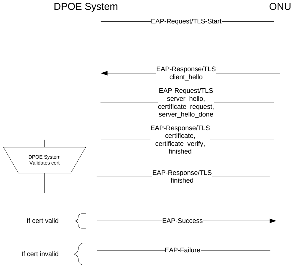
Figure 20 - EAP-TLS Message Sequence
