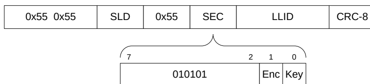
Figure 6 - Security Octet (1Down)
