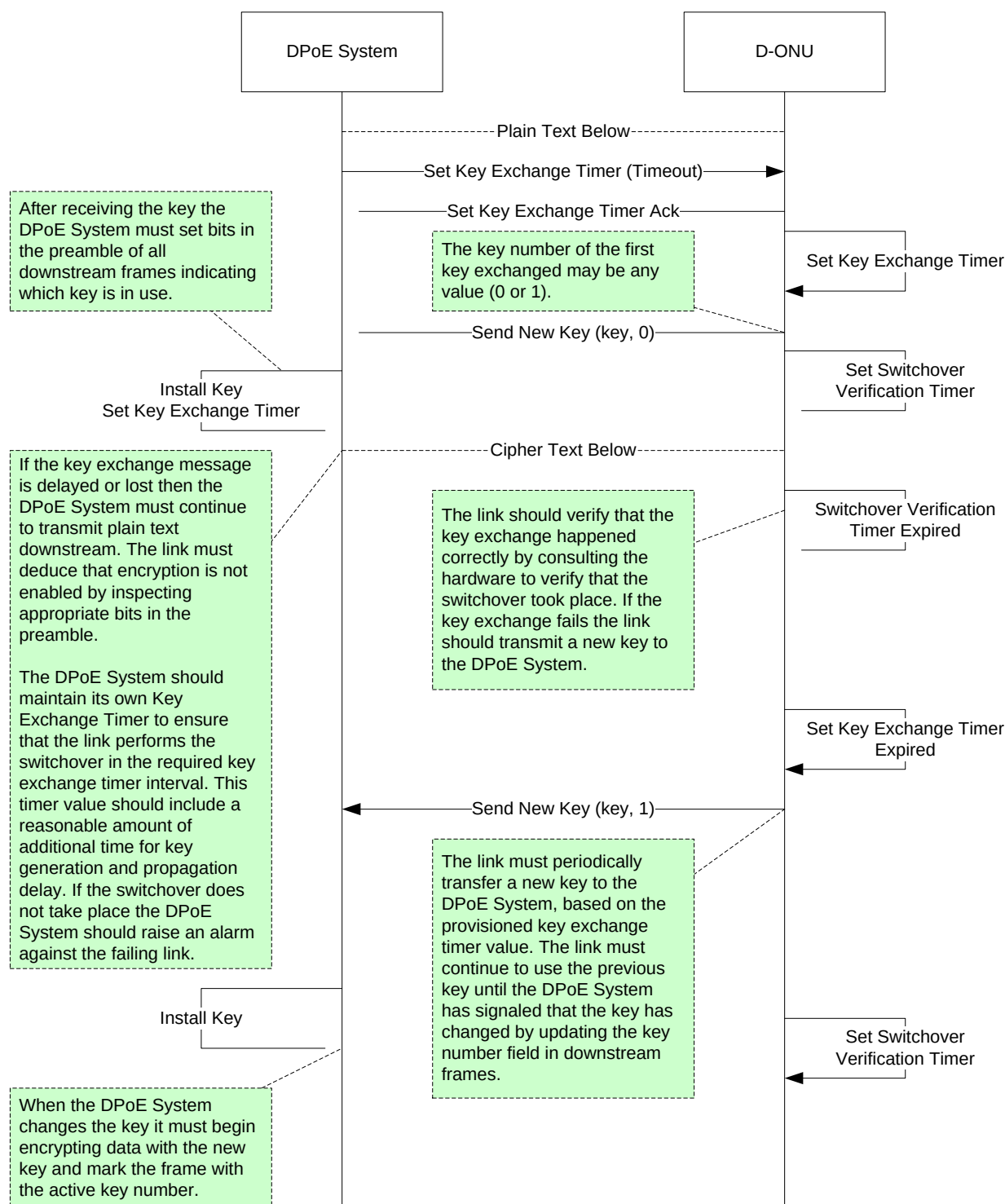
Figure 13 - Changing Keys On Timer Expiration
