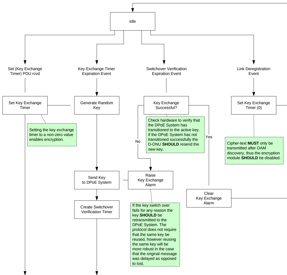
Figure 9 - D-ONU Key Exchange State Machine
