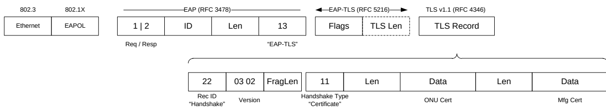
Figure 22 - EAP-TLS Frame Format 2
