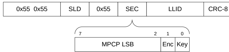
Figure 8 - Security Octet (10G Zero Overhead)
