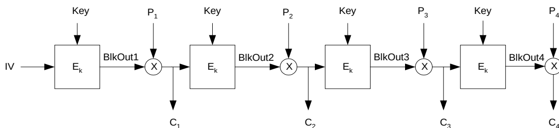
Figure 23 - Encrypting Data with Cipher Feedback Algorithm
