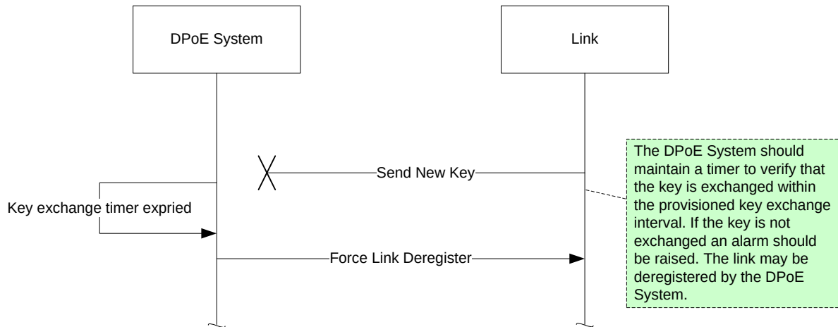
Figure 14 - Key Exchange Failure Detected By DPoE System
