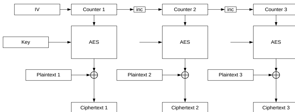
Figure 27 - Encrypting Data with CTR Mode
