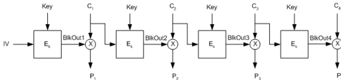
Figure 24 - Decrypting Data with Cipher Feedback Algorithm
