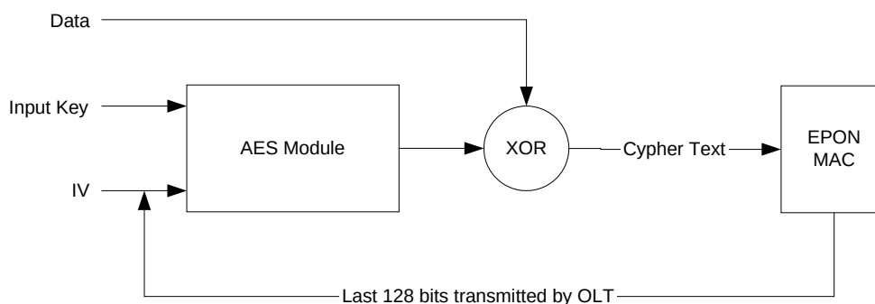
Figure 25 - Determining the Initial Vector
