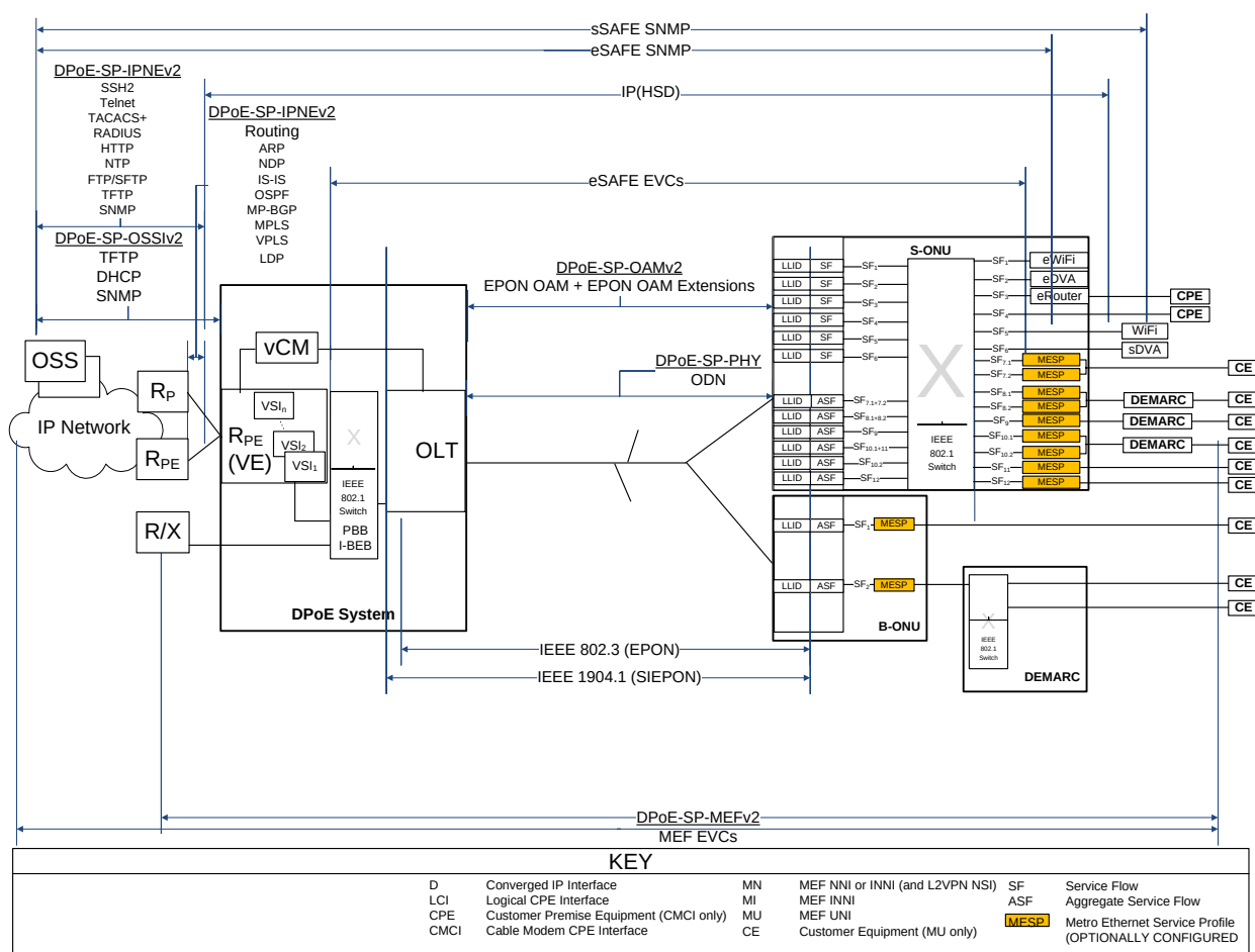
Figure 1 - DPoE 2.0 Reference Architecture 3
