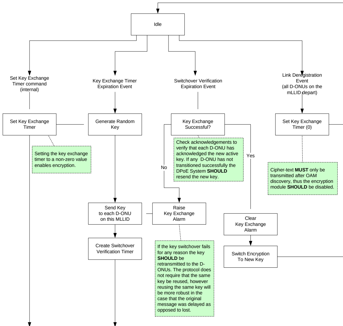
Figure 16 - mLLID Key Exchange DPoE System State Machine
