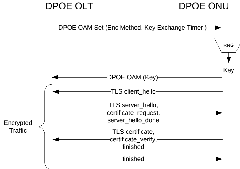
Figure 19 - Authentication in Downstream-Only Methods
