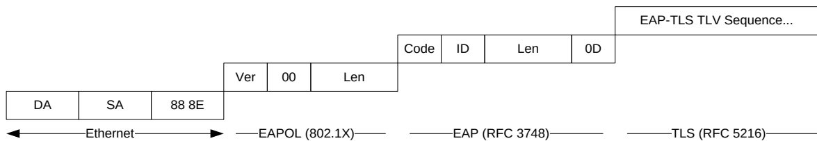
Figure 21 - EAP-TLS Frame Format
