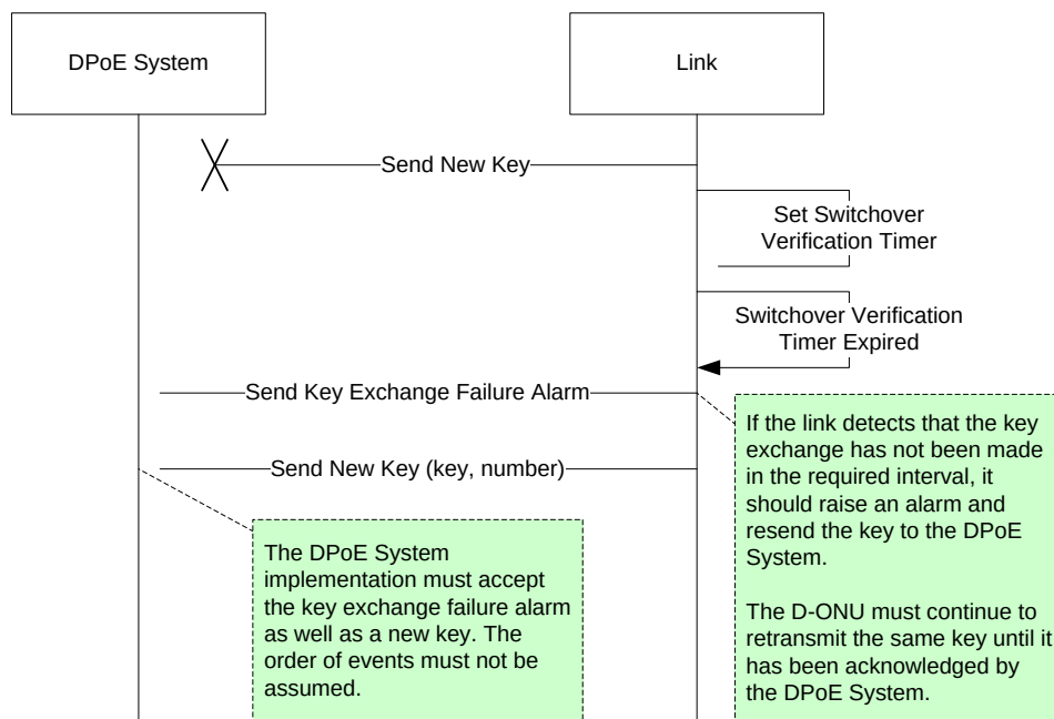
Figure 12 - Key Exchange Failure Detected by Link
