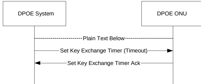
Figure 10 - Setting the Key Exchange Timer
