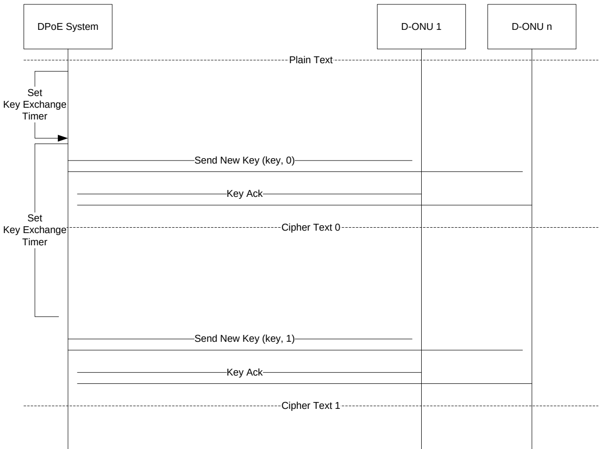
Figure 17 - Sending mLLID Keys to D-ONUs
