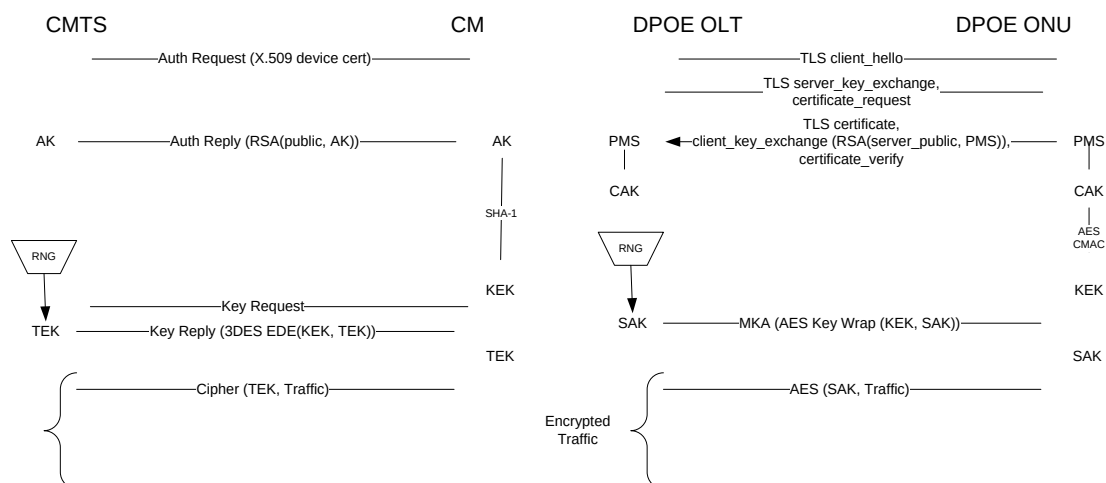
Figure 18 - Authentication in Bidirectional Methods
