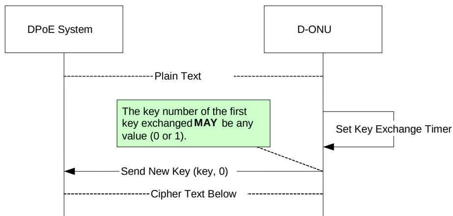
Figure 11 - Send Key to the DPoE System
