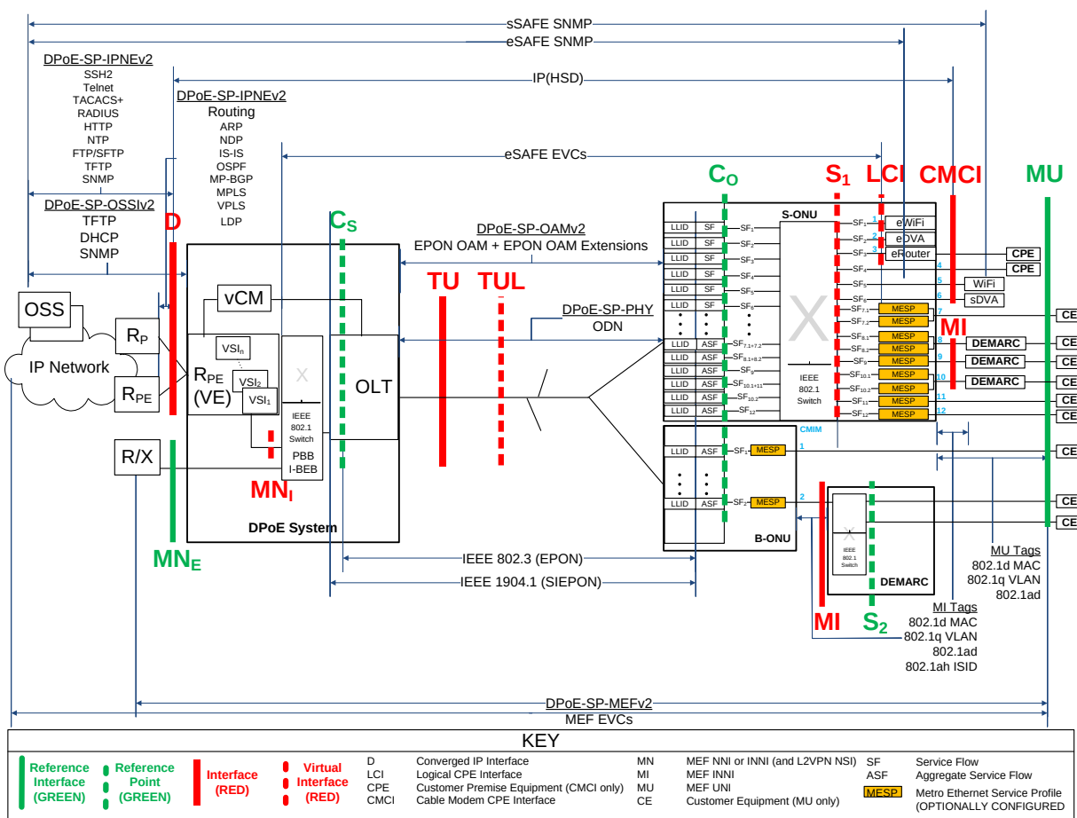
Figure 2 - DPoE 2.0 Interfaces and Reference Points 4
