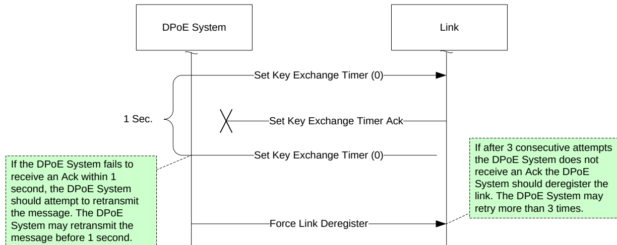
Figure 15 - Set Key Exchange Timer Failure Detected by DPoE System
