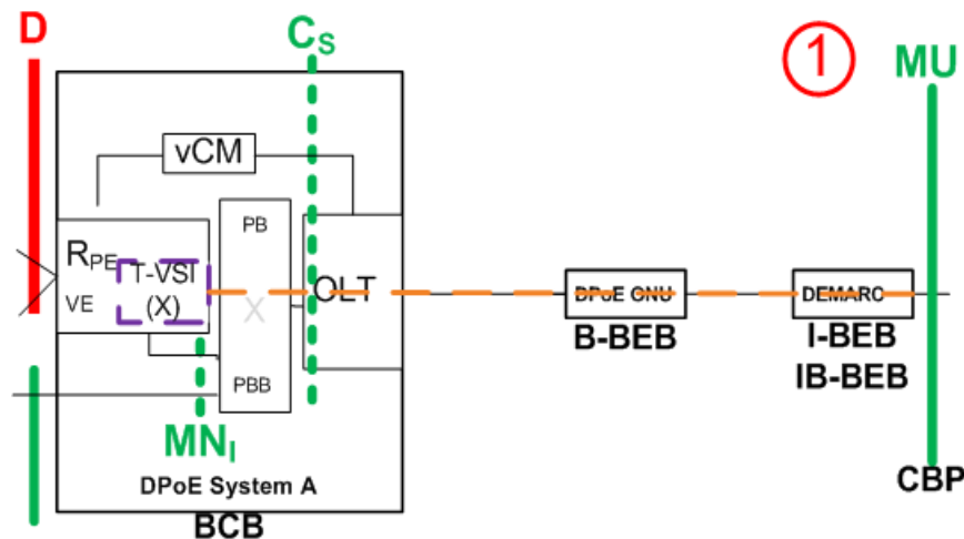
Figure 16 - DPoE-PBB-DEMARC
