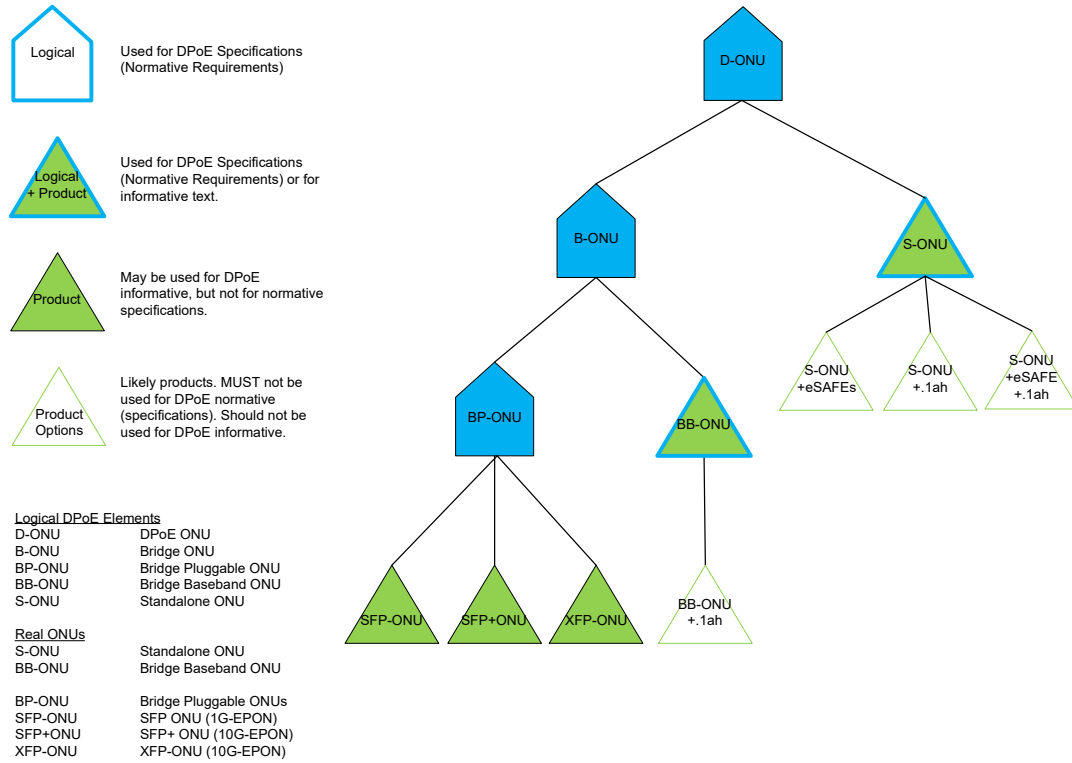
Figure 3 - D-ONU Types
