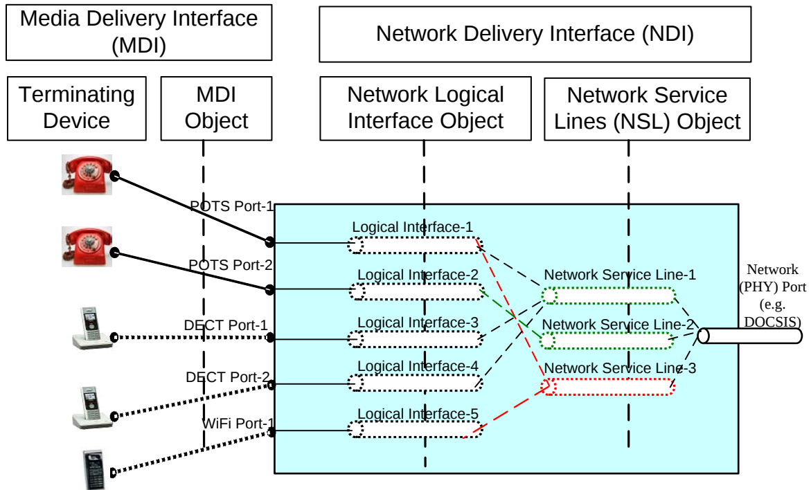
Figure 3 - PacketCable HDV Client Abstraction Model (general case)
