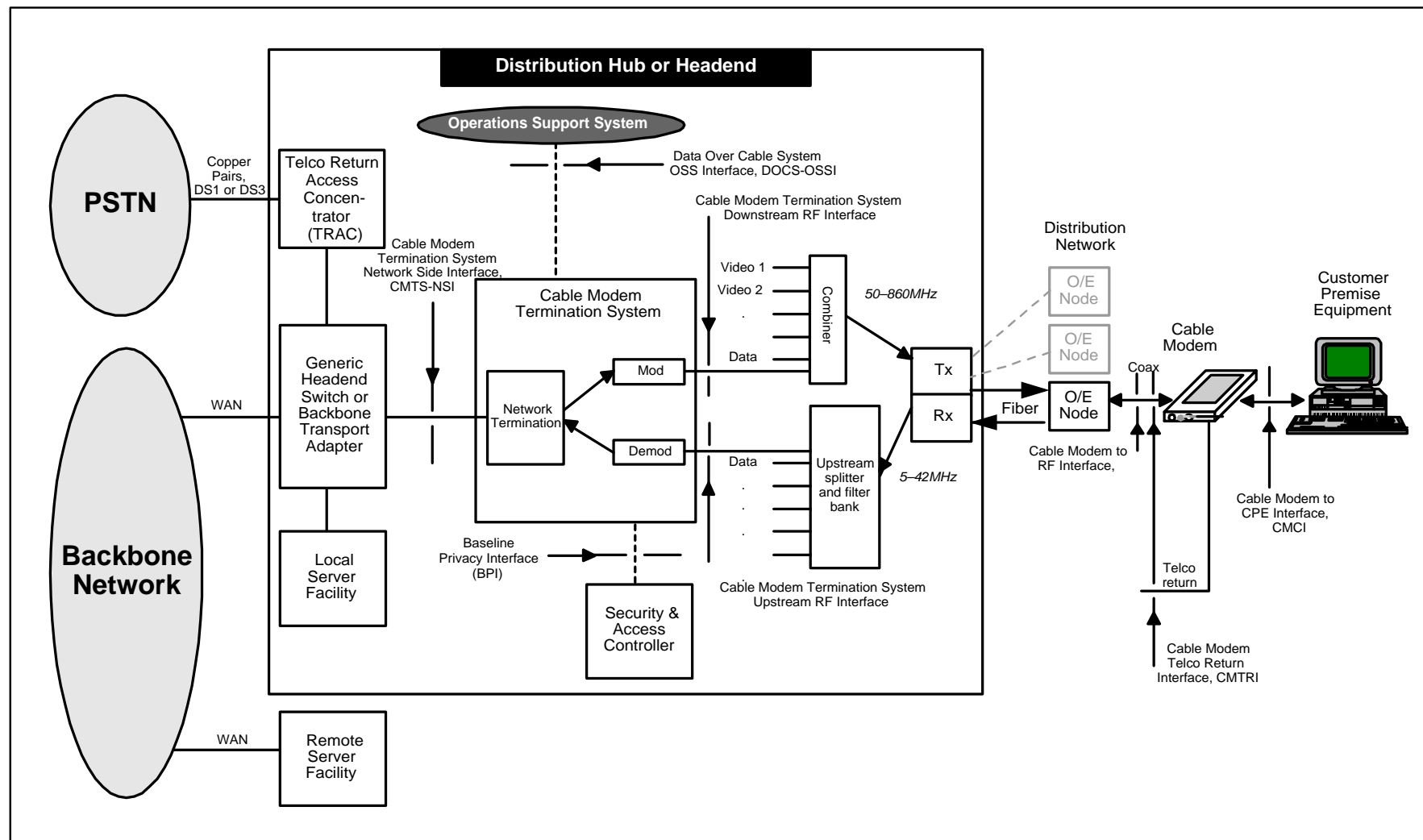
Figure 1-2 Data-Over-Cable Reference Architecture
