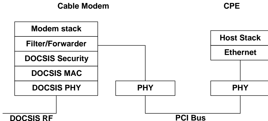
Figure 3-9 CM-to-MAC Forwarding
