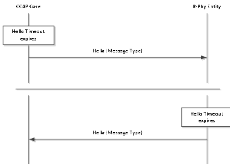
Figure 7–9 - R-PHY L2TP Keep-alive
