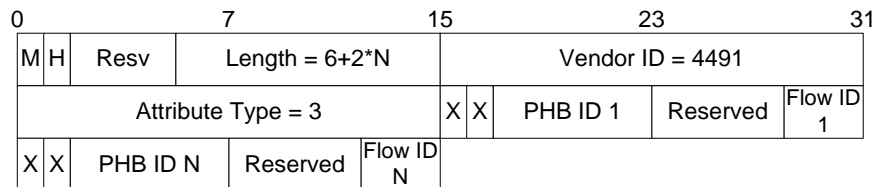
Figure 7–33 - DEPI Resource Allocation Reply AVP
