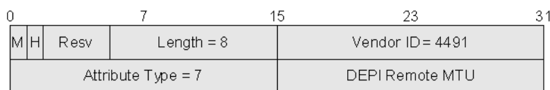
Figure 7–35 - DEPI Remote MTU Max Payload AVP
