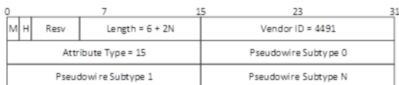
Figure 7-30 - DEPI Pseudowire Subtype Capabilities List AVP
