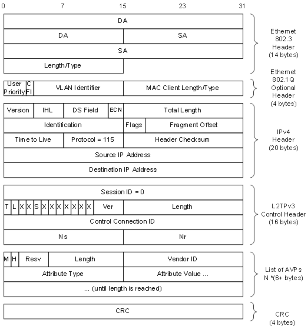
Figure 7–5 - L2TP Control Message without UDP Header
