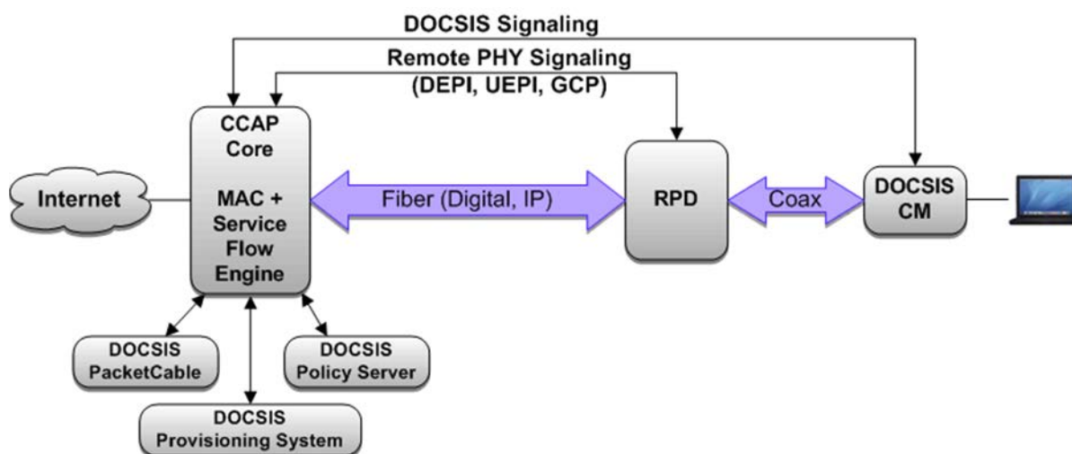
Figure 5–1 - MHA v2 / R-PHY System Architecture
