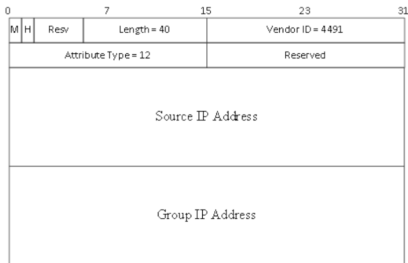
Figure 7–38 - DEPI Remote Multicast Leave AVP
