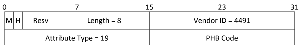
Figure 7-44 - DEPI S-BFD Return Path DSCP AVP
