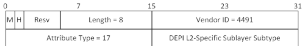
Figure 7-42 - DEPI L2-Specific Sublayer Subtype AVP 41
