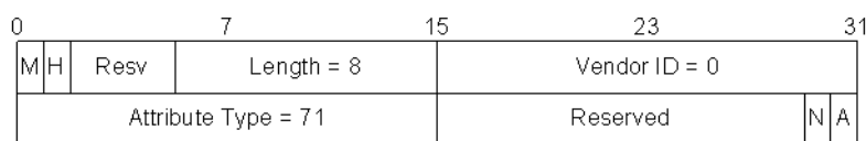
Figure 7–29 - Circuit Status AVP
