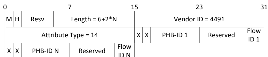
Figure 7–40 - Upstream Flow AVP
