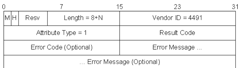
Figure 7–31 - DEPI Result and Error Code AVP
