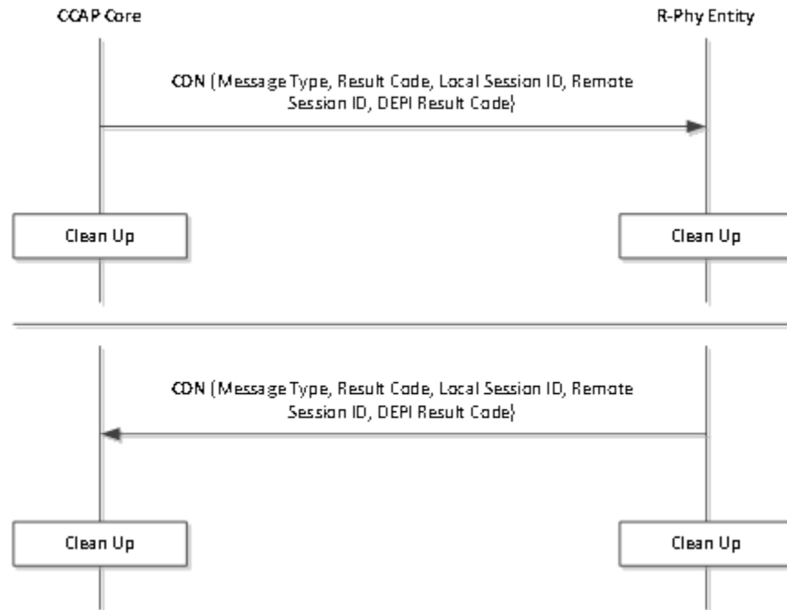
Figure 7–11 - R-PHY Session Teardown
