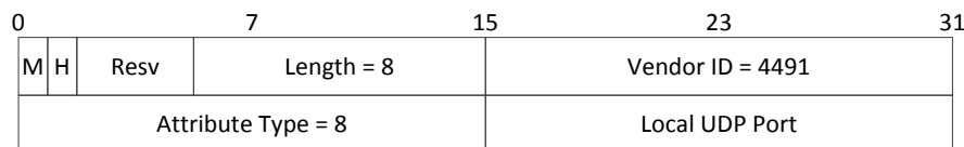
Figure 7-36 - DEPI Local UDP Port AVP
