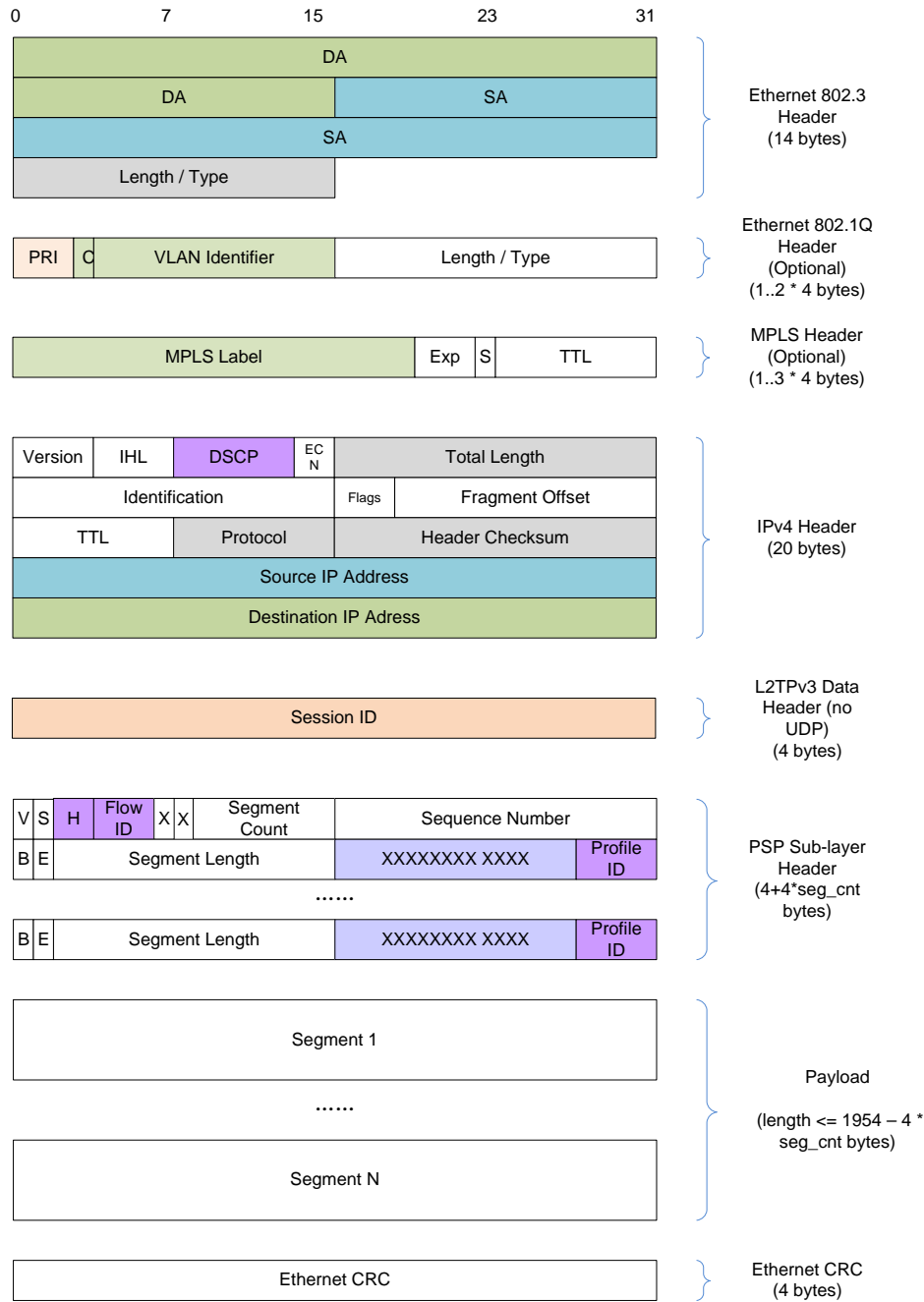
Figure 8-8 - Example of a Complete DEPI Packet Format (IPv4) with Extras 55
