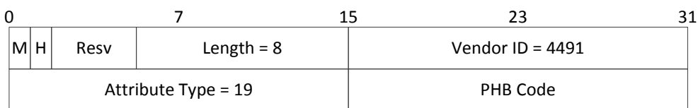
Figure 7-43 - DEPI DLM Response DSCP AVP
