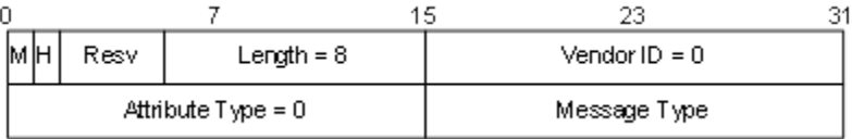
Figure 7–13 - Message Type AVP
