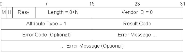
Figure 7–14 - Result Code AVP
