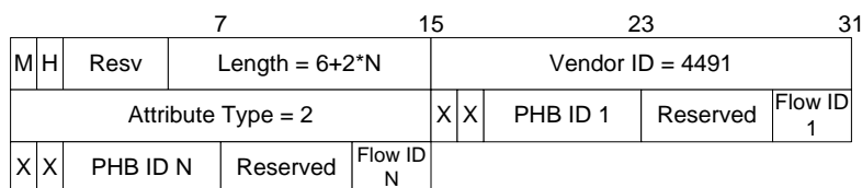
Figure 7–32 - DEPI Resource Allocation Request AVP
