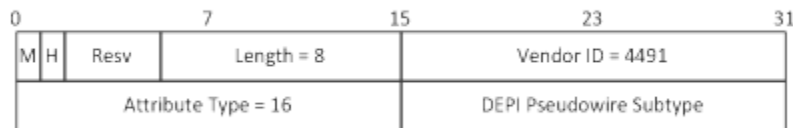
Figure 7-41 - DEPI Pseudowire Subtype AVP
