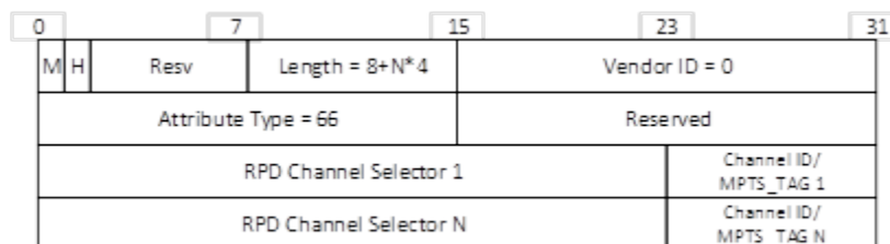
Figure 7–24 - Remote End ID AVP
