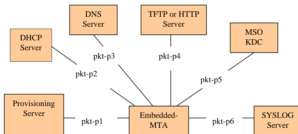
Figure 3. PacketCable Provisioning Interfaces
