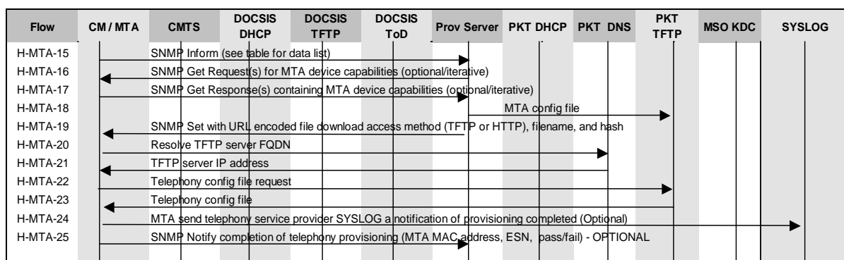
Figure 9. Embedded-MTA Hybrid Power-on Initialization Flow
