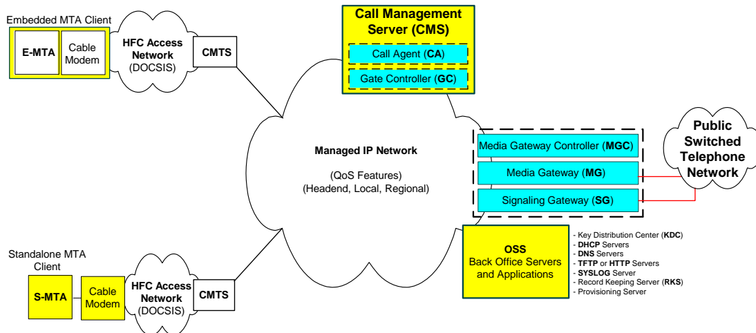
Figure 2. PacketCable 1.0 Network Component Reference Model
