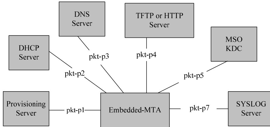
Figure 3. PacketCable Provisioning Interfaces
