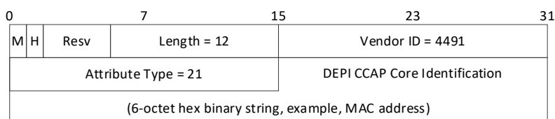
Figure 36 - DEPI Specific Message Type AVP
