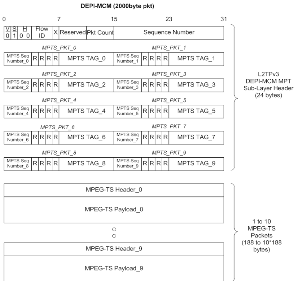
Figure 59 - MCM Sublayer Header and Payload
