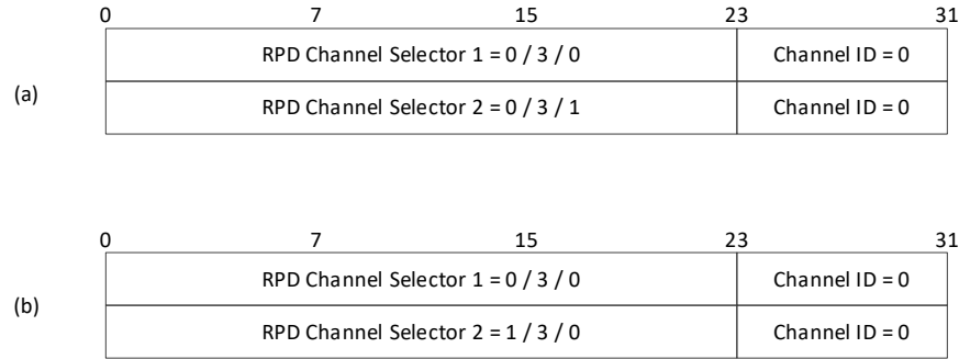
Figure 31 - Remote End ID Example for RPD Channel Replication
