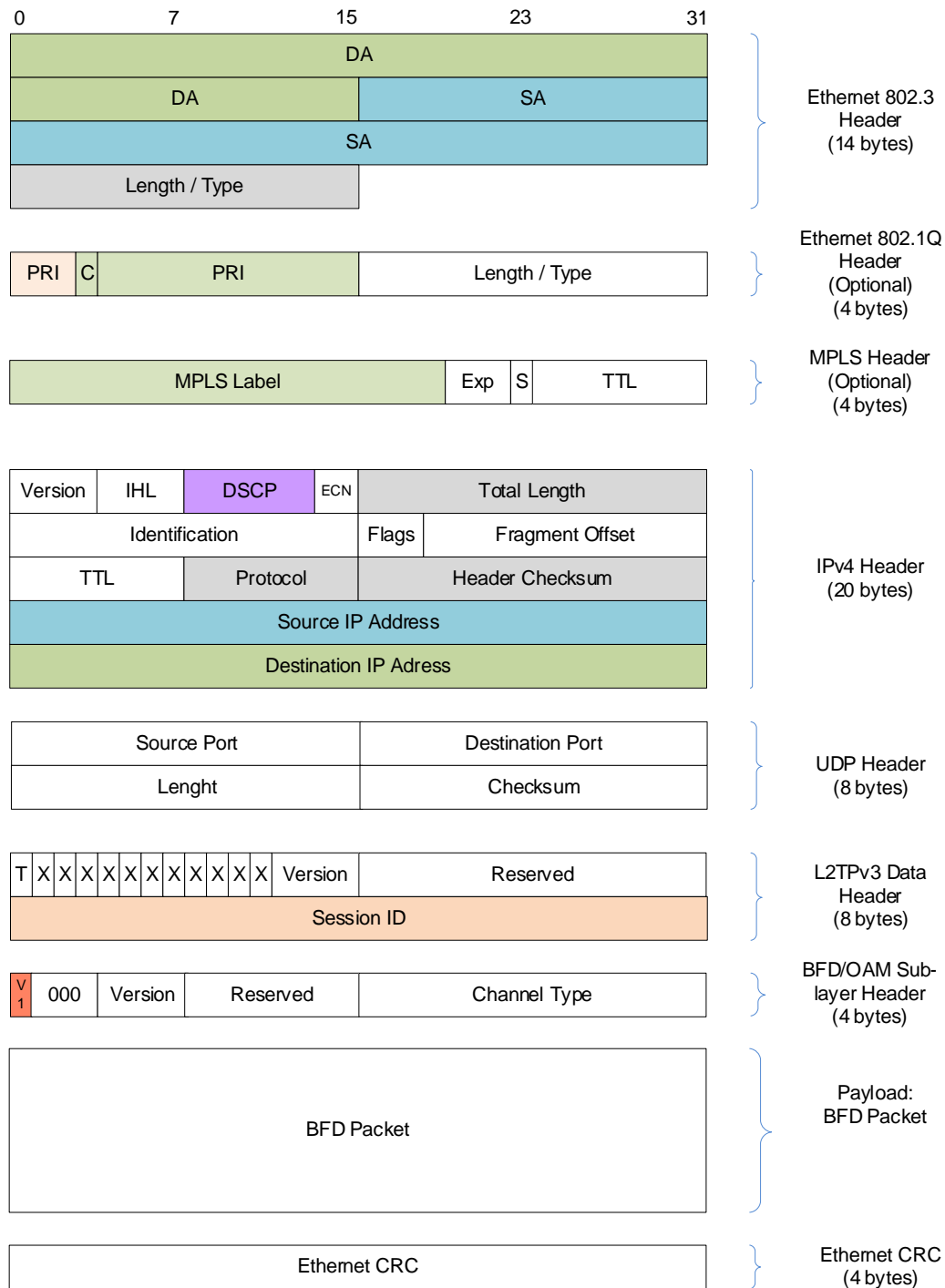
Figure 65 - BFD Sublayer (with UDP)
