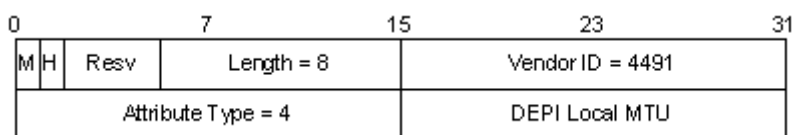
Figure 45 - DEPI Local MTU AVP
