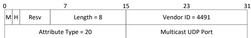
Figure 55 - DEPI Multicast UDP Port AVP
