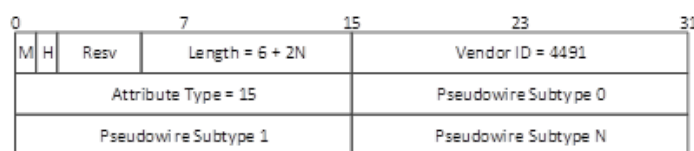
Figure 37 - DEPI Pseudowire Subtype Capabilities List AVP
