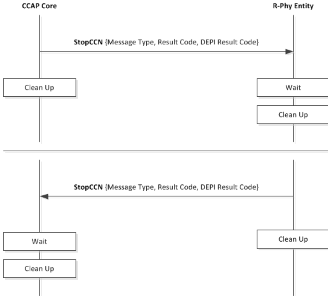
Figure 13 - R-PHY L2TP Control Connection Teardown
