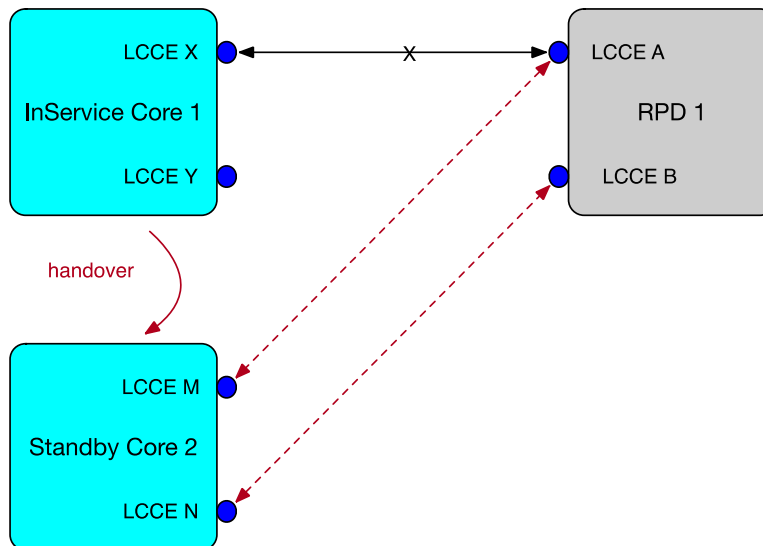
Figure 69 - Active and Standby Tunnels
