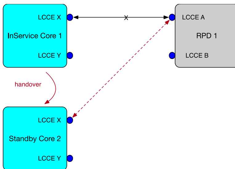
Figure 70 - Standby Core using Identical IP /LCCE Addressing
