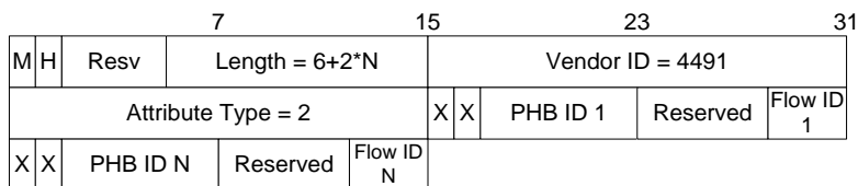
Figure 43 - DEPI Resource Allocation Request AVP
