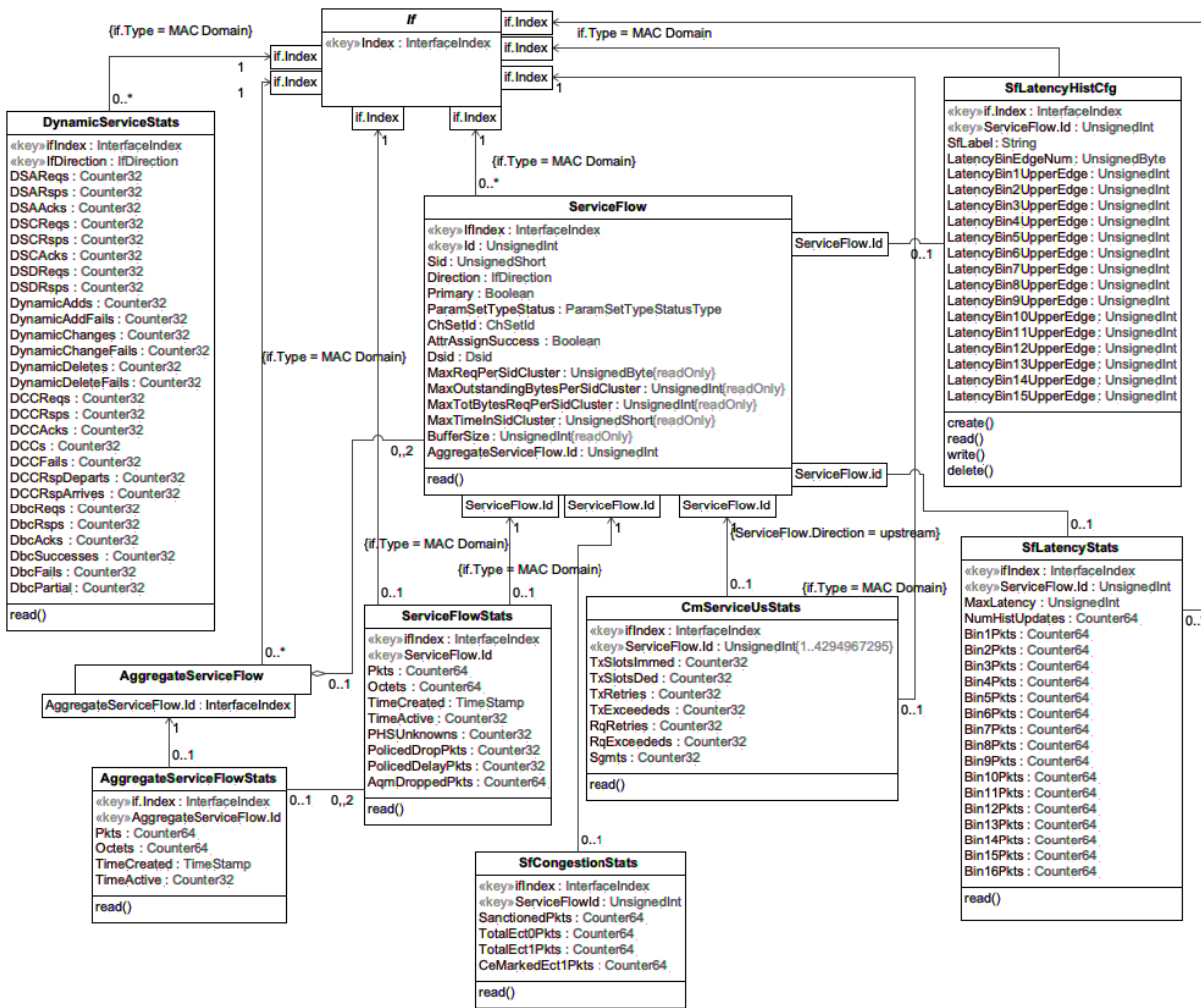
Figure 20 - QoS Statistics Information Model
