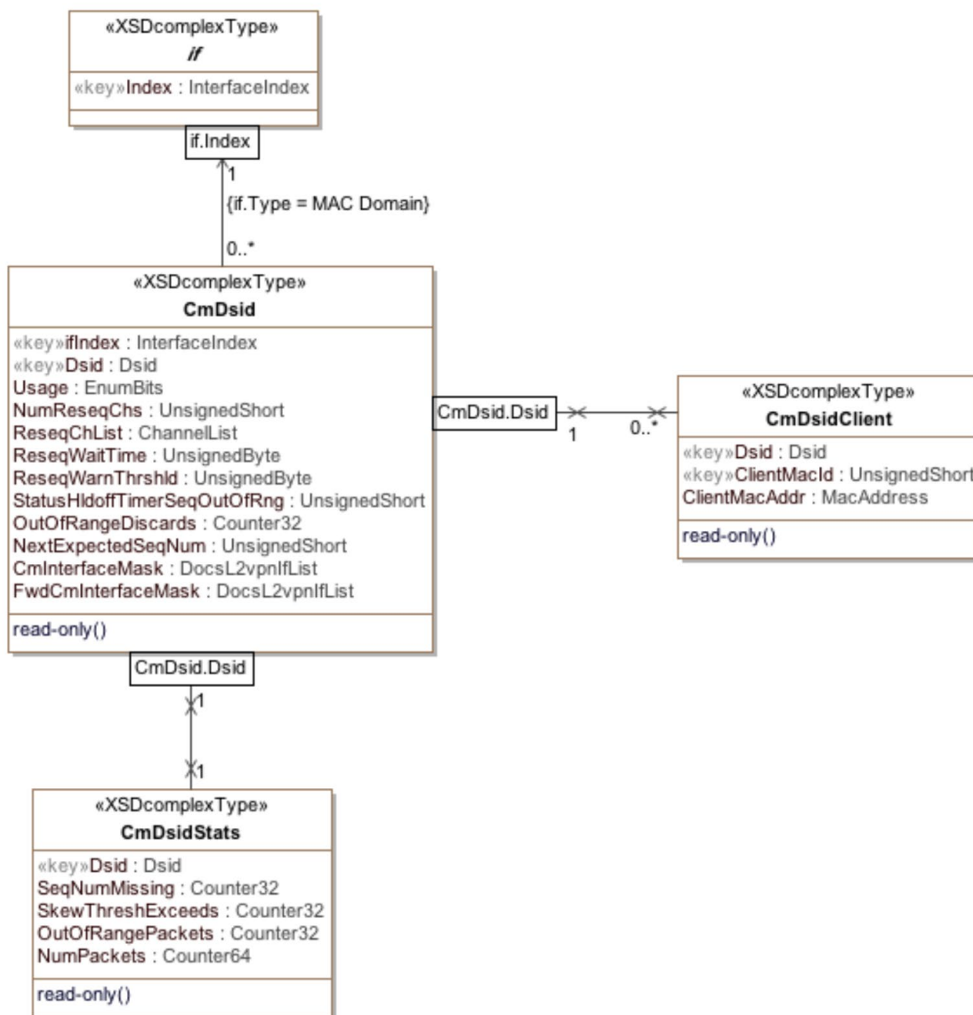
Figure 21 - DSID Information Model
