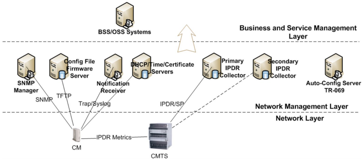
Figure 4 - CM Management Architecture
