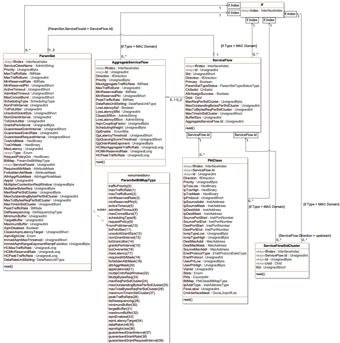
Figure 19 - QoS Configuration Status Information Model
