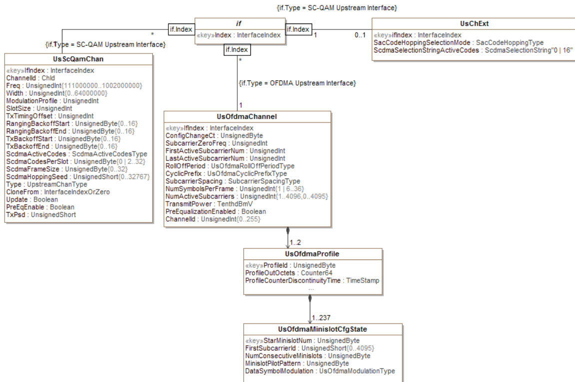
Figure 16 - CM Upstream Information Model
