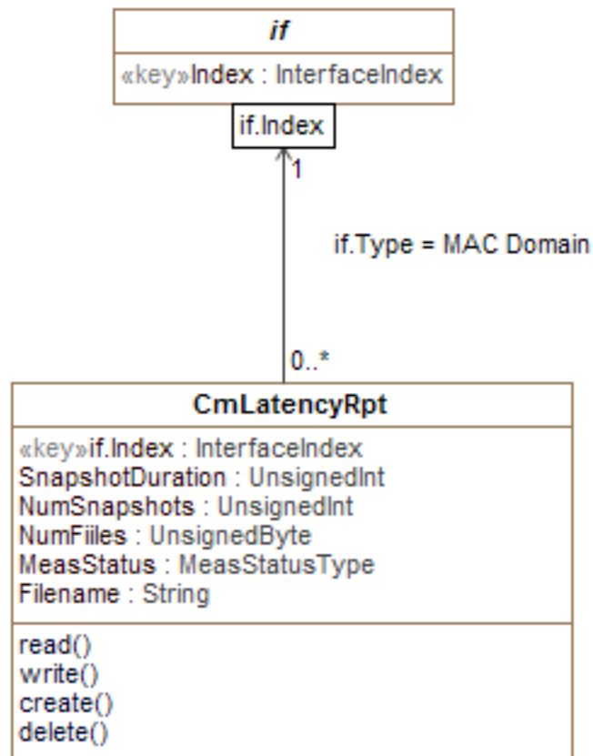
Figure 10 - Latency Report Information Model
