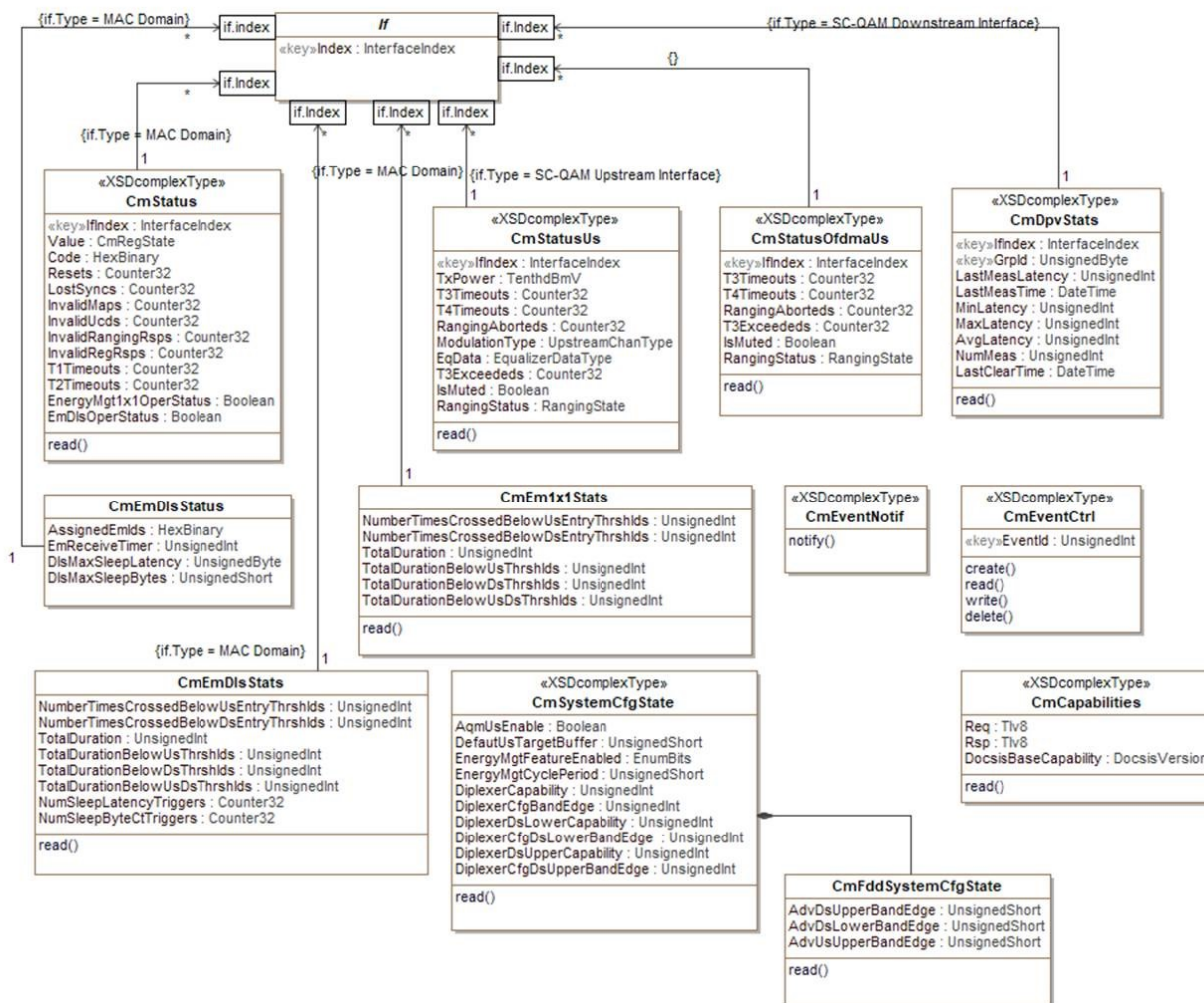
Figure 14 - CM Operational Status Information Model
