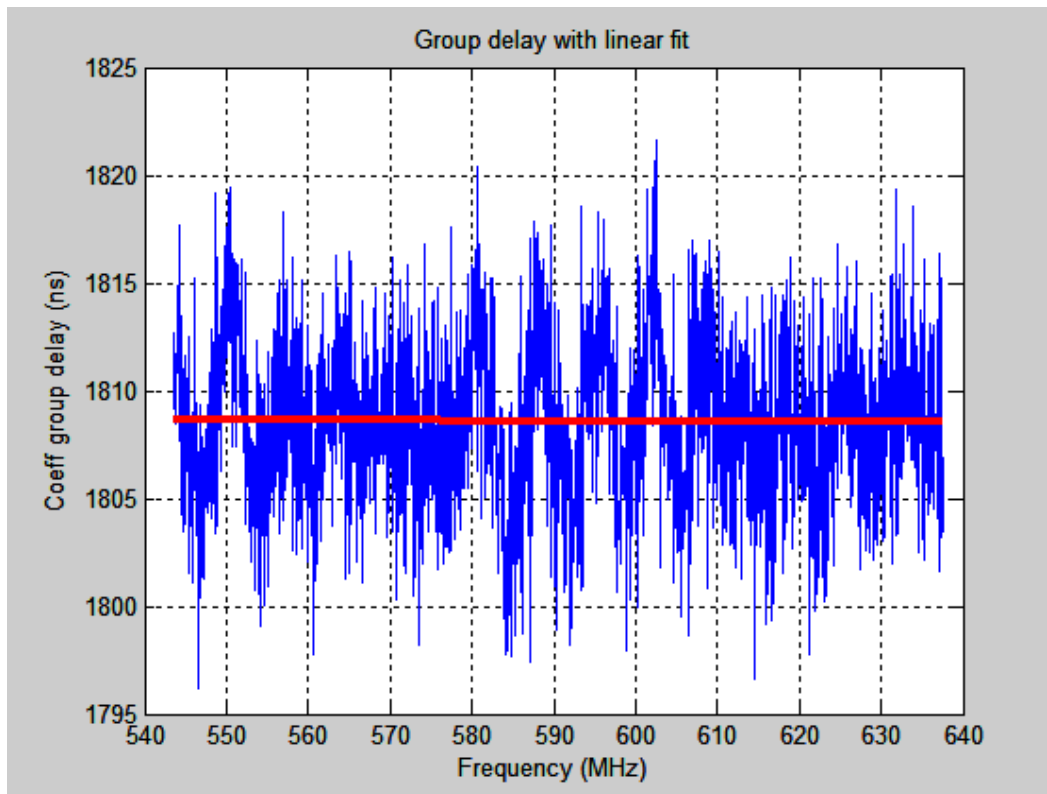
Figure 12 - Group Delay Response Of Channel Estimate Coefficients, With Best-Fit Line
