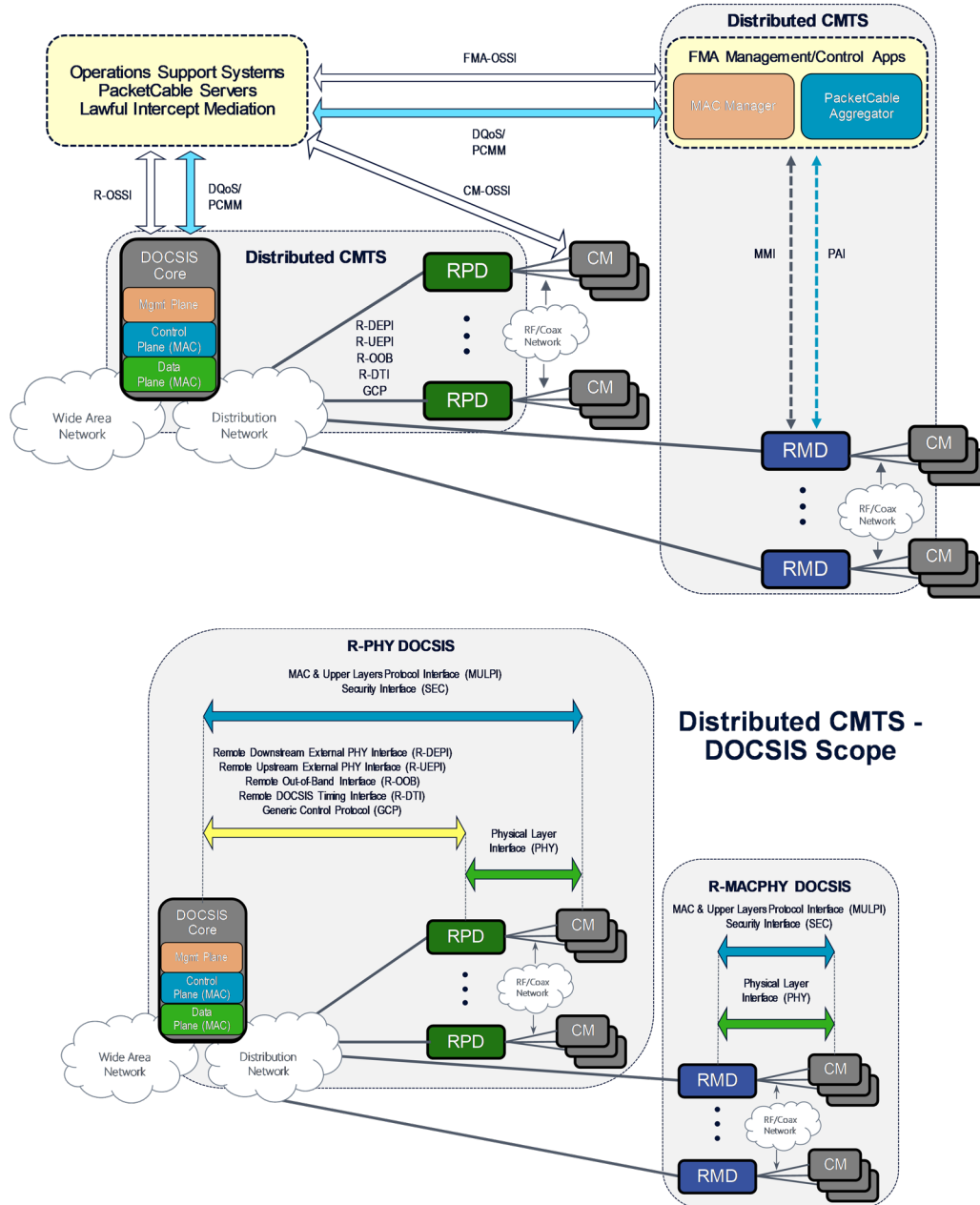
Figure 3 - Data-Over-Cable Reference Architecture
