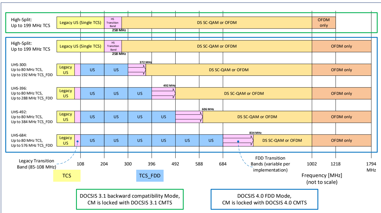
Figure 25 - Configurable FDD Upstream Allocated Spectrum Bandwidths
