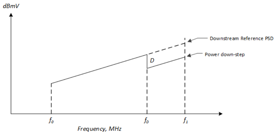
Figure 9 - Downstream Power Profile with D dB Step-down at f_0 MHz
