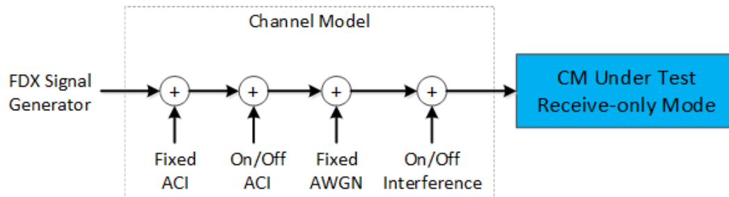
Figure 11 - Test Set-up for External ACI Test
