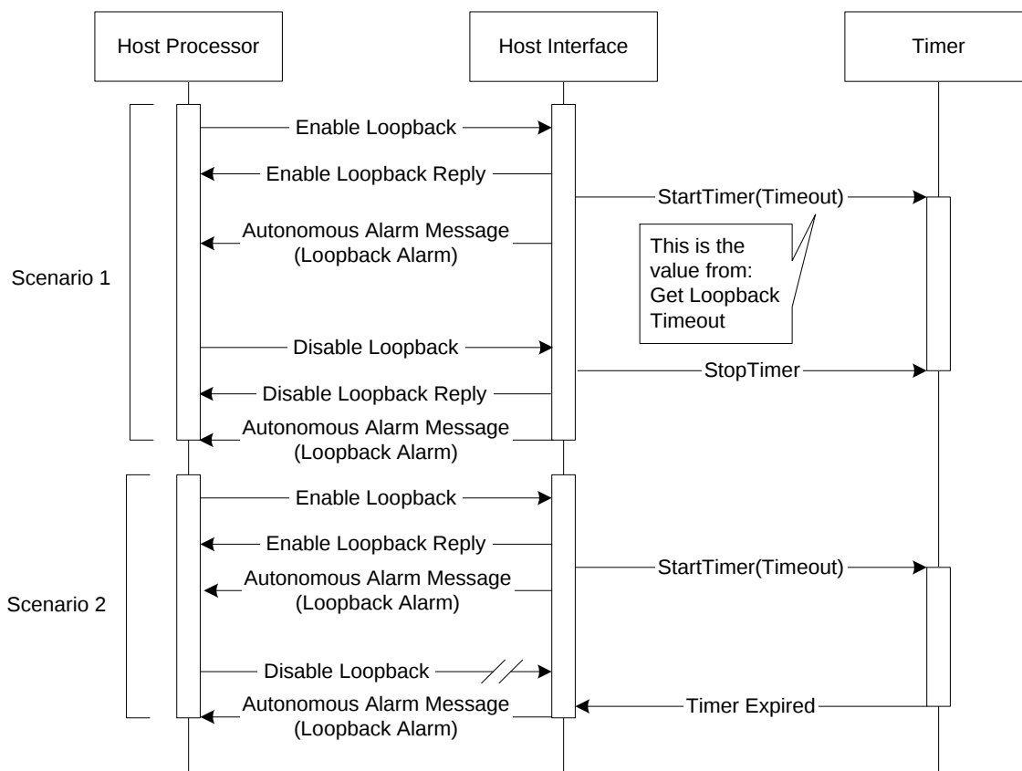
Figure 18 - Enable/Disable Loopback
