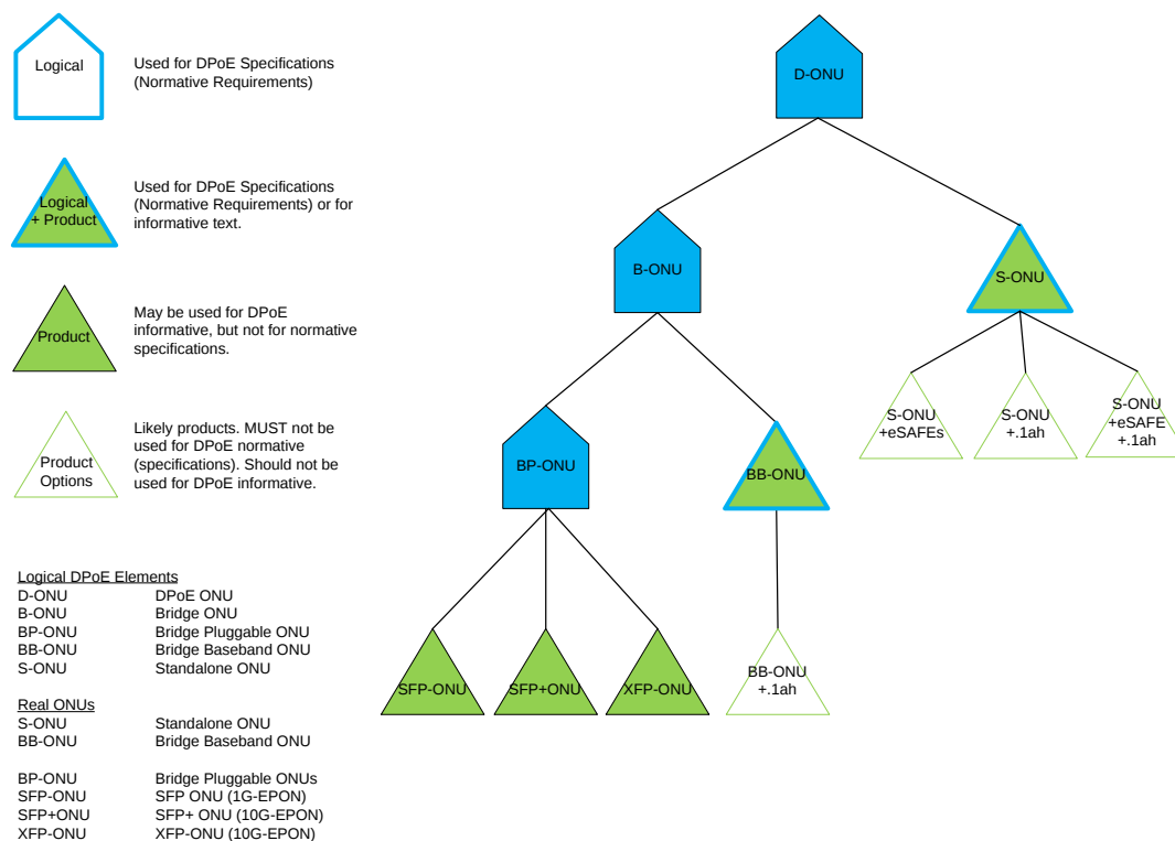
Figure 3 - D-ONU Types
