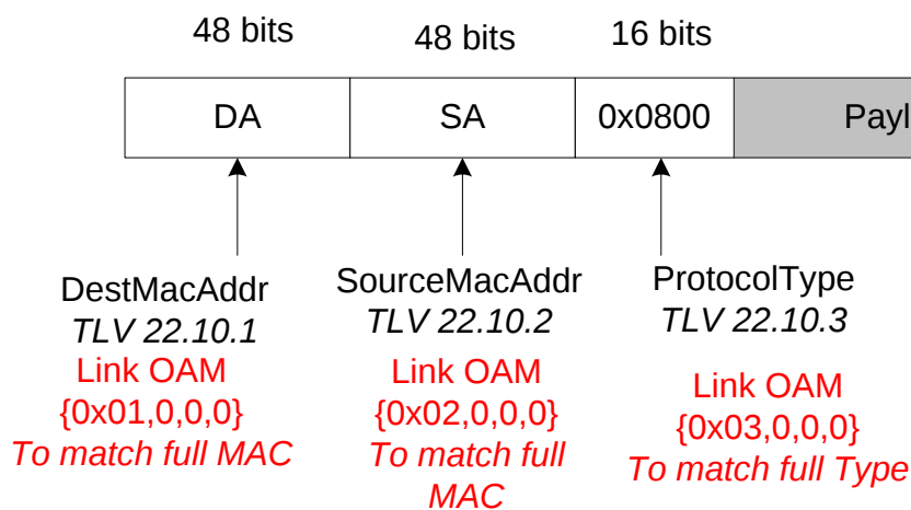
Figure 28 - Field Masking Example for Untagged Frame
