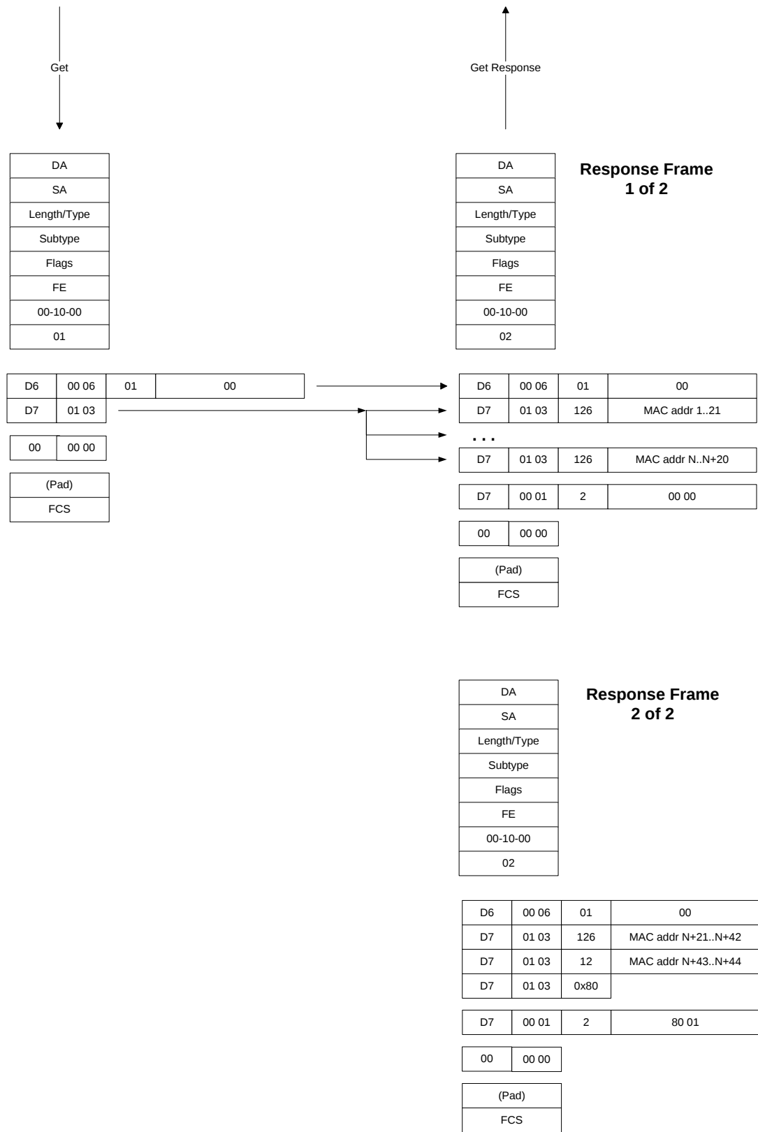
Figure 22 - Multi-Part Replies
