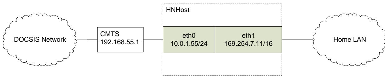
Figure 2 - Auto-IP on LAN Reference Network
