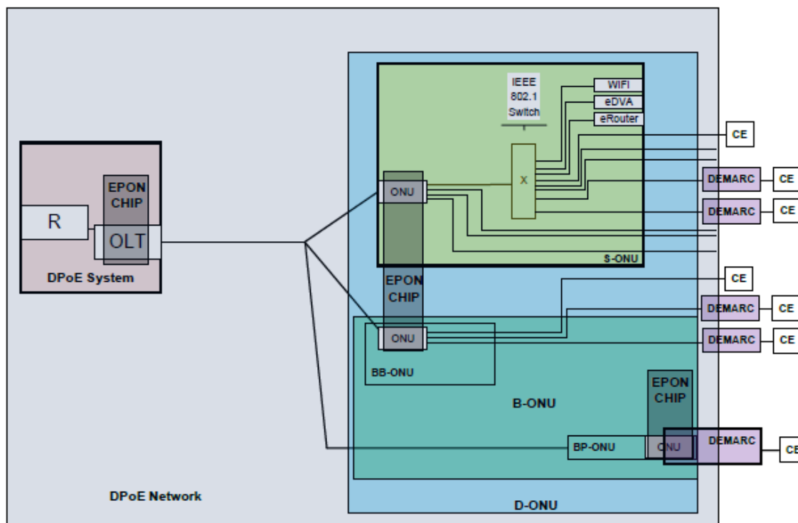
Figure 4 - DPoE Network Elements
