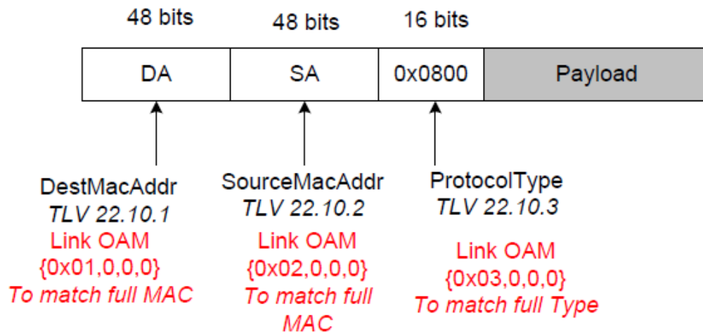
Figure 28 - Field Masking Example for Untagged Frame
