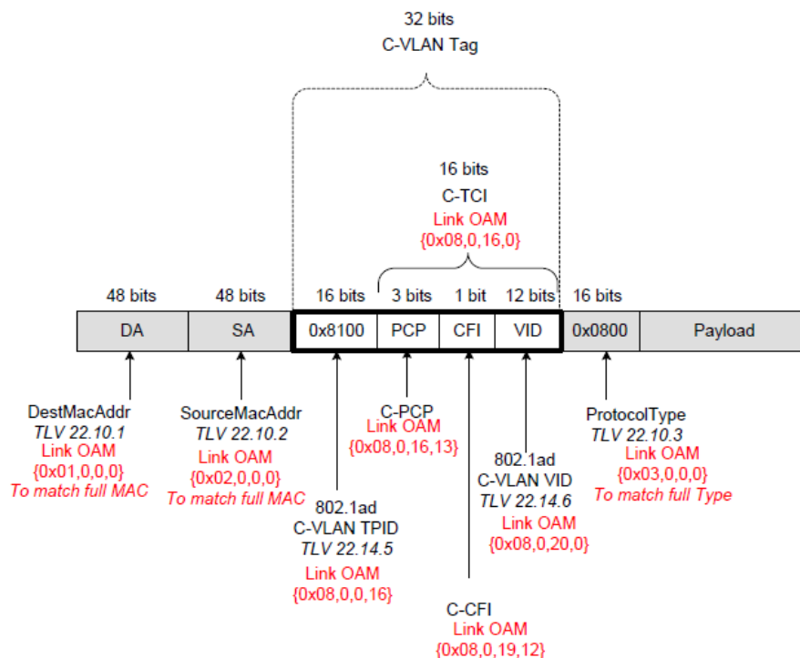
Figure 29 - Field Masking Example for 802.1Q C-tagged Frame
