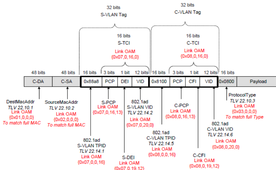
Figure 30 - Field Masking Example for 802.1ad Tagged Frame
