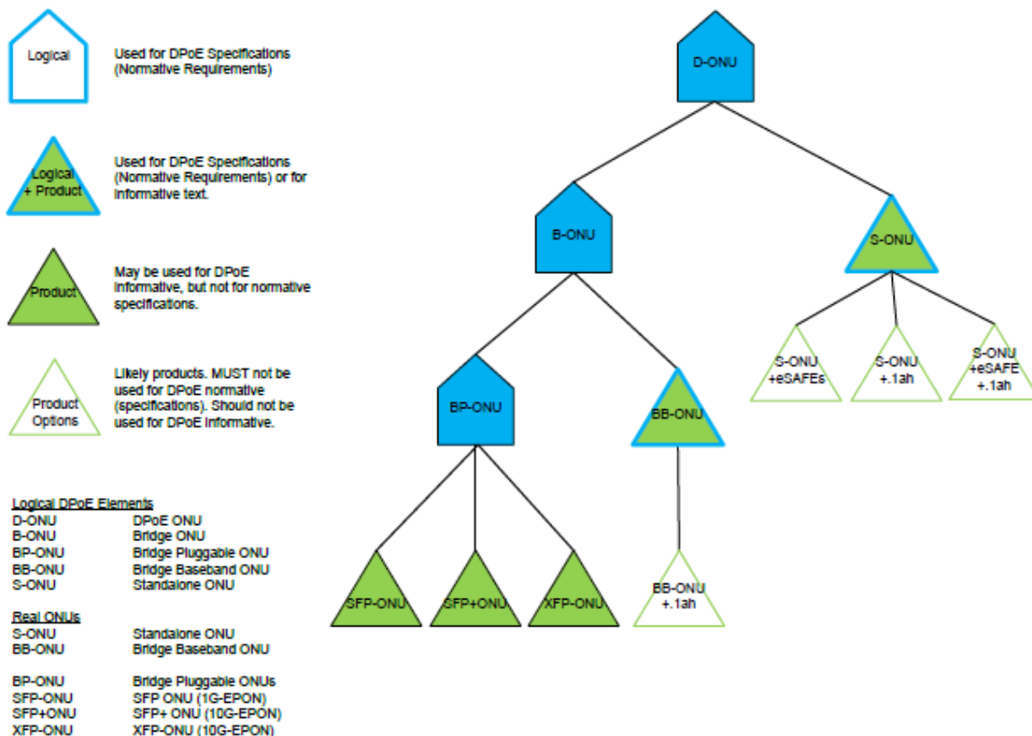
Figure 3 - D-ONU Types
