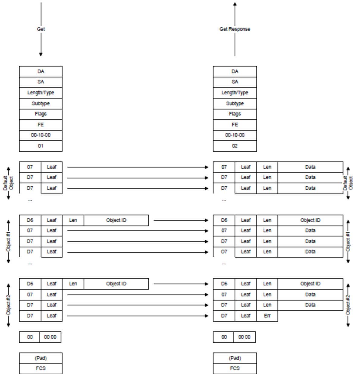
Figure 19 - Get and Get Response
