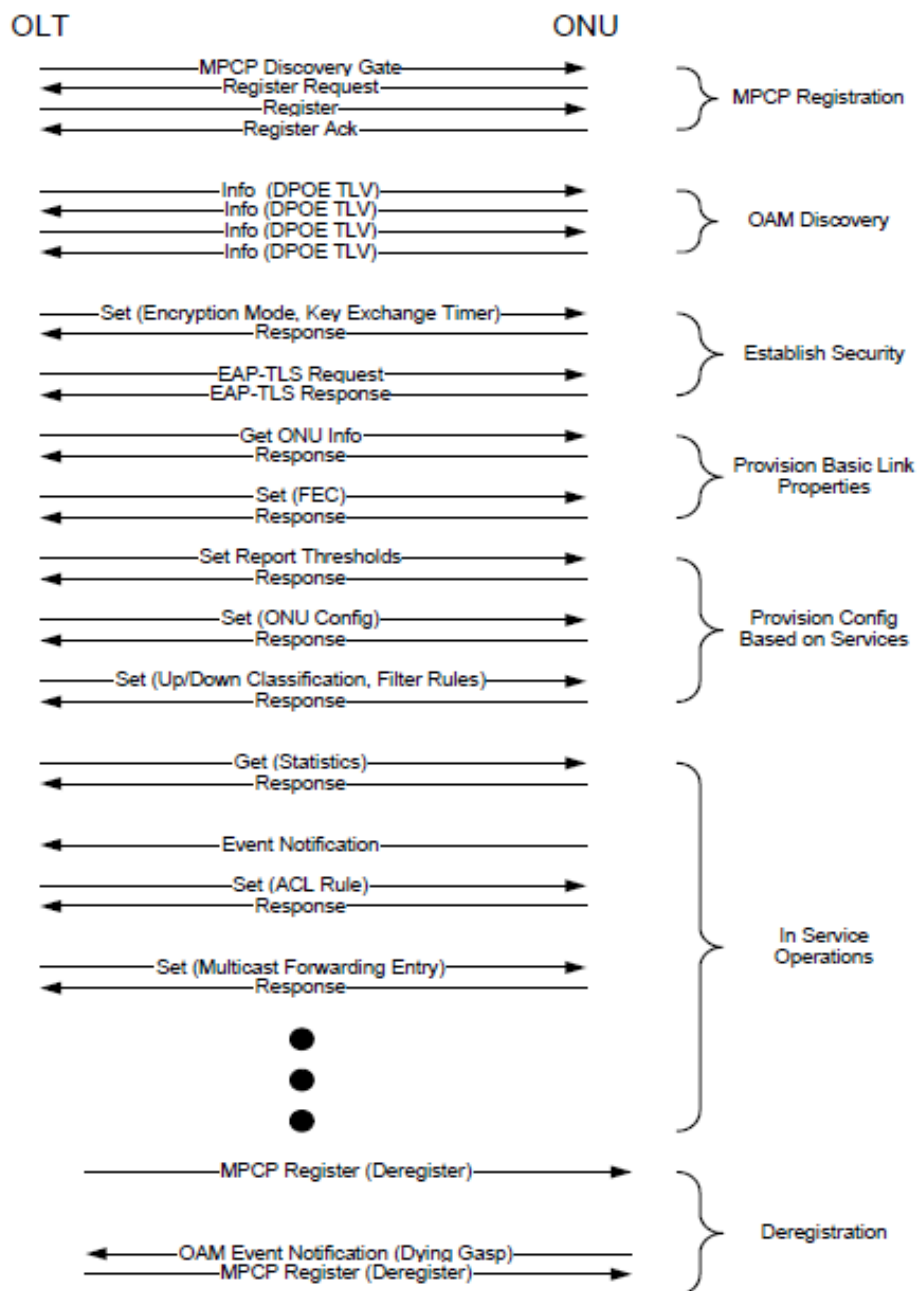
Figure 27 - Unicast Logical Link Life Cycle
