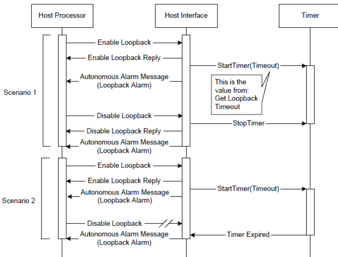
Figure 18 - Enable/Disable Loopback
