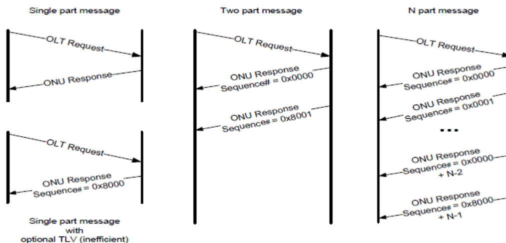
Figure 6 - Sample Message Exchange
