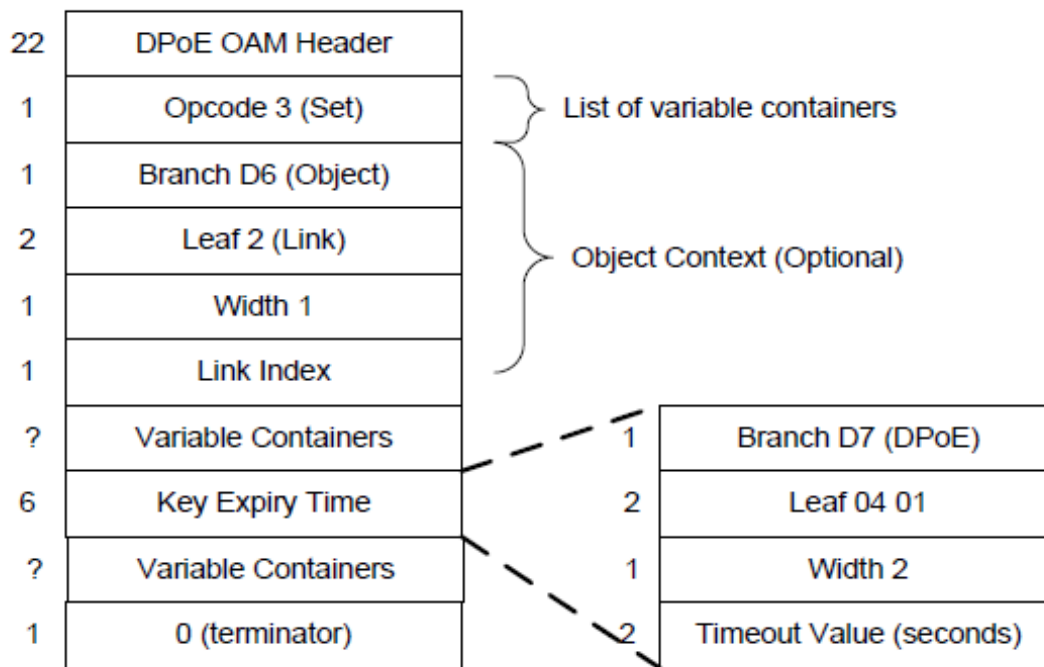
Figure 23 - Set Key Exchange Timer Request PDU
