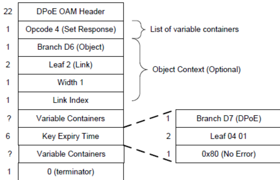
Figure 24 - Set Key Exchange Timer Response PDU
