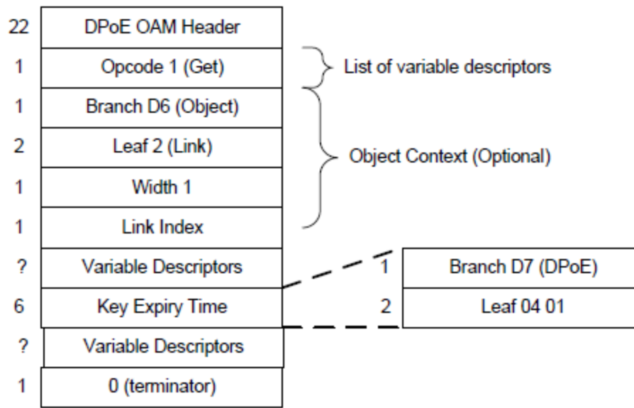
Figure 25 - Get Key Exchange Timer PDU
