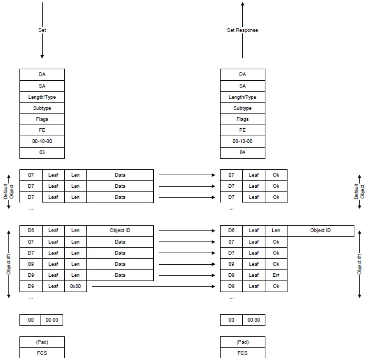
Figure 20 - Set and Set Response
