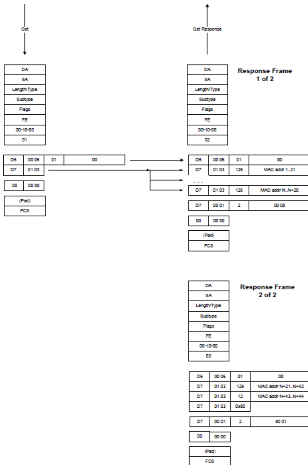
Figure 22 - Multi-Part Replies
