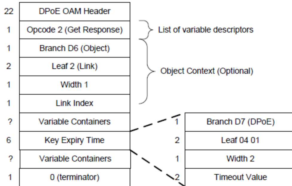
Figure 26 - Get Key Exchange Timer Response PDU
