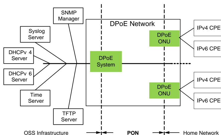
Figure 5 - DPoE OSS Overview
