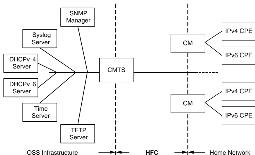
Figure 4 - DOCSIS OSS Overview
