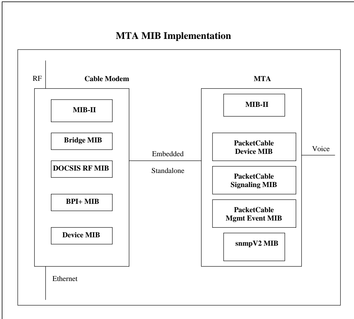
Figure 3. Embedded and Standalone MTA implementations
