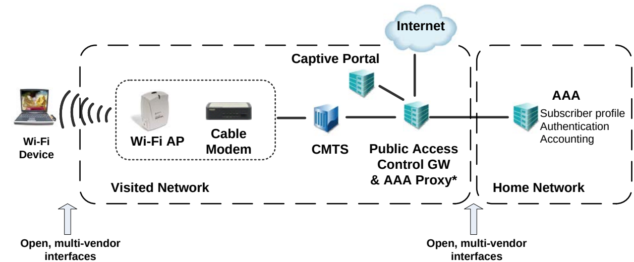
Figure 1 - Architecture View
