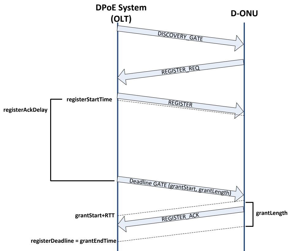
Figure 24 - Discovery Process with registerStartTime , registerAckDelay , and registerDeadline .
