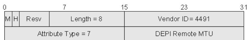
Figure 42 - DEPI Remote MTU Max Payload AVP
