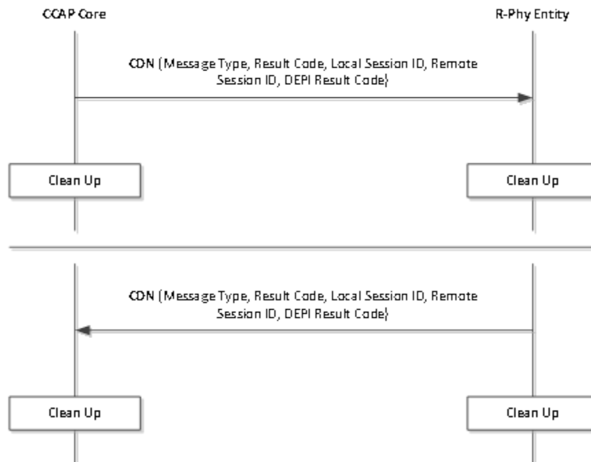
Figure 16 - R-PHY Session Teardown
