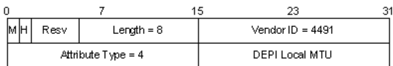
Figure 41 - DEPI Local MTU AVP
