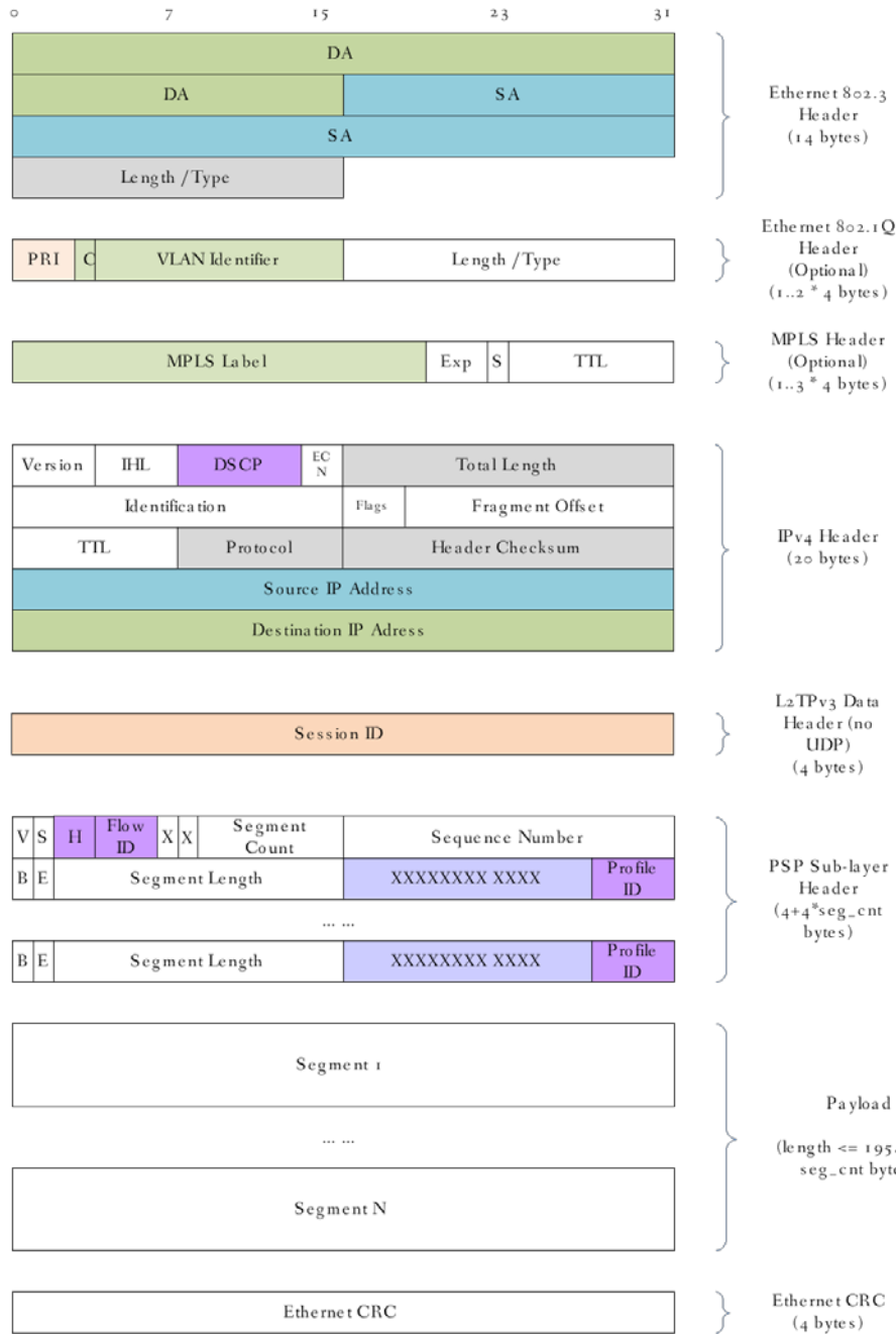
Figure 58 - Example of a Complete DEPI Packet Format (IPv4) with Extras
