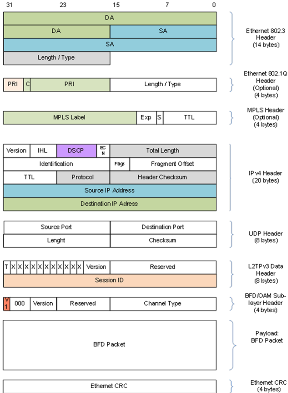
Figure 60 - BFD Sublayer (with UDP)
