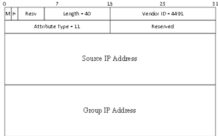
Figure 42 - DEPI Remote Multicast Join AVP
