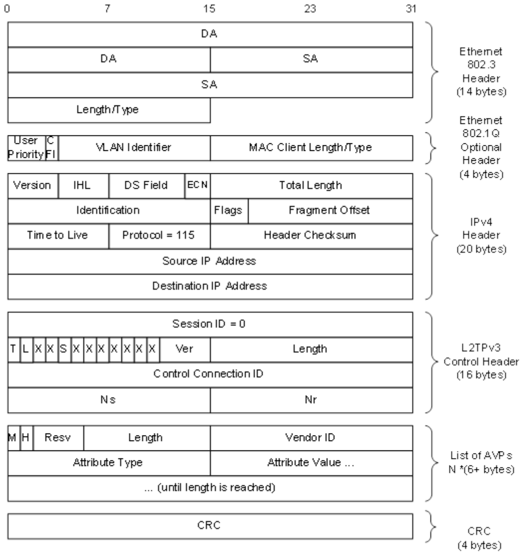
Figure 10 - L2TP Control Message without UDP Header
