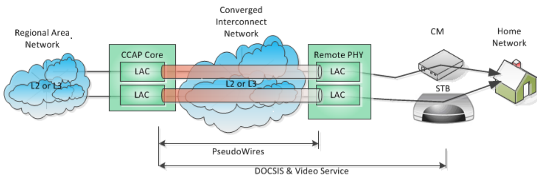
Figure 8 - Remote PHY Topology with Multiple Connections
