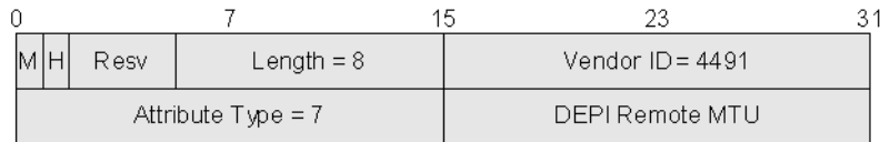
Figure 40 - DEPI Remote MTU Max Payload AVP
