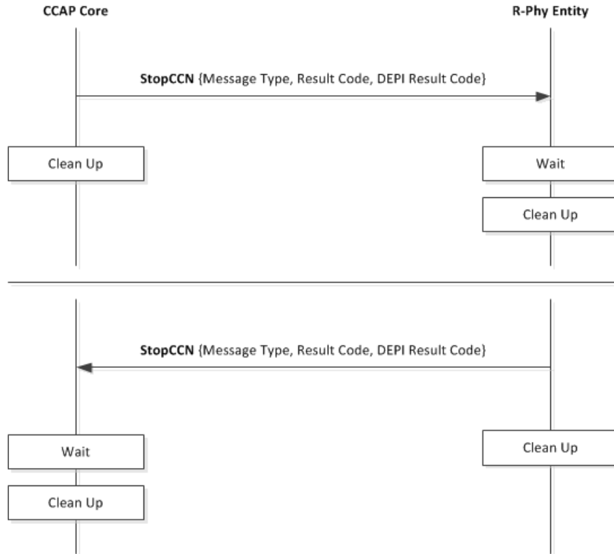
Figure 13 - R-PHY L2TP Control Connection Teardown
