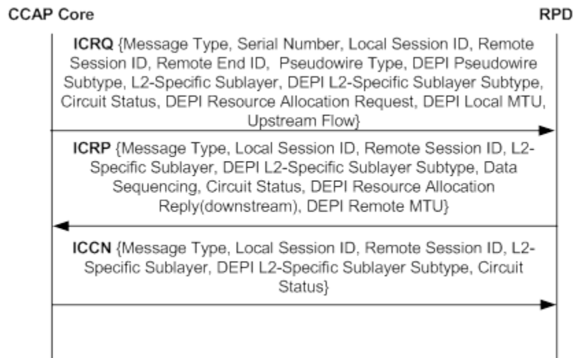
Figure 15 - R-PHY L2TP Session Setup
