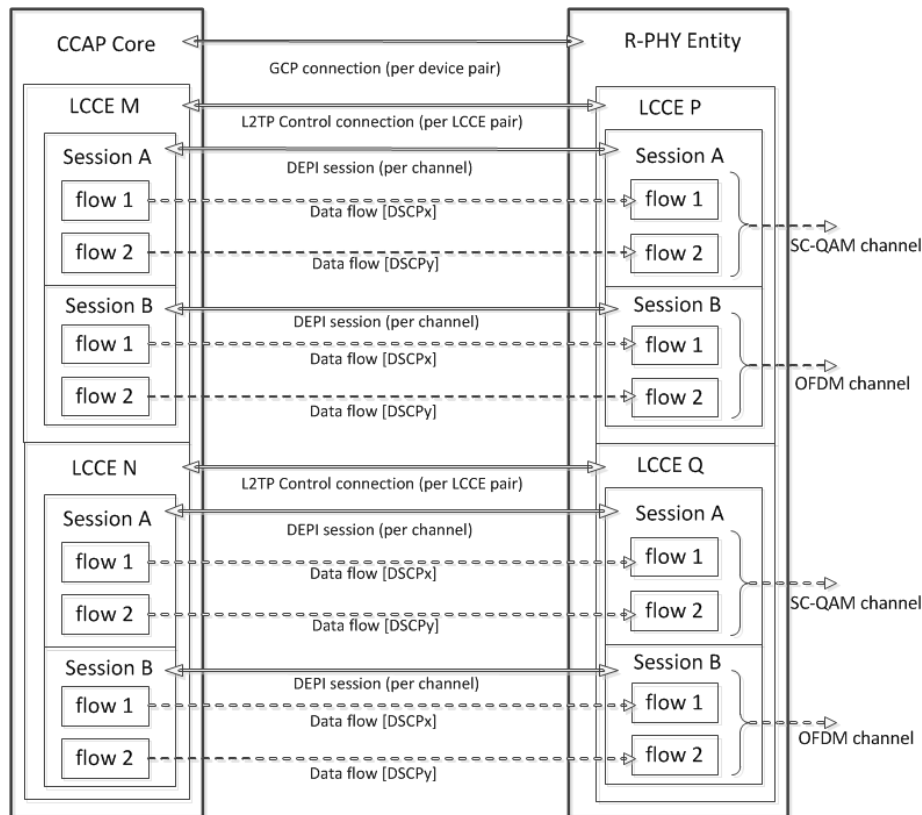
Figure 9 - R-PHY Connectivity Hierarchy
