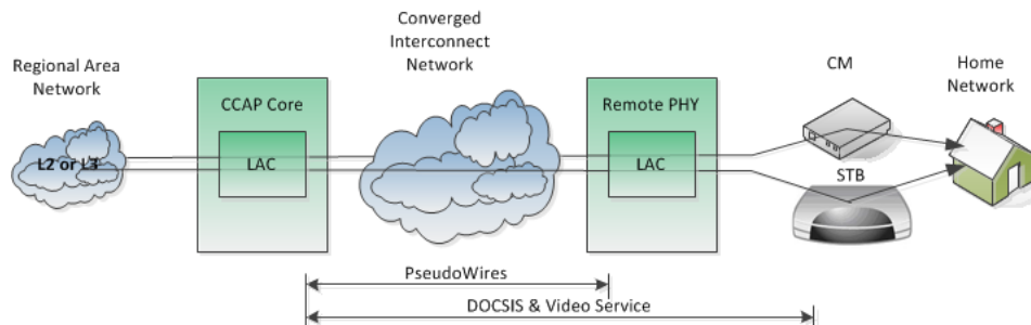
Figure 6 - End-to-end Remote PHY Topology
