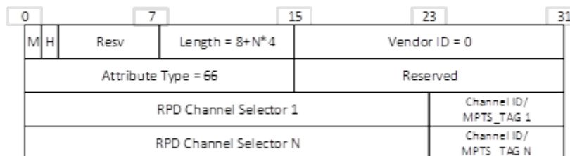
Figure 29 - Remote End ID AVP
