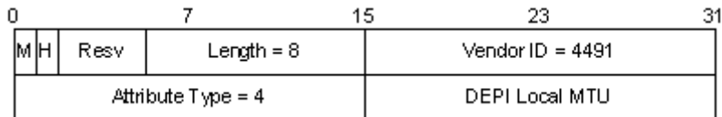
Figure 39 - DEPI Local MTU AVP
