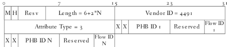
Figure 38 - DEPI Resource Allocation Reply AVP
