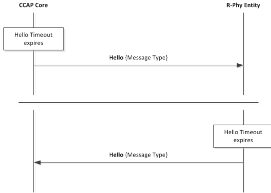
Figure 14 - R-PHY L2TP Keep-alive
