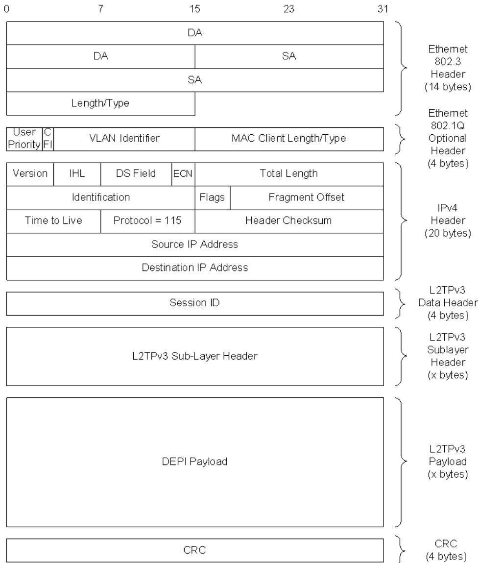
Figure 50 - L2TPv3 Data Packet Outer Encapsulation (without UDP)
