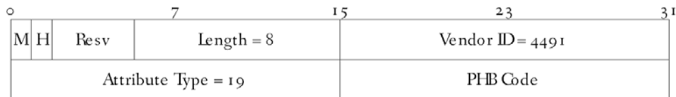
Figure 48 - DEPI S-BFD Return Path DSCP AVP
