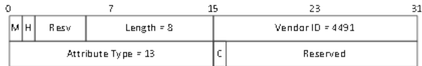
Figure 43 - DEPI Multicast Capability AVP
