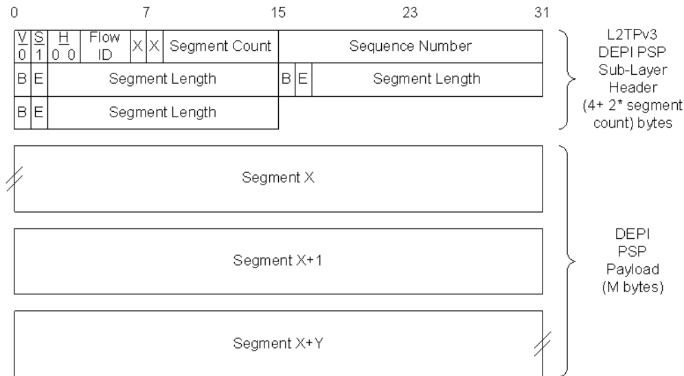
Figure 54 - DEPI Legacy PSP Sublayer Header and Payload
