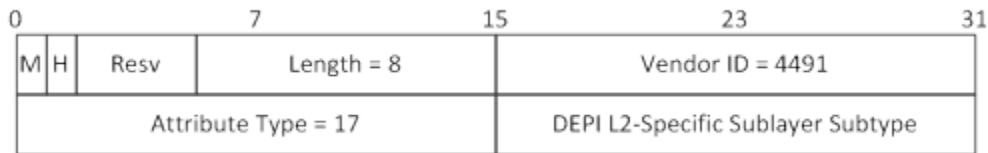
Figure 46 - DEPI L2-Specific Sublayer Subtype AVP
