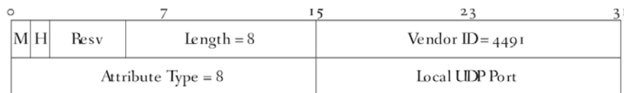
Figure 41 - DEPI Local UDP Port AVP
