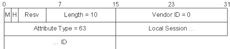
Figure 27 - Local Session ID AVP
