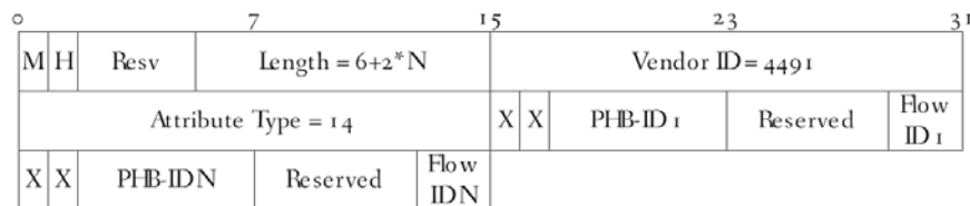
Figure 44 - Upstream Flow AVP
