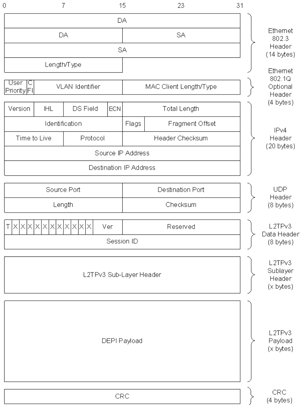
Figure 51 - L2TPv3 Data Packet Outer Encapsulation with UDP Header
