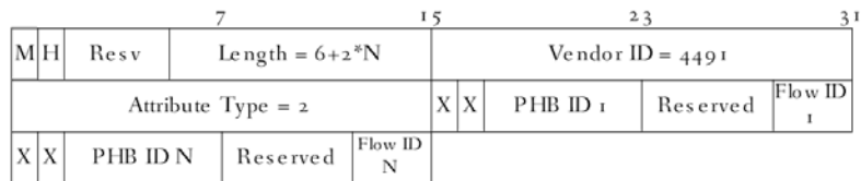
Figure 37 - DEPI Resource Allocation Request AVP
