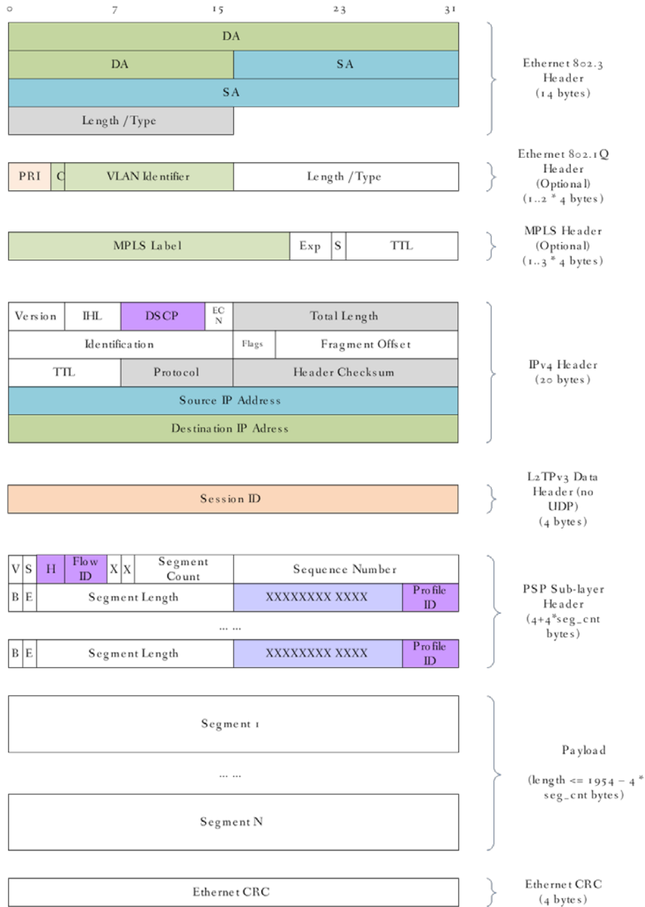
Figure 57 - Example of a Complete DEPI Packet Format (IPv4) with Extras
