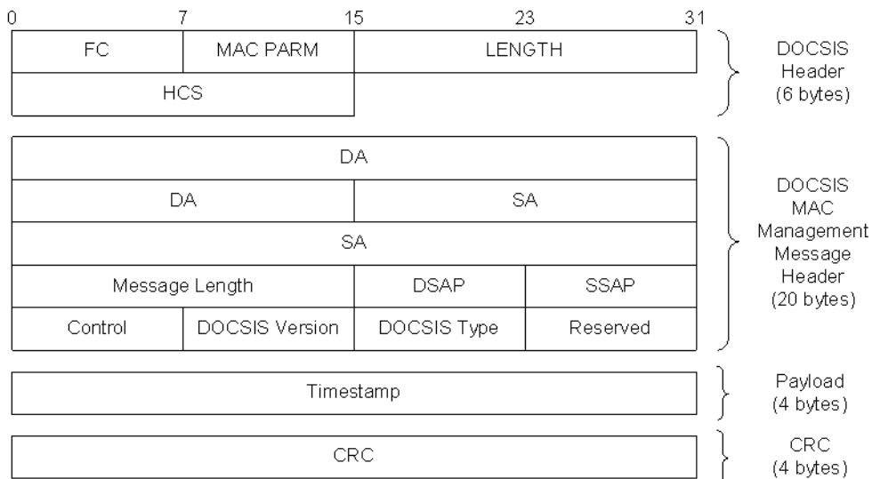
Figure 5 - Format of a DOCSIS SYNC MAC Message
