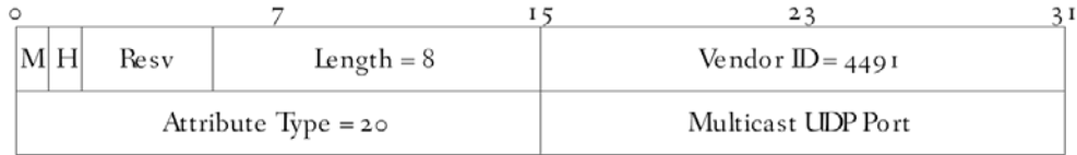
Figure 49 - DEPI Multicast UDP Port AVP
