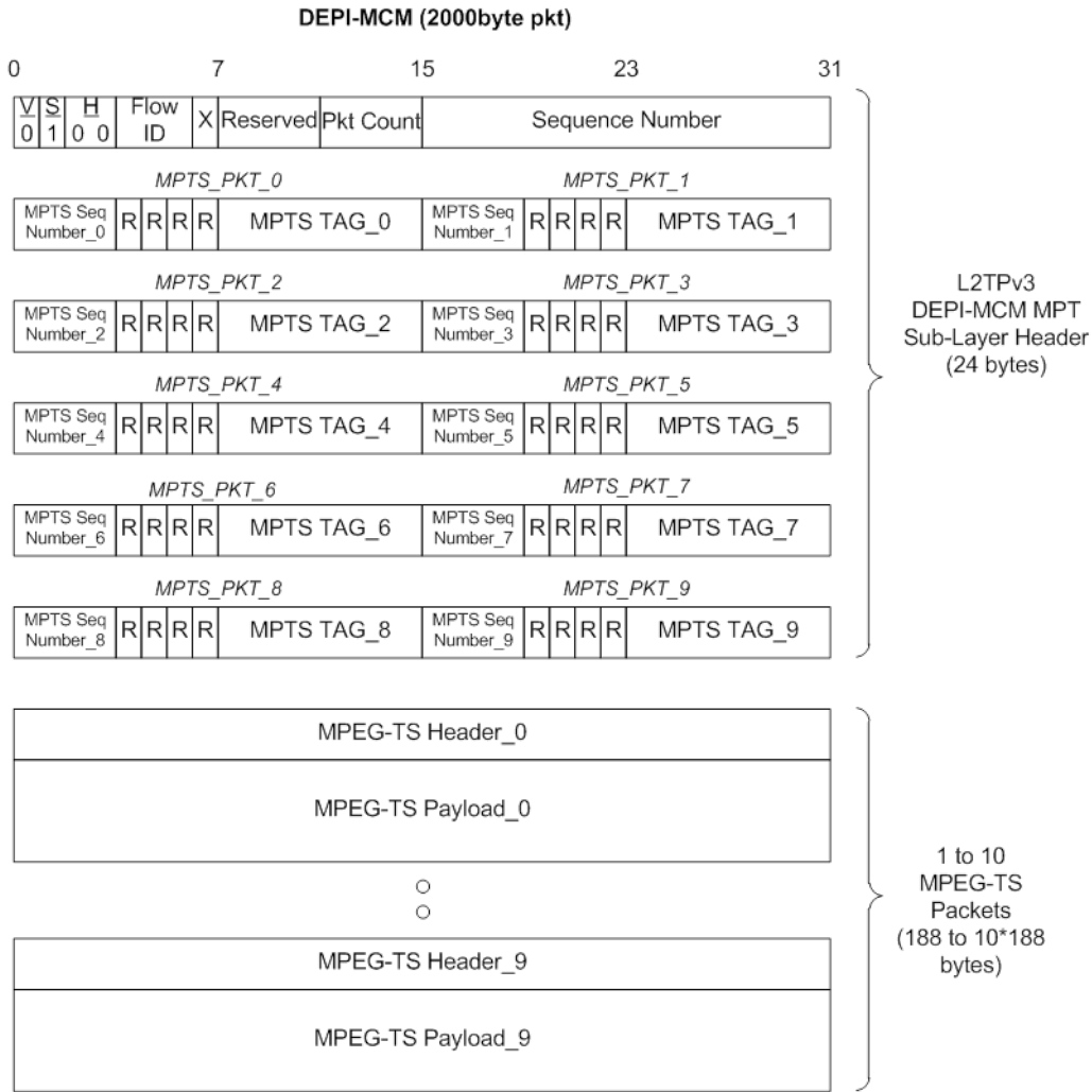
Figure 53 - MCM Sublayer Header and Payload
