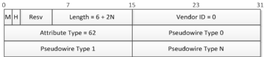
Figure 26 - Pseudowire Capabilities List AVP
