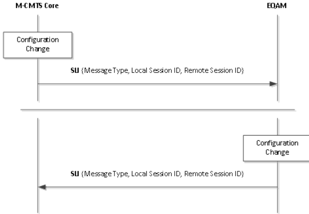
Figure 17 - R-PHY Session Updates
