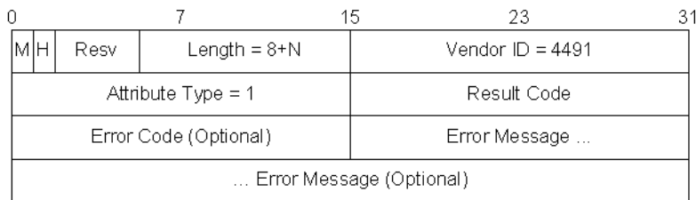
Figure 36 - DEPI Result and Error Code AVP
