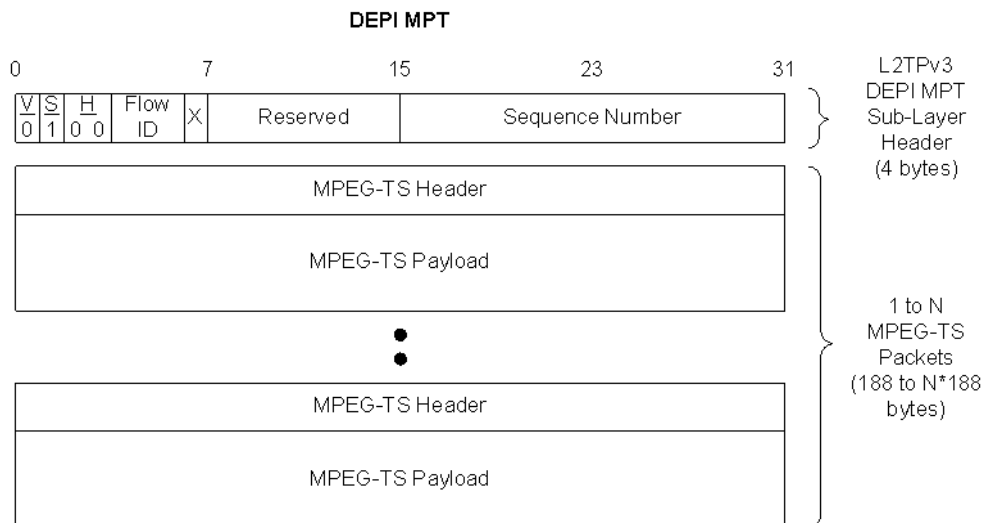
Figure 52 - DEPI MPT Sublayer Header and Payload
