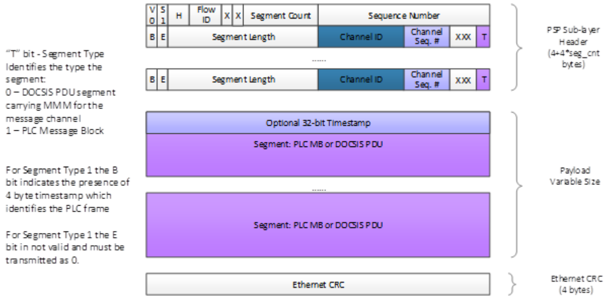
Figure 56 - Use of DEPI PSP Sublayer Header for PLC Sub-channel
