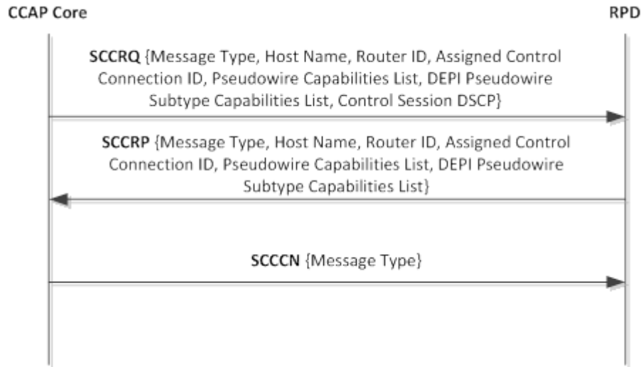
Figure 12 - R-PHY L2TP Control Connection Setup
