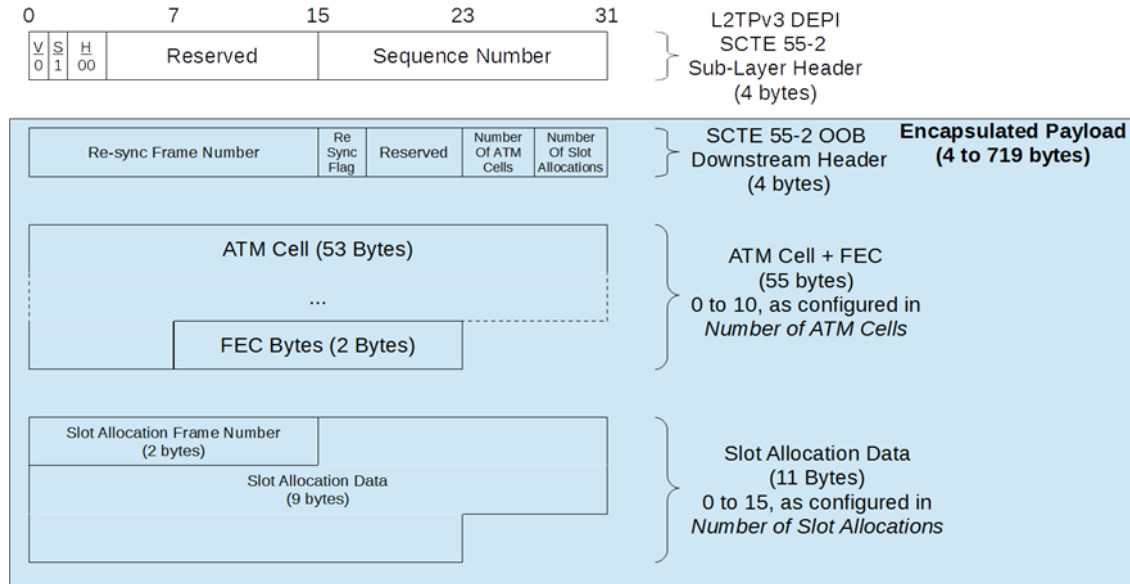
Figure 2 - SCTE 55-2 Downstream Packet Format
