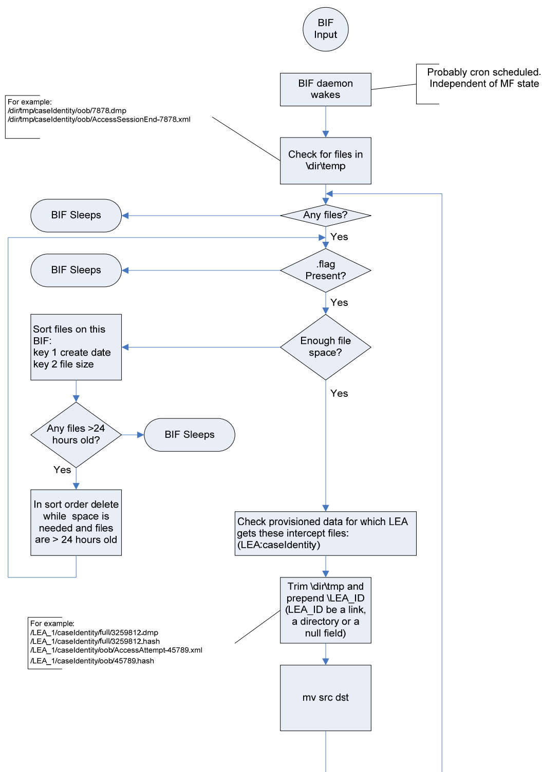
Figure 7 - The Broadband Intercept Function 31
