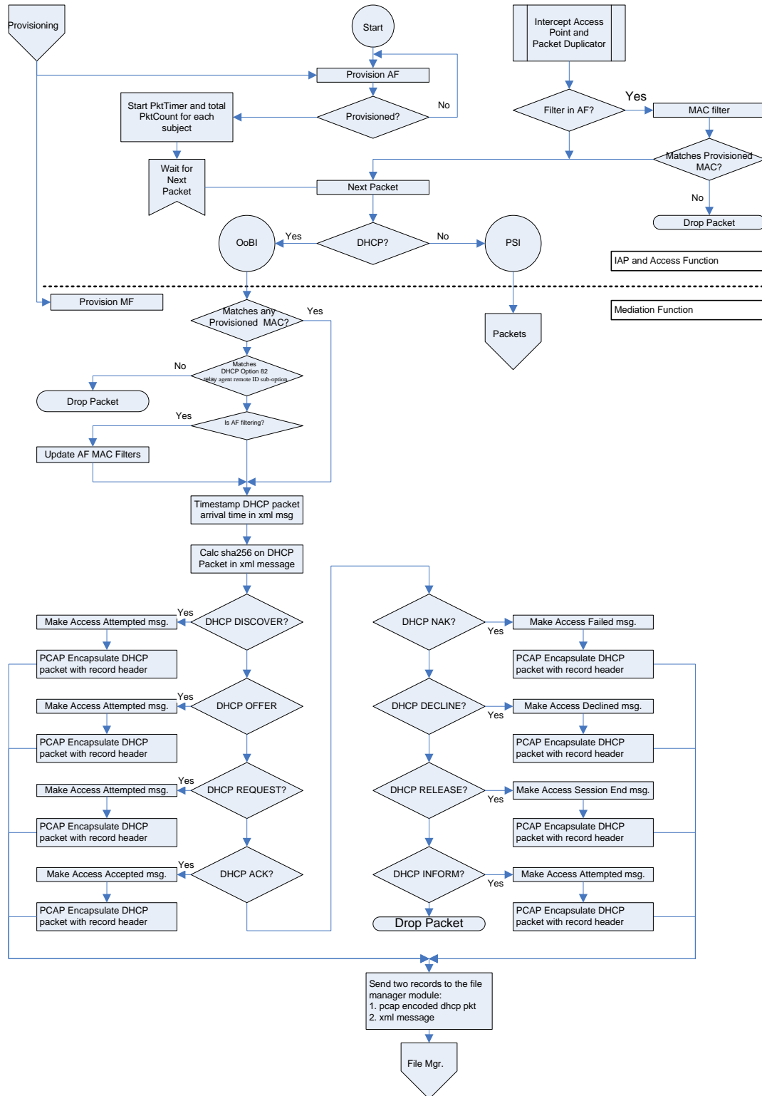
Figure 4 - The Access Function, Intercept Access Points, and Out-of-Band Processing 28
