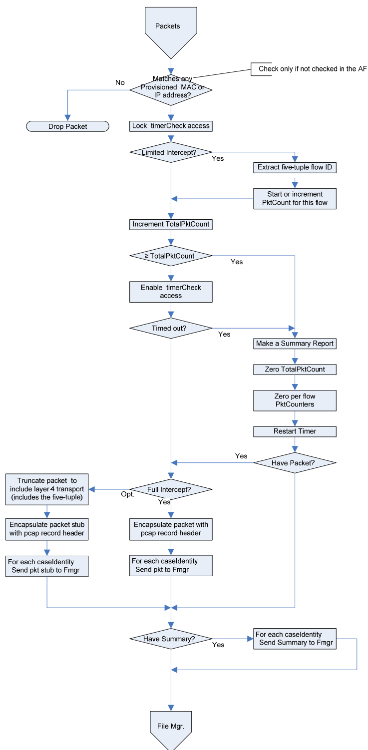
Figure 5 - Packet Processing: full intercepts and limited intercepts 29
