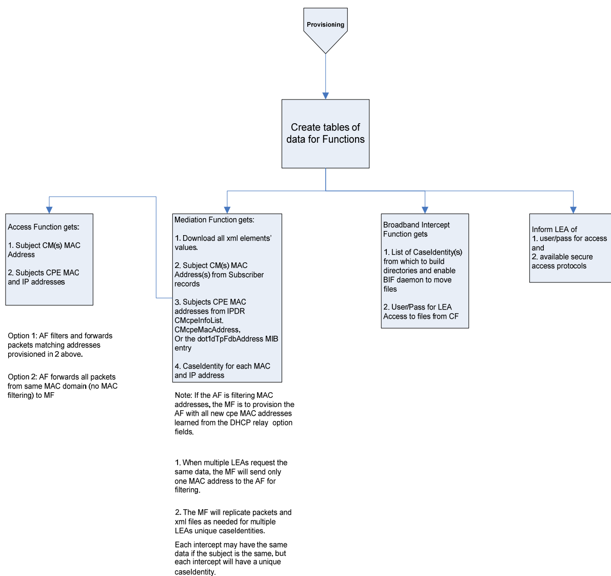
Figure 3 - Provisioning the functions with data from the CMTS 27
