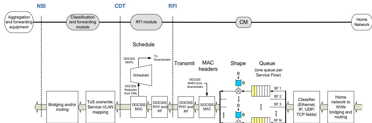
Figure 7-3 - Processing upstream data packets in the distributed CMTS architecture
