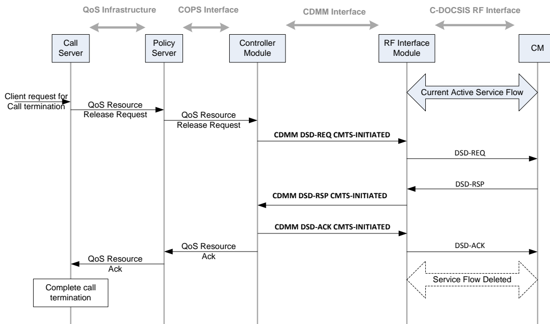
Figure I-4 - Headend-Initiated DSD for Session Termination
