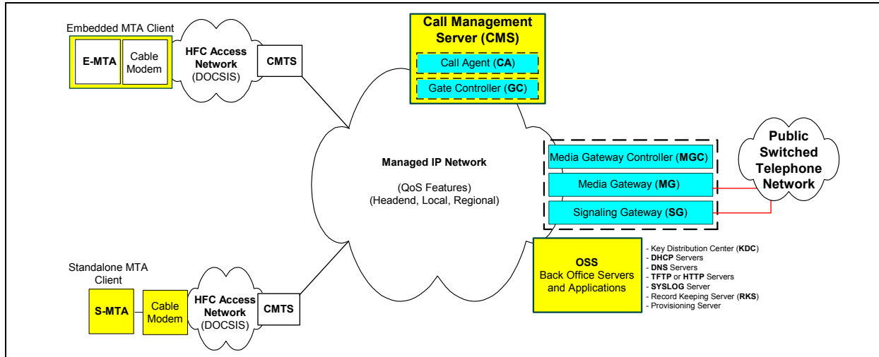
Figure 1. PacketCable Network Component Reference Mode
