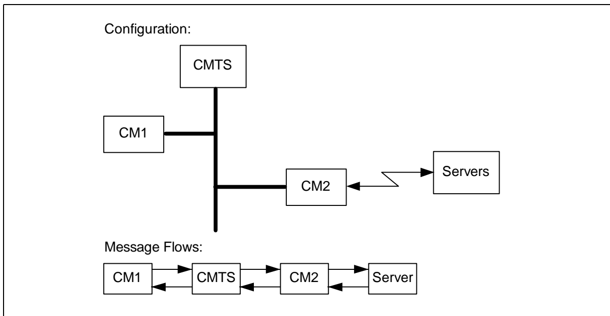
Figure 1-3. Server Location Not At CMTS
