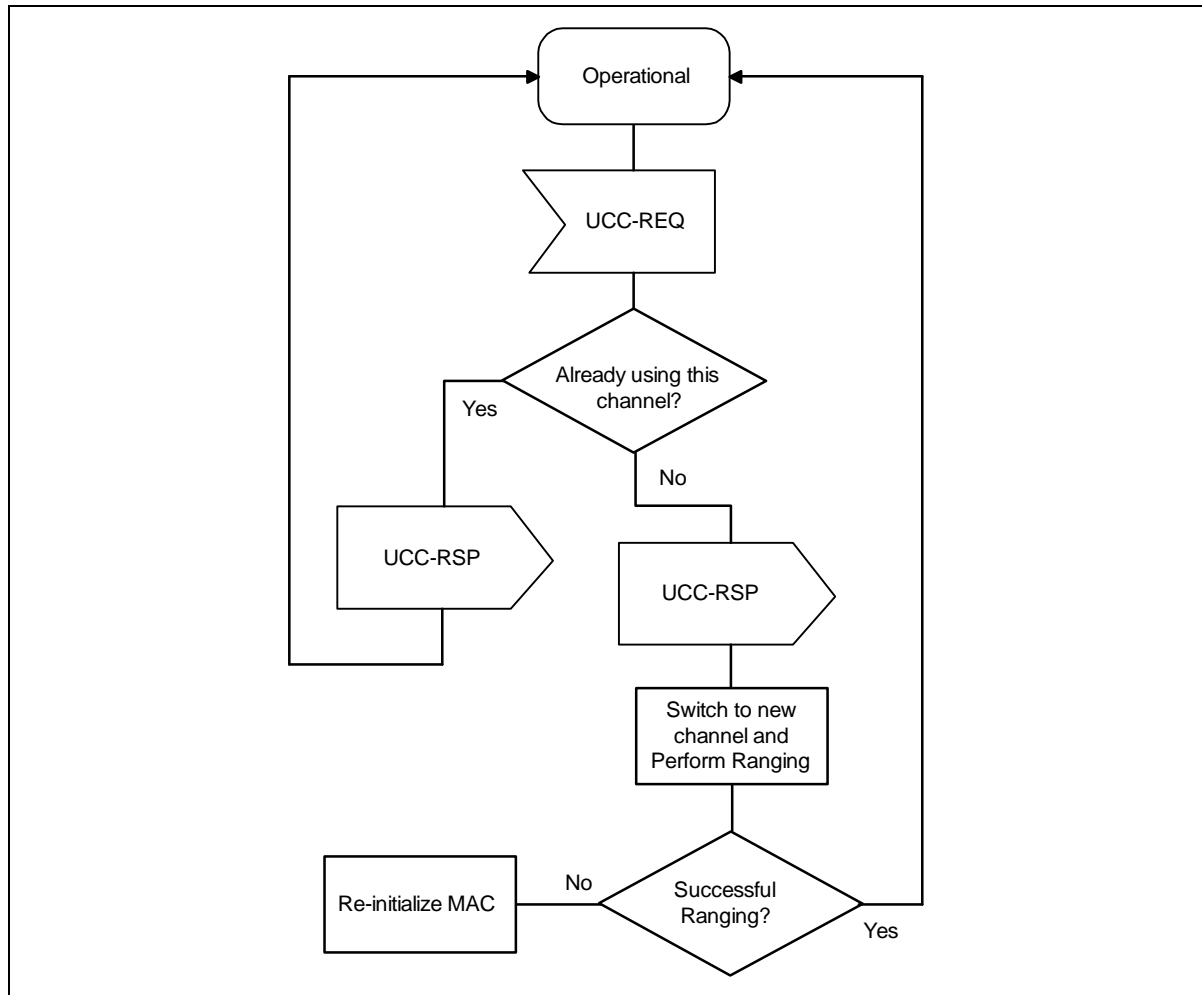
Figure 7-16. Changing Upstream Channels: CM View
