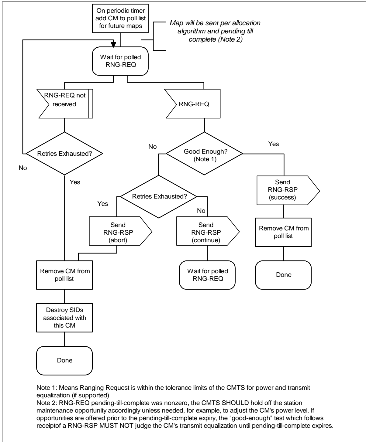
Figure 7-13. Periodic Ranging - CMTS
