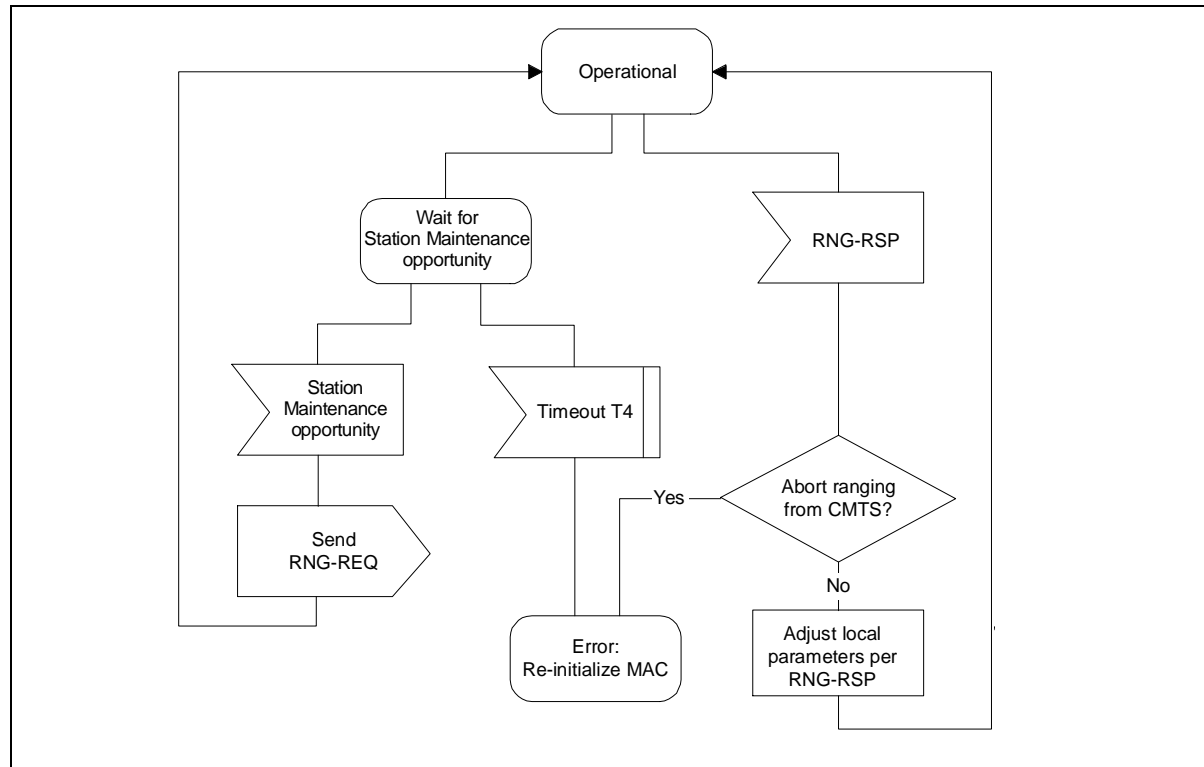
Figure 7-14. Periodic Ranging - CM View
