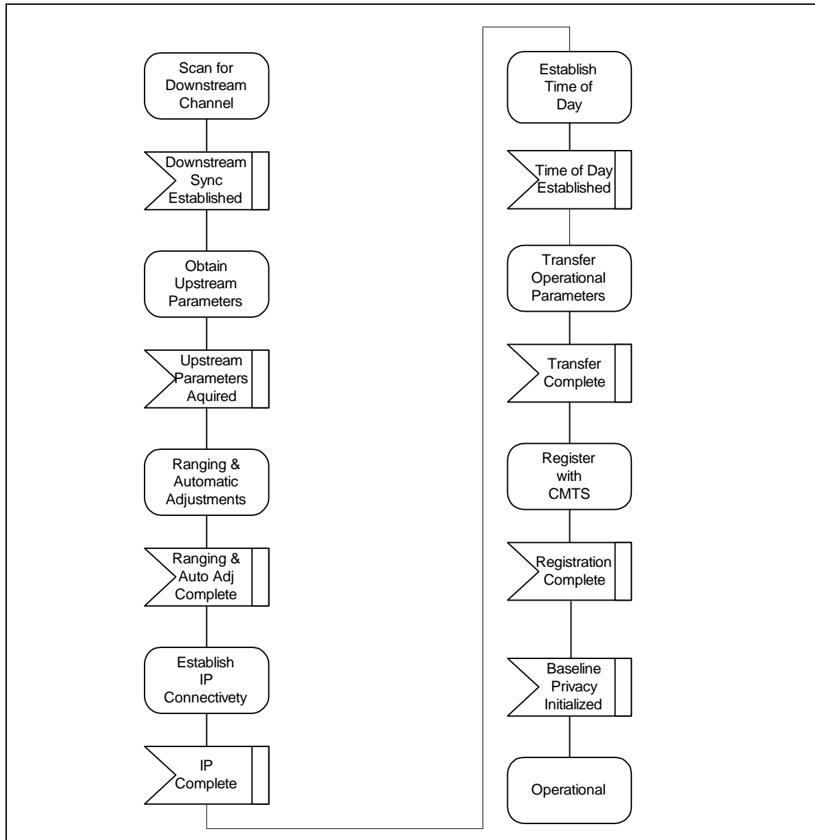
Figure 7-1. CM Initialization Overview
