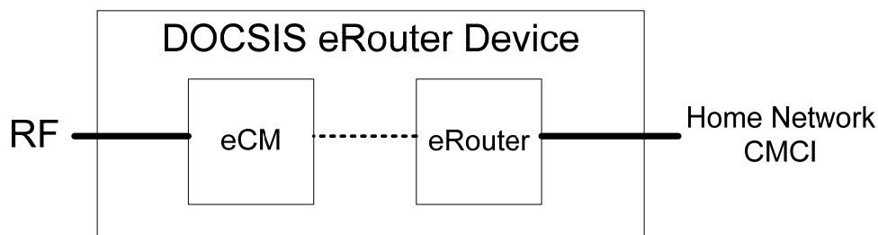
Figure 5–15 - DOCSIS eRouter eDOCSIS Device Reference Model 28
