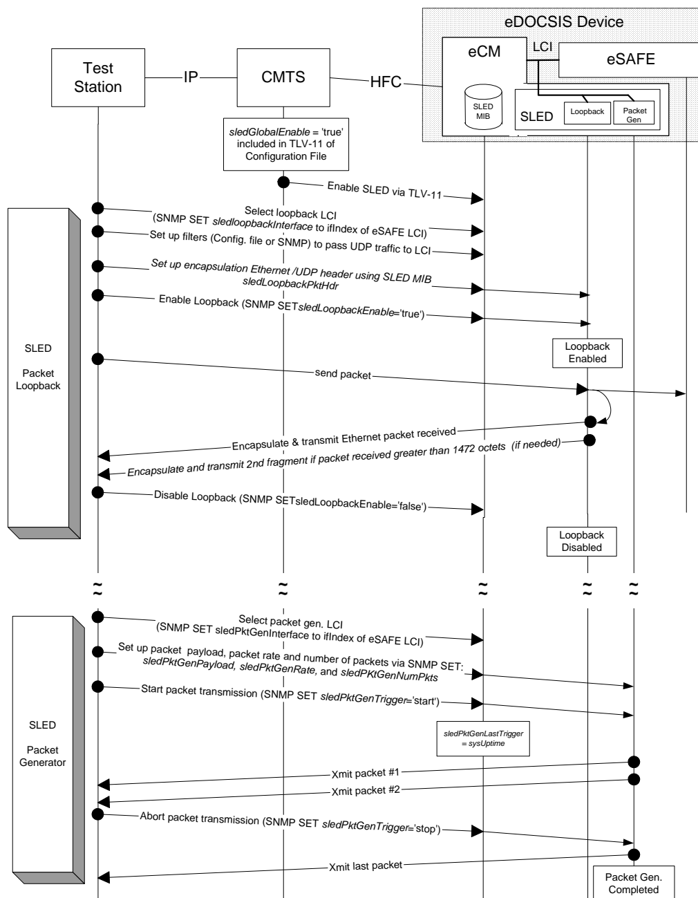
Figure 5-24 - SLED Packet Loopback And Generation Sequences
