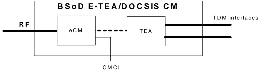
Figure 5–13 - BSoD eTEA (with DOCSIS CM) eDOCSIS Reference Model 26
