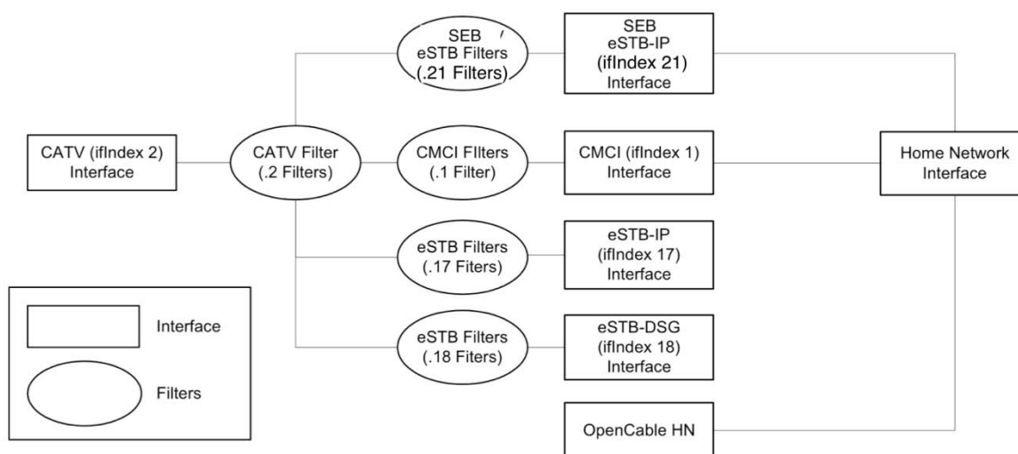
Figure 5-21 – eSTB Interface 41
