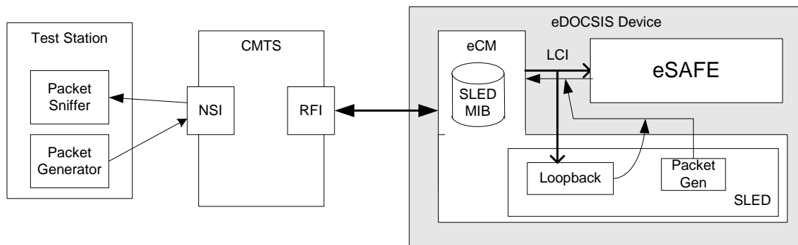
Figure 5–22 - SLED Reference Model
