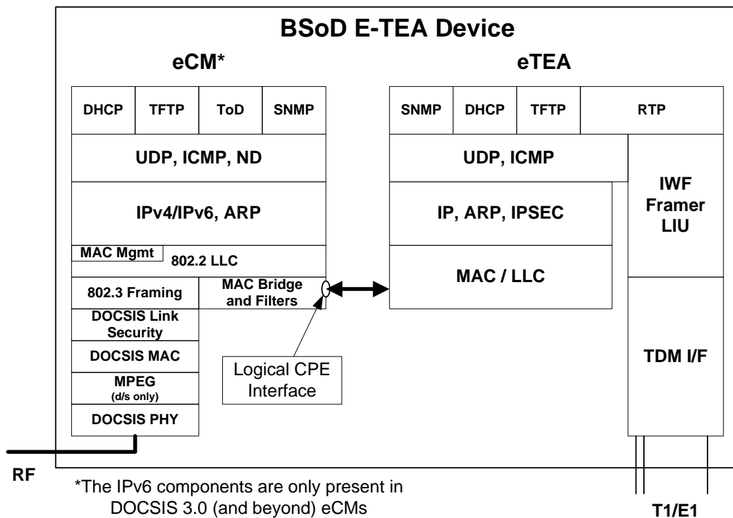
Figure 5–14 - eCM - eTEA Protocol Stacks 27
