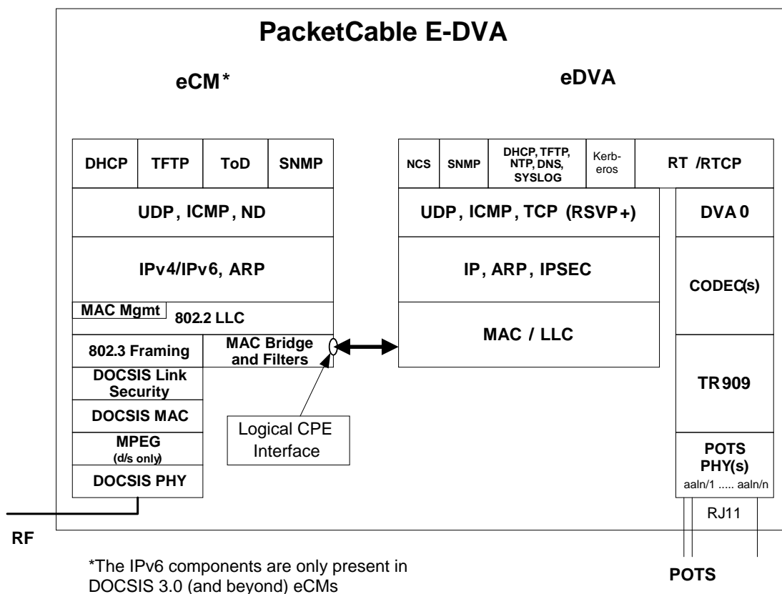
Figure 5–18 - eCM - eDVA Protocol Stacks 30
