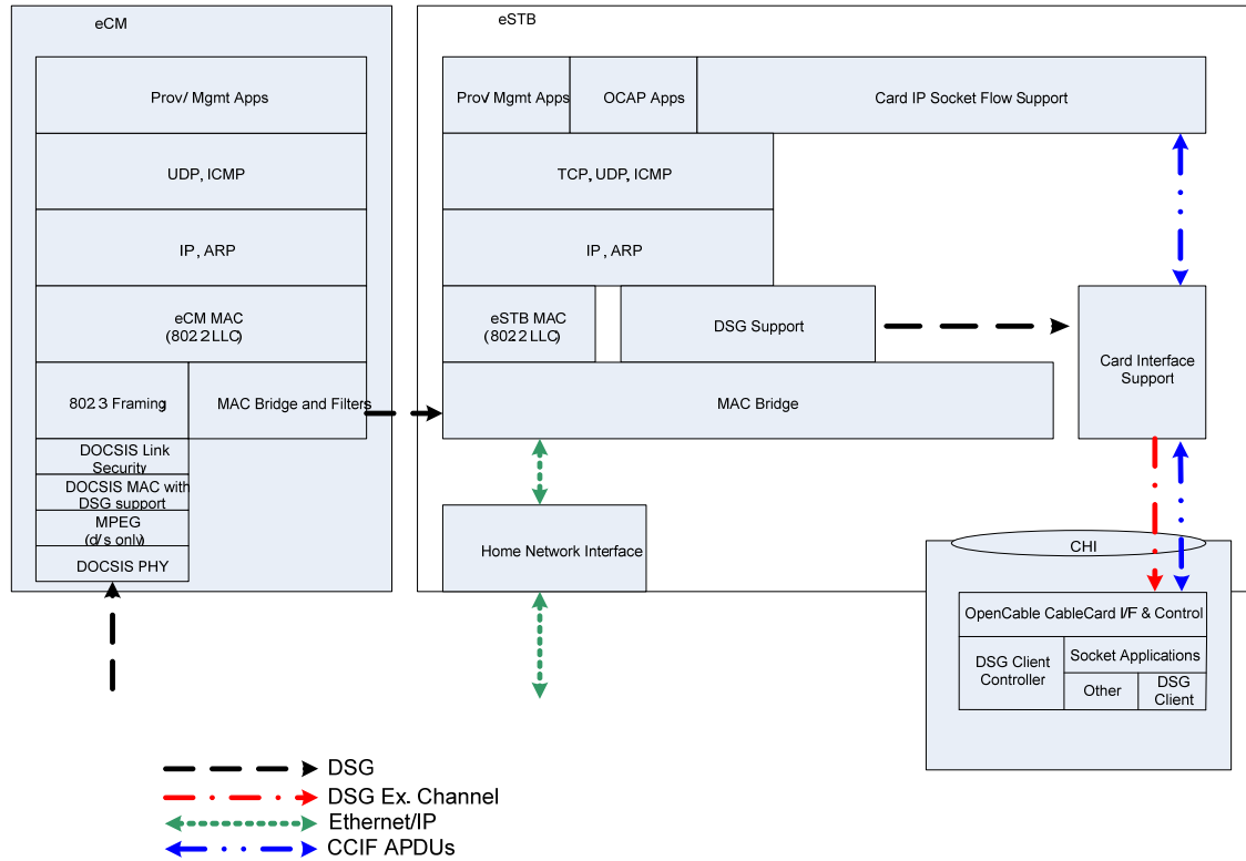
Figure 5-11 - Set-top Extender Bridge Client - Protocol Stack
