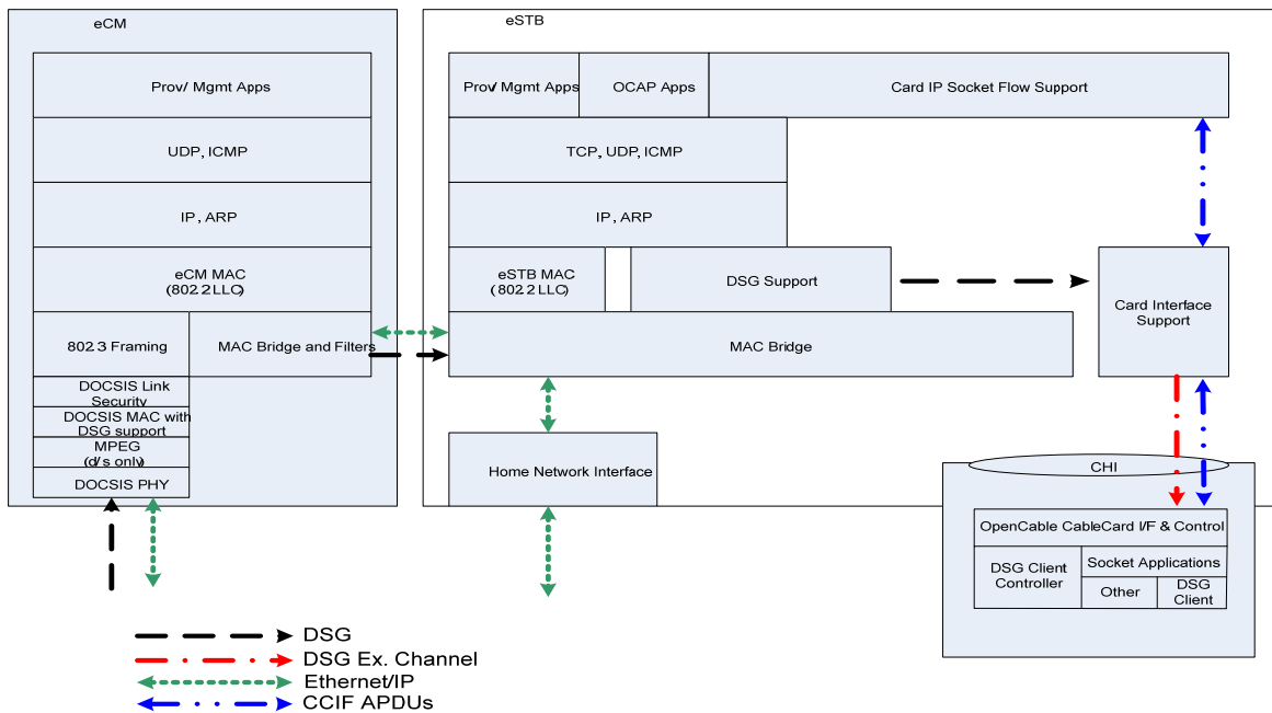
Figure 5-12 - Set-top Extender Bridge Server - Protocol Stack
