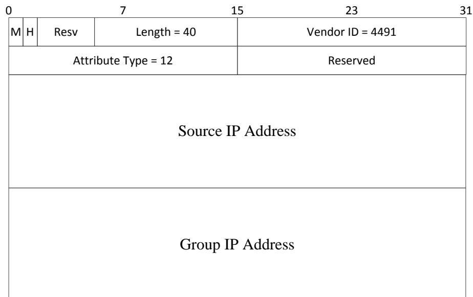
Figure 7-39 - DEPI Remote Multicast Leave AVP
