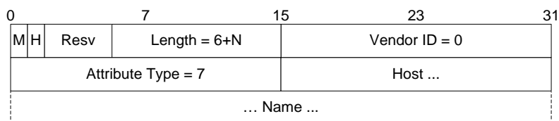
Figure 7–18 - Host Name AVP
