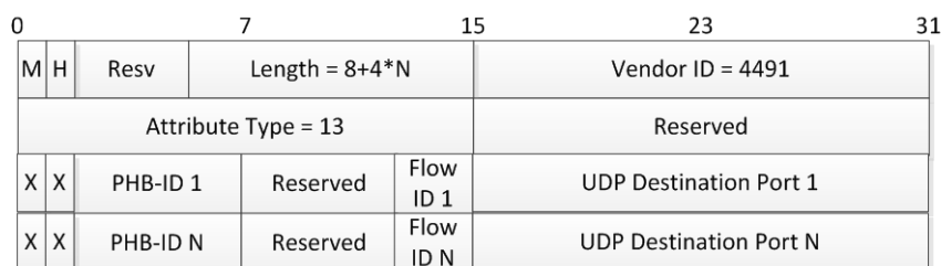
Figure 7-41 - Upstream Flow AVP
