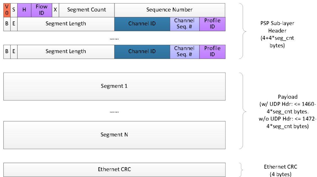
Figure 8-6 - DEPI PSP Sublayer Header and Payload
