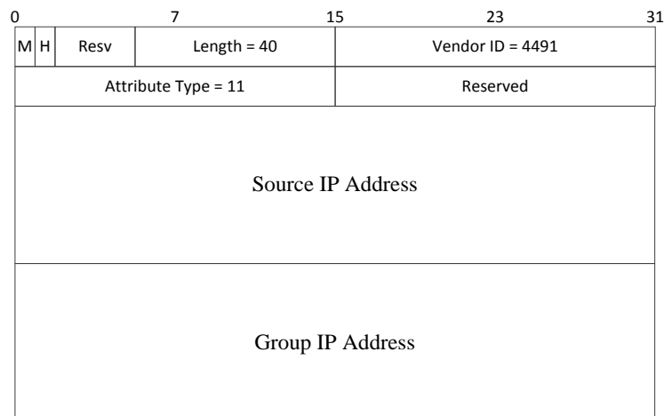
Figure 7–38 - DEPI Remote Multicast Join AVP
