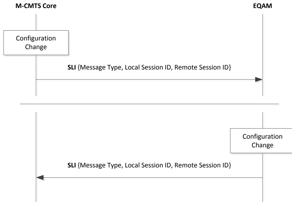
Figure 7–15 - R-PHY Session Updates
