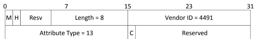
Figure 7-40 - DEPI Multicast Capability AVP
