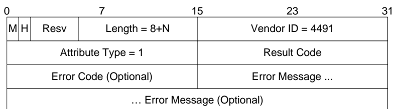
Figure 7–33 - DEPI Result and Error Code AVP
