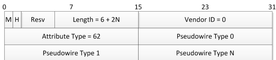
Figure 7–24 - Pseudowire Capabilities List AVP
