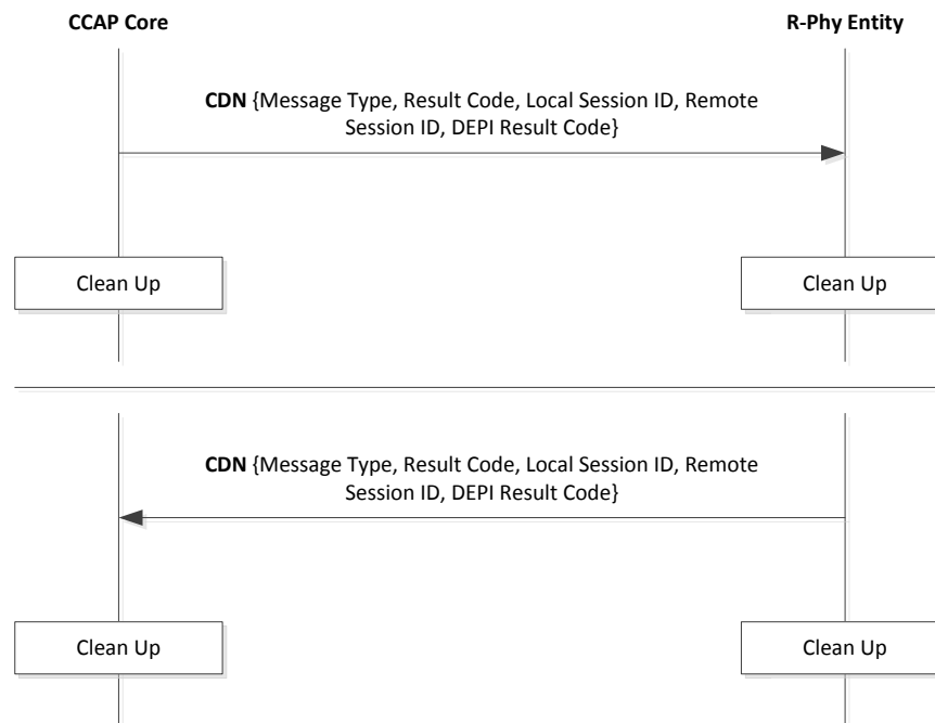
Figure 7–14 - R-PHY Session Teardown
