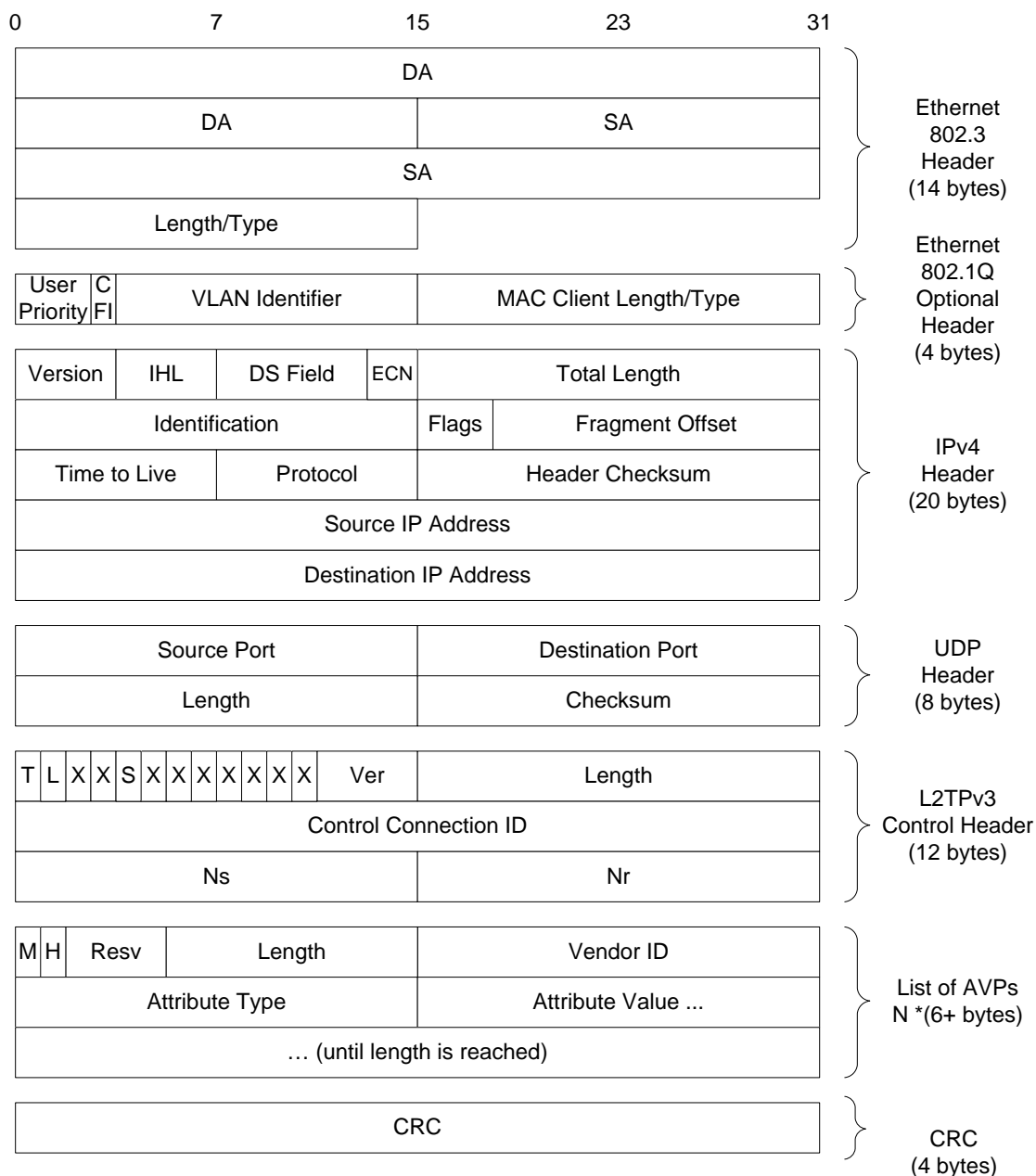
Figure 7–9 - L2TPv3 Control Packet with UDP Header
