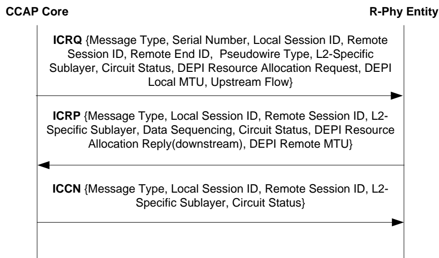
Figure 7–13 - R-PHY L2TP Session Setup
