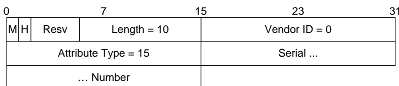
Figure 7–20 - Serial Number AVP
