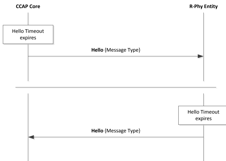
Figure 7–12 - R-PHY L2TP Keep-alive
