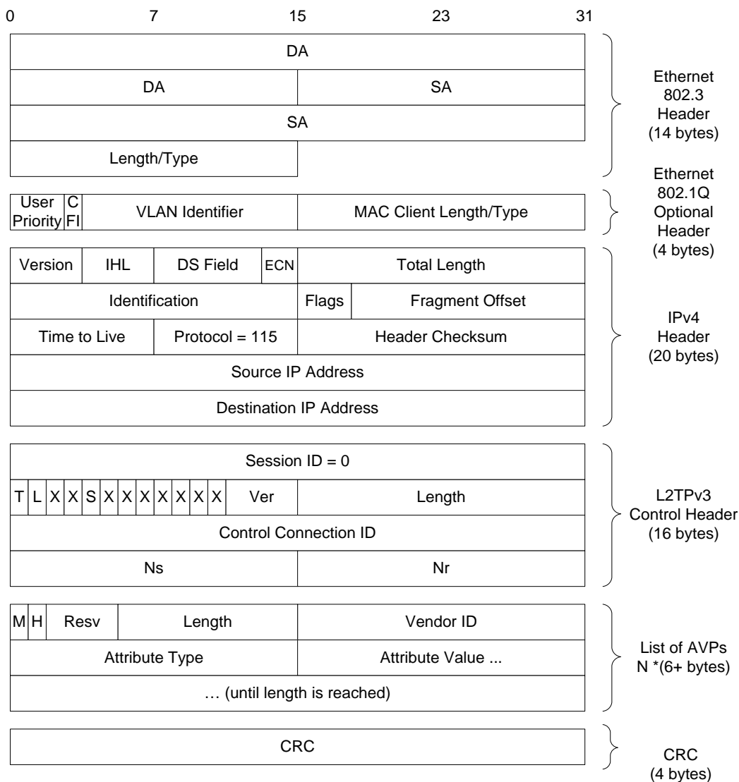
Figure 7–8 - L2TP Control Message without UDP Header
