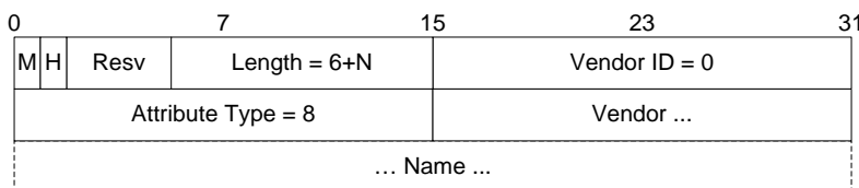
Figure 7–19 - Vendor Name AVP
