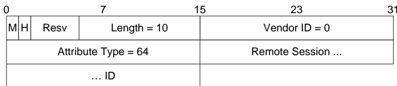
Figure 7–26 - Remote Session ID AVP
