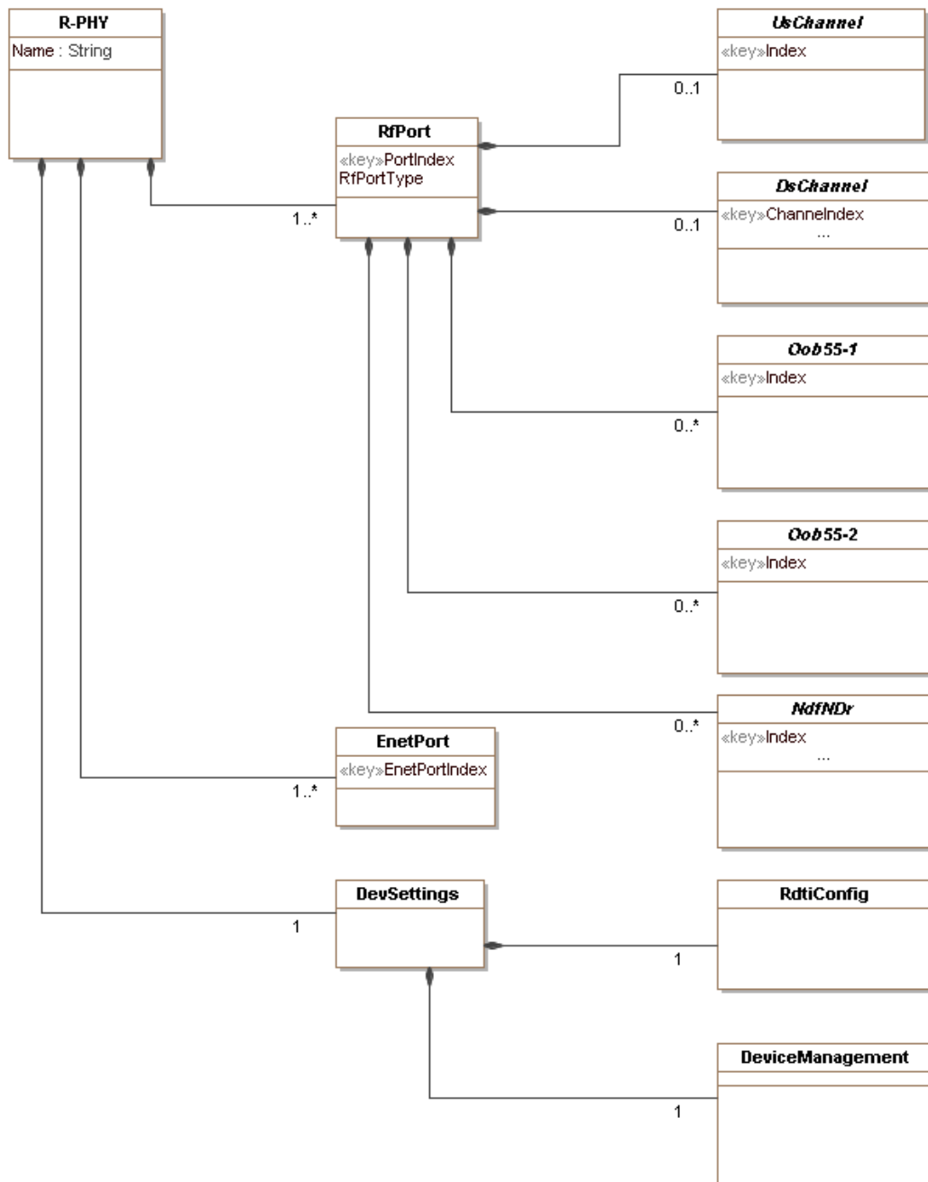
Figure 7-5 - Top-level Divisions of the RPD Model
