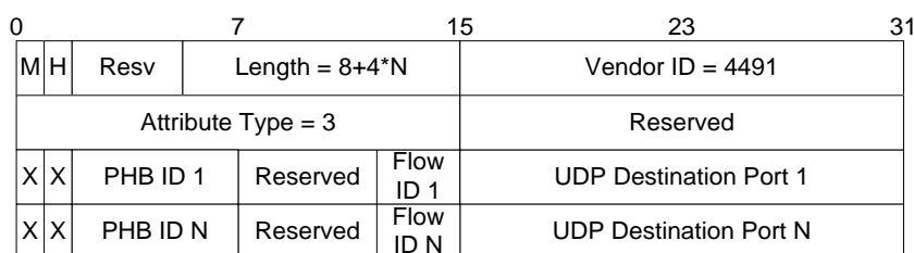
Figure 7-35 - DEPI Resource Allocation Reply AVP
