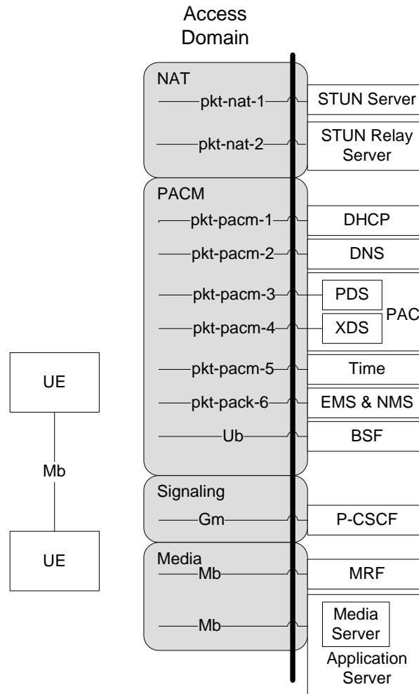
Figure 11 - Access Domain Reference Points
