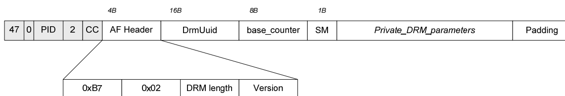
Figure I-3 - TAG Packet
