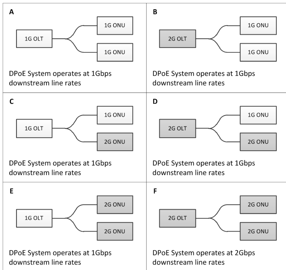
Figure 4: 2G-EPON system backward compatibility with 1G-EPON system
