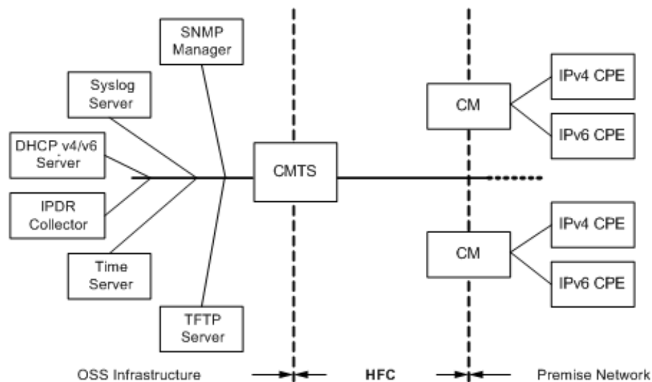
Figure 3 - DOCSIS OSS Overview
