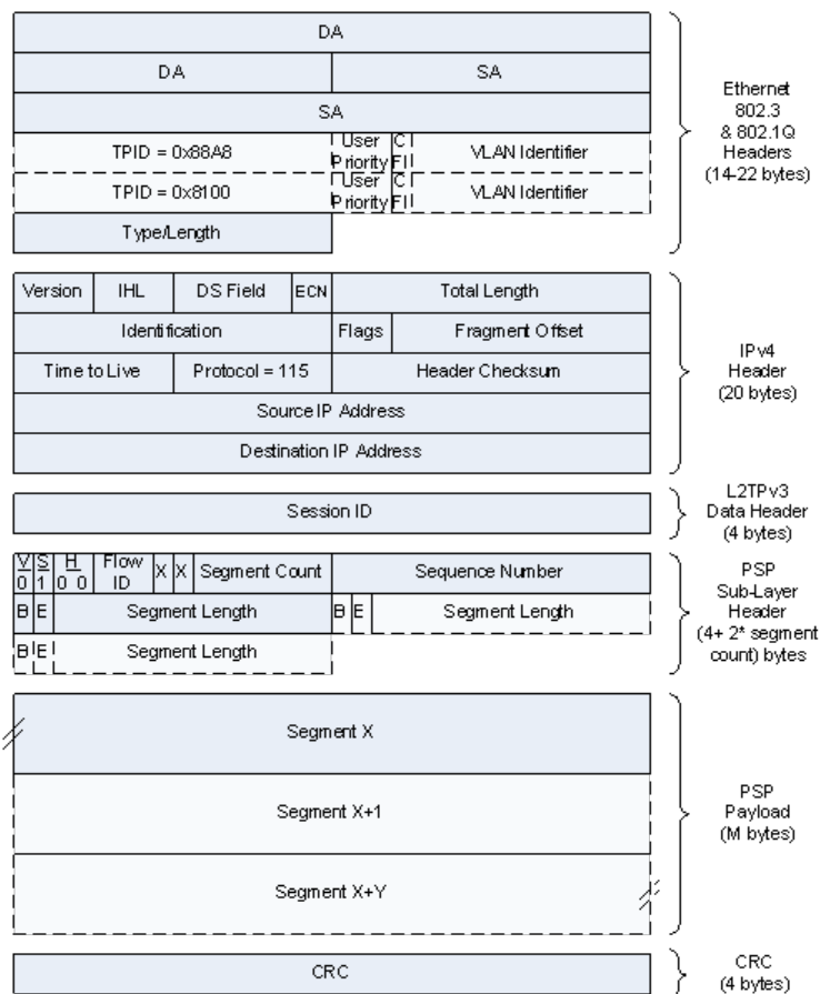
Figure 4 - UEPI IPv4 Packet with L2TPv3 Encapsulation
