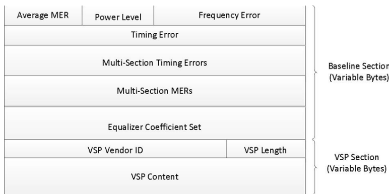
Figure 22 - UEPI Probe Payload Segment Format
