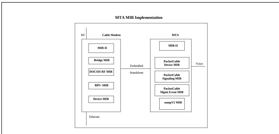
Figure 3. Embedded and Standalone MTA implementations
