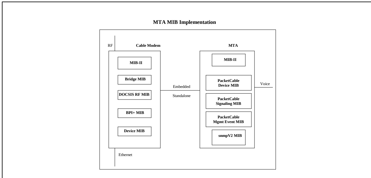
Figure 3 describes the possible MIB module implementation for an MTA (Embedded or Standalone):
