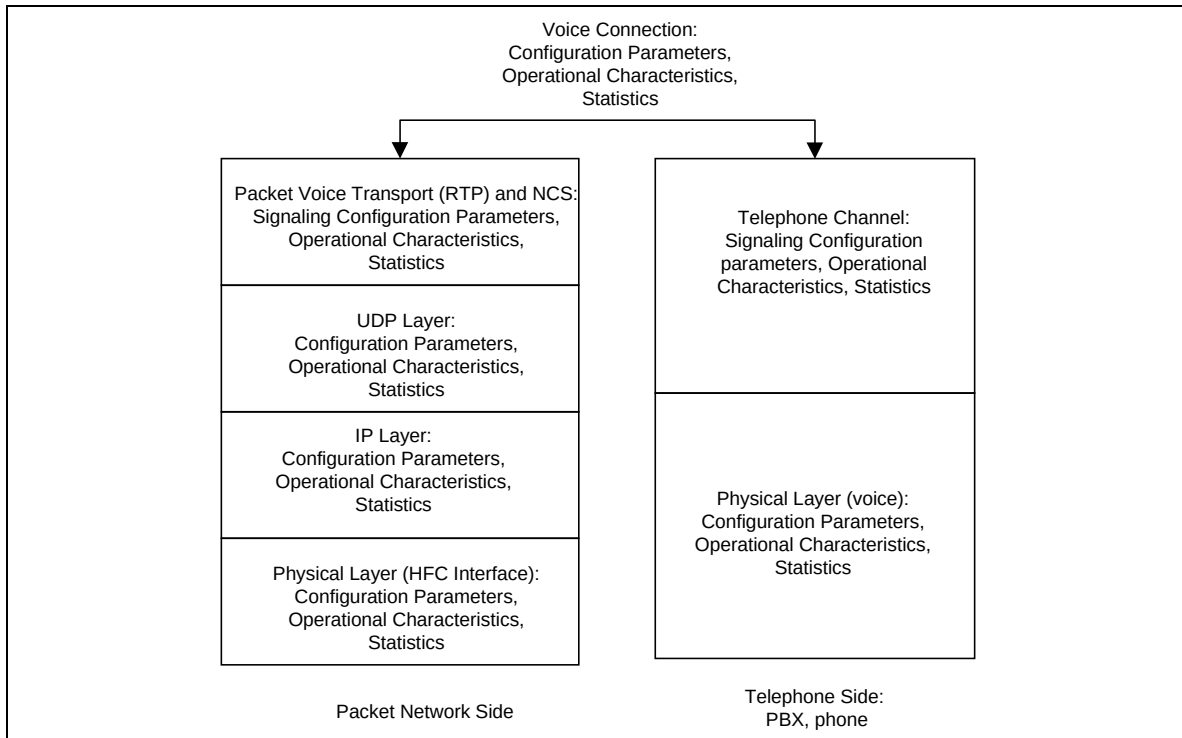
Figure 5. MIB Layering Model
