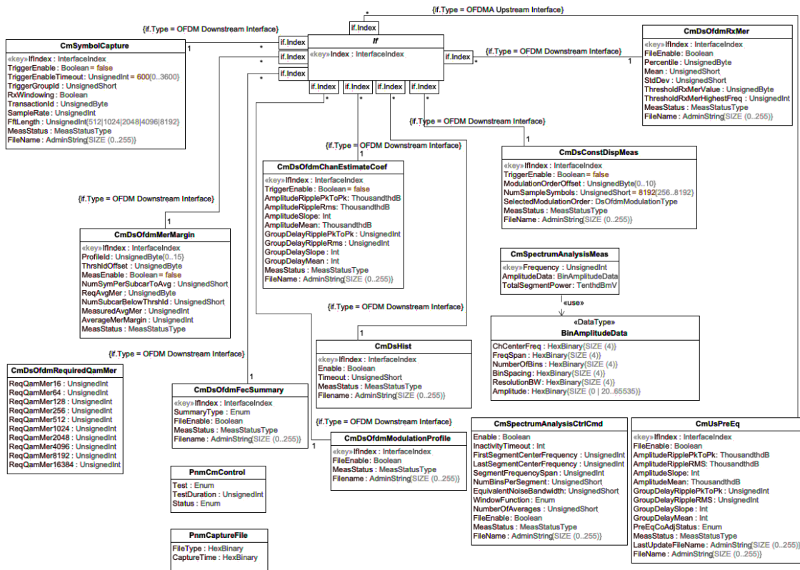
Figure 8 - Proactive Network Maintenance Information Model
