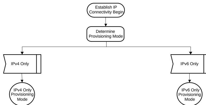
Figure 14 - Establish IP Connectivity
