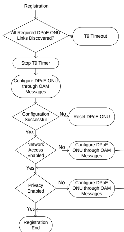
Figure 20 - Registration of D-ONU in DPoE System
