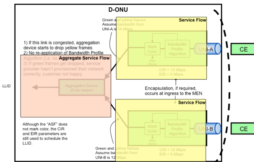
Figure 28 - Behavior of ASF-SF within D-ONU
