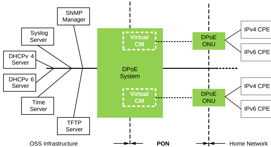
Figure 6 - vCM within the DPoE network
