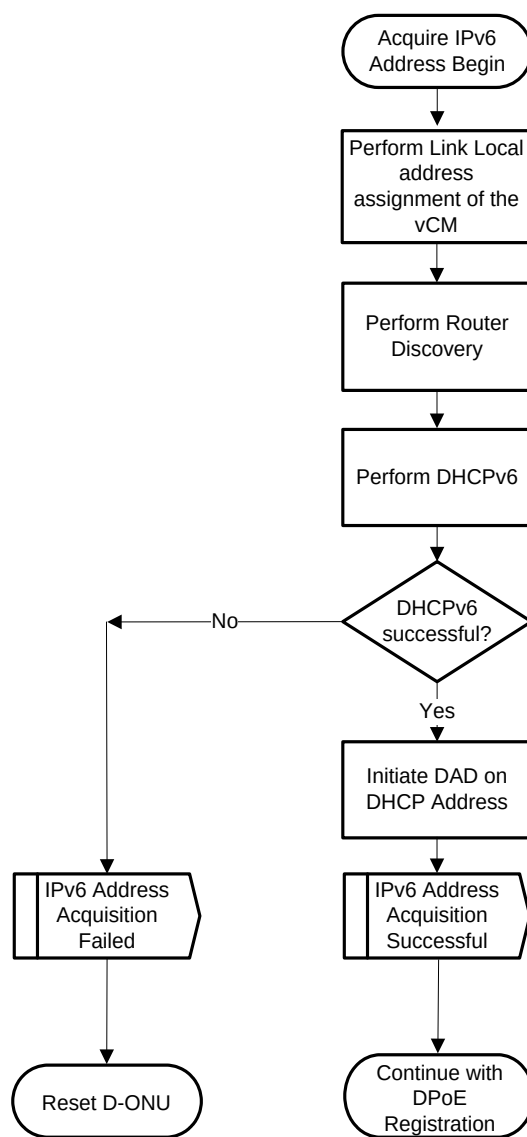
Figure 17 - IPv6 Address Acquisition
