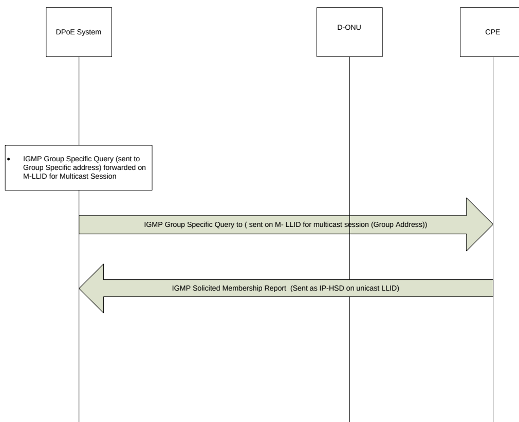
Figure 32 - Multicast Group Specific Messages
