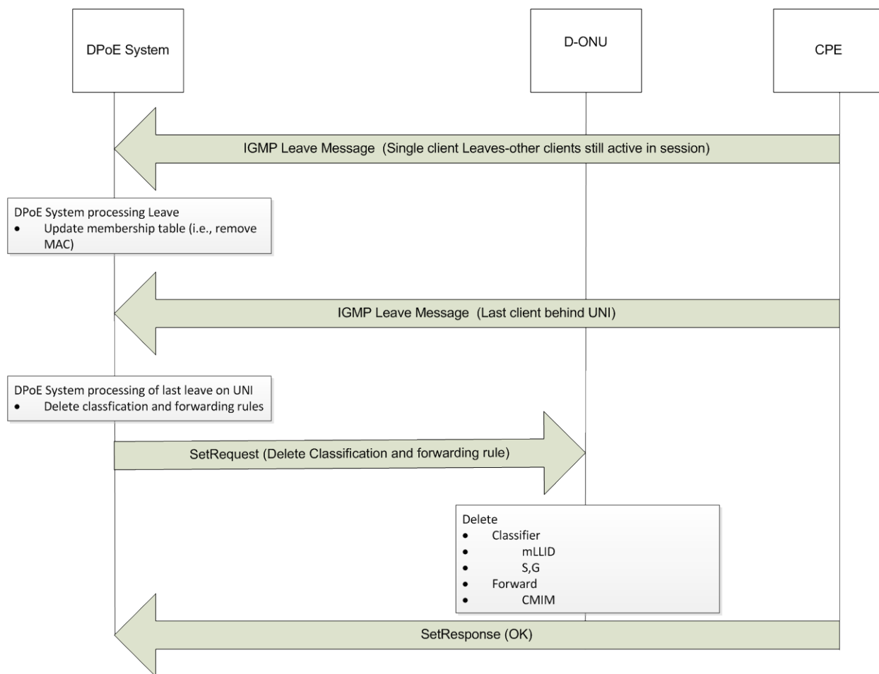
Figure 33 - Multicast Leave Processing 69
