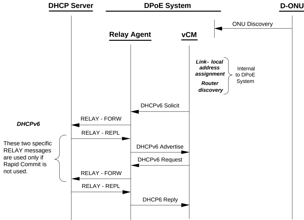
Figure 19 - Establishment of IPv6 Network Connectivity
