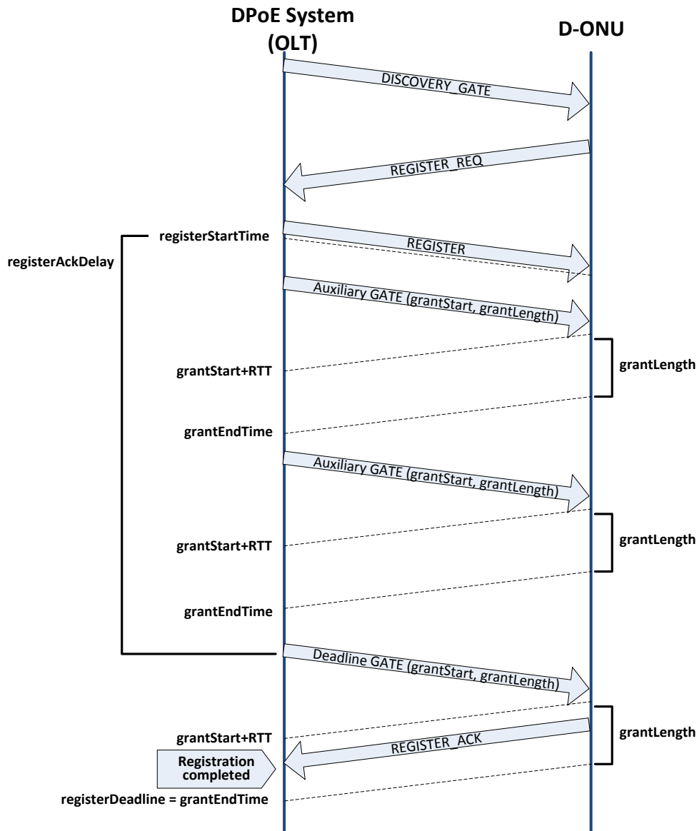
Figure 26 - DPoE MPCP Discovery Process Using Multiple GATE Messages, REGISTER_ACK Message Arrived in Grant from Deadline GATE message.
