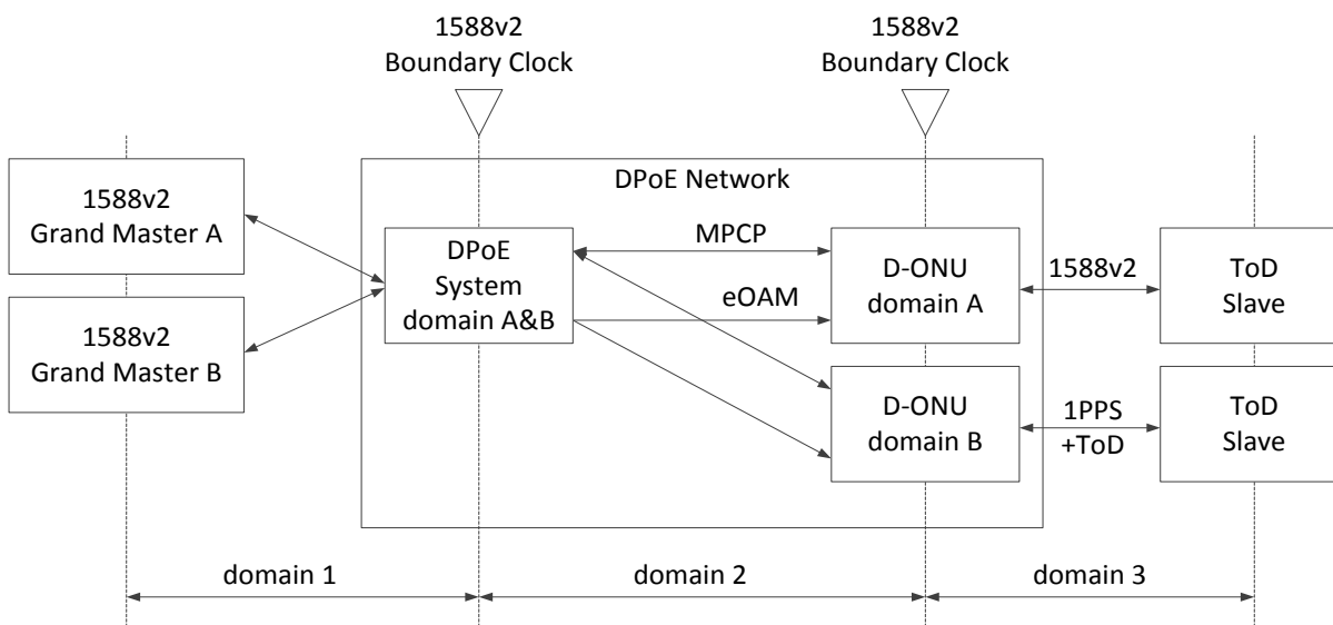
Figure 7 - Graphical Representation of the EToD Distribution Mechanism in DPoE Network
