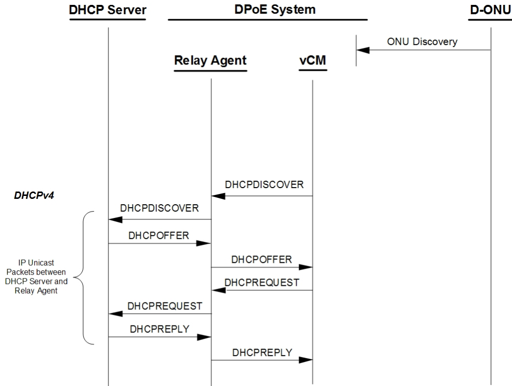
Figure 18 - Establishment of IPv4 Network Connectivity
