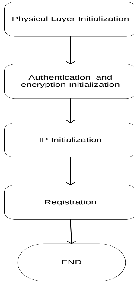
Figure 5 - D-ONU Initialization
