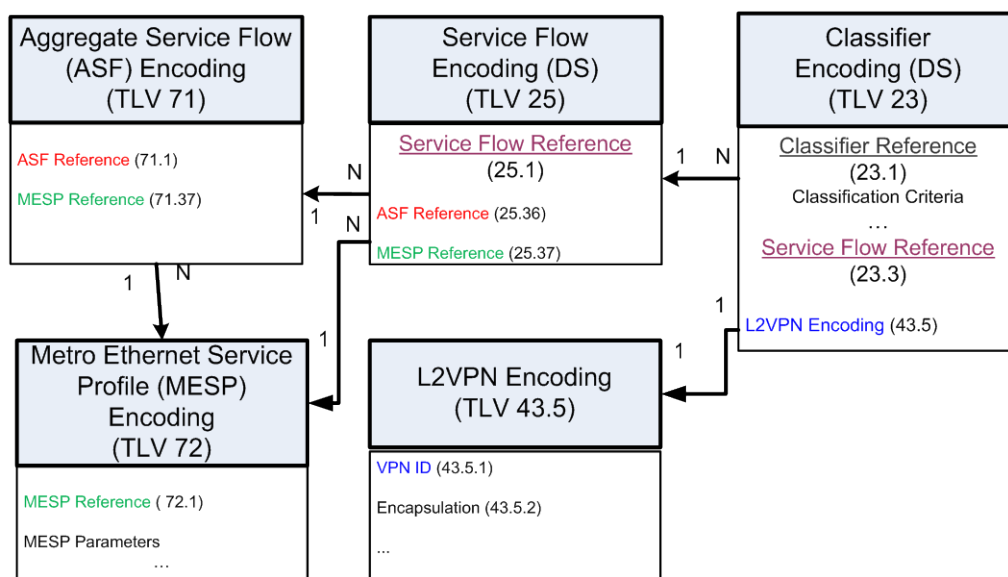
Figure 10 - Object Model Diagram for Downstream ASF and MESP TLVs and Relationship to L2VPN Model
