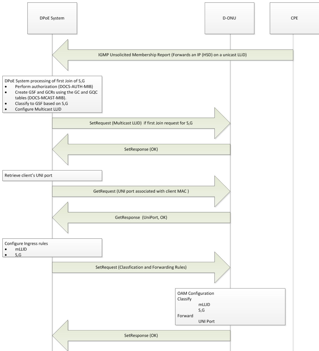
Figure 29 - Dynamic Join
