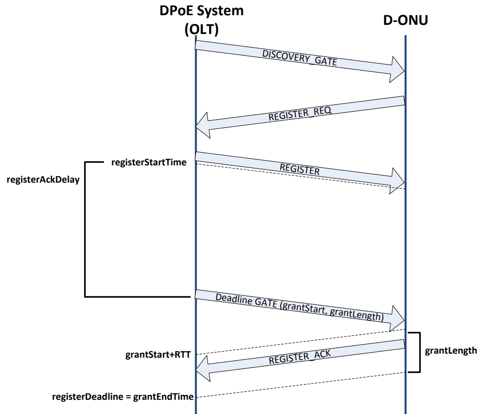
Figure 24 - Discovery Process with registerStartTime, registerAckDelay, and registerDeadline.
