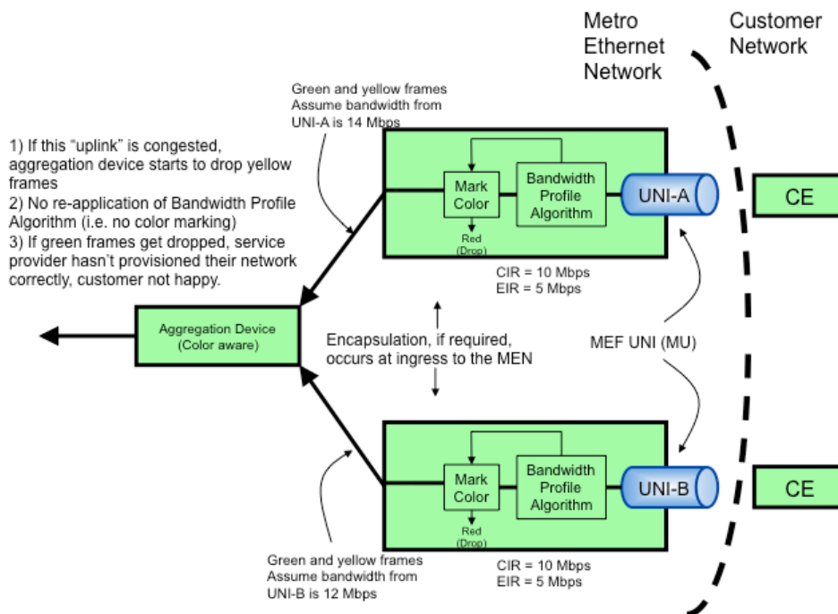
Figure 27 - Behavior of Devices within MEF Network
