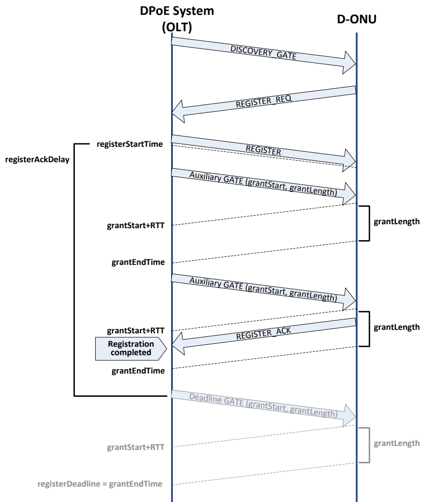
Figure 25 - DPoE MPCP Discovery Process Using Multiple Auxiliary GATE Messages, REGISTER_ACK Message Arrived in Grant from Auxiliary GATE Message.
