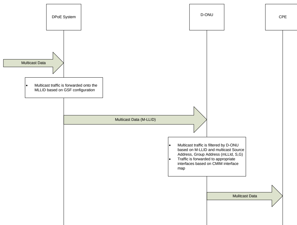
Figure 31 - Downstream Multicast Data Traffic Forwarding
