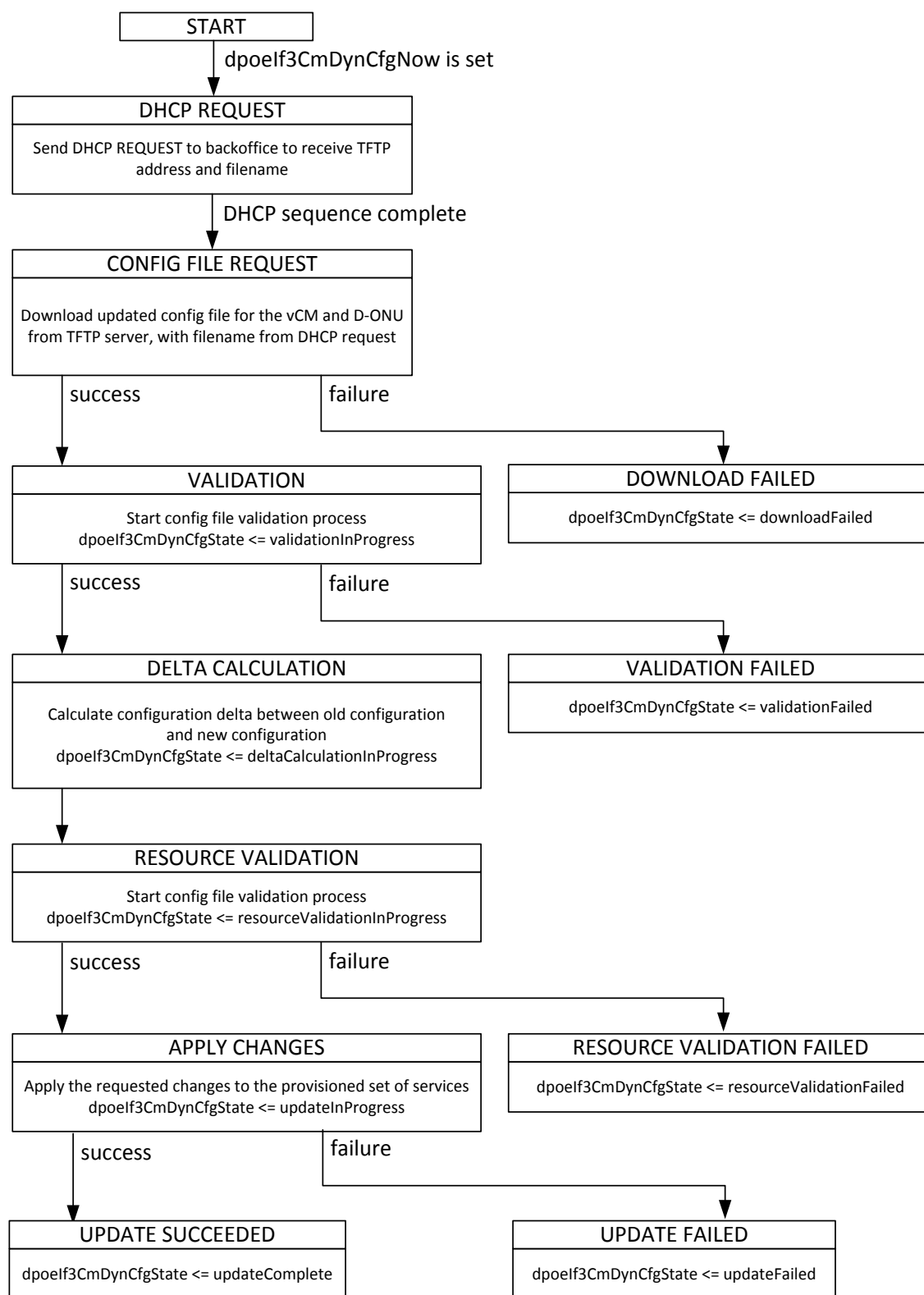
Figure 22 - Operation of the vCM
