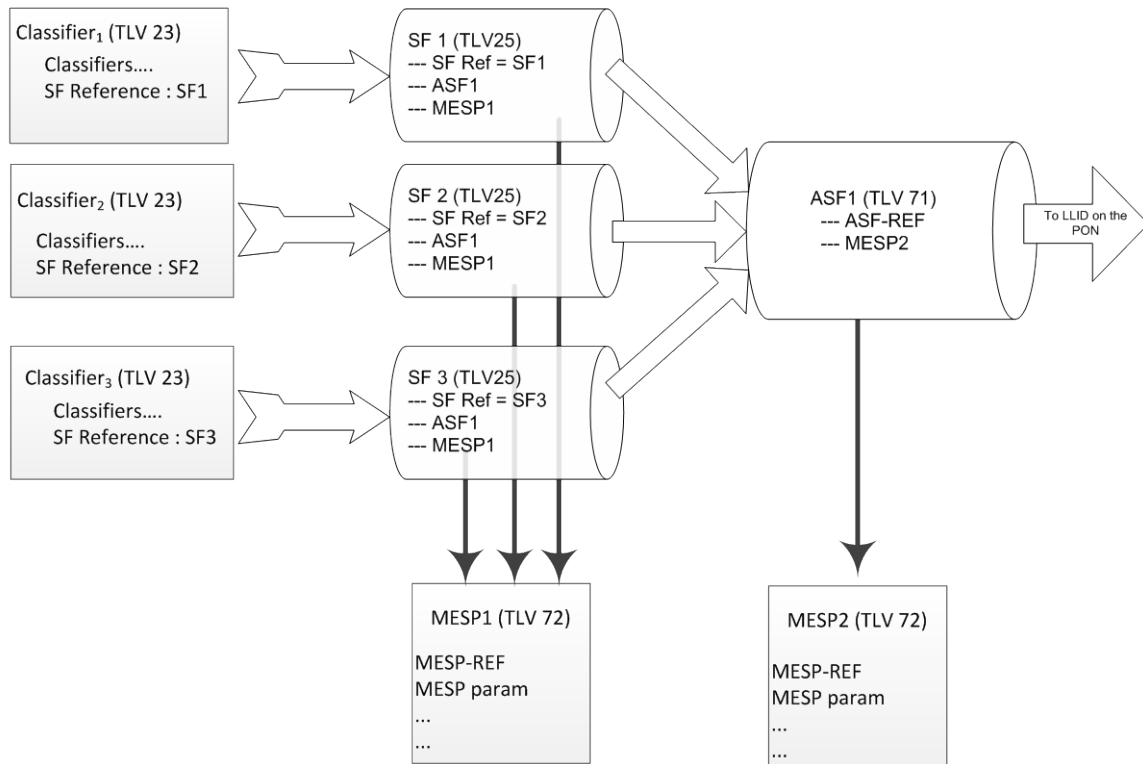
Figure 12 - Example of Three Downstream SFs (SF1, SF2, and SF3) Aggregated into ASF
