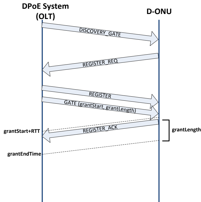
Figure 23 - MPCP Discovery Process Message Sequence.
