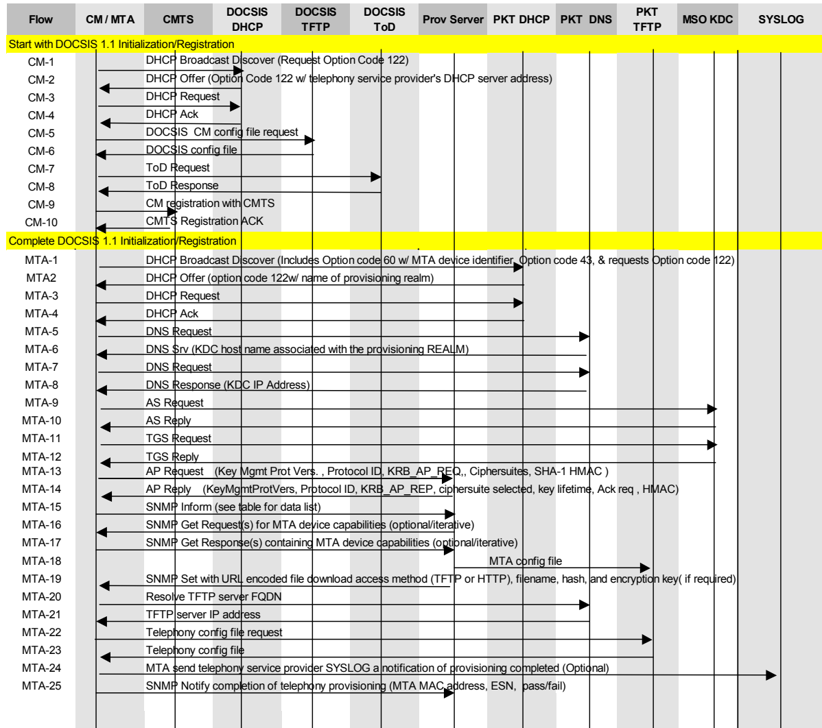
Figure 6. Embedded-MTA Secure Power-on Initialization Flow
