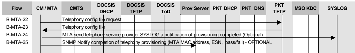
Figure 7. Embedded-MTA Basic Power-on Initialization Flow
