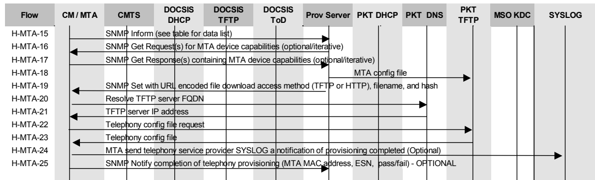
Figure 8. Embedded-MTA Hybrid Power-on Initialization Flow
