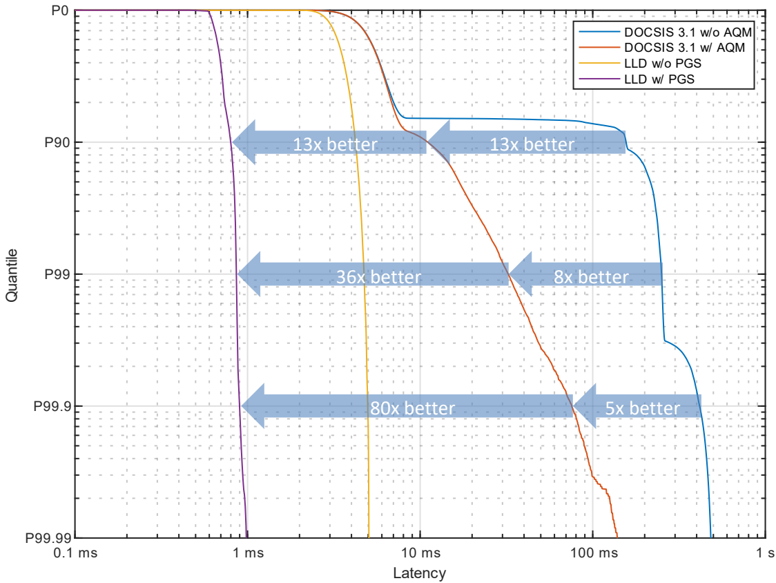
Figure 9. Overall Round-Trip Latency Performance for NQB-Marked Traffic
