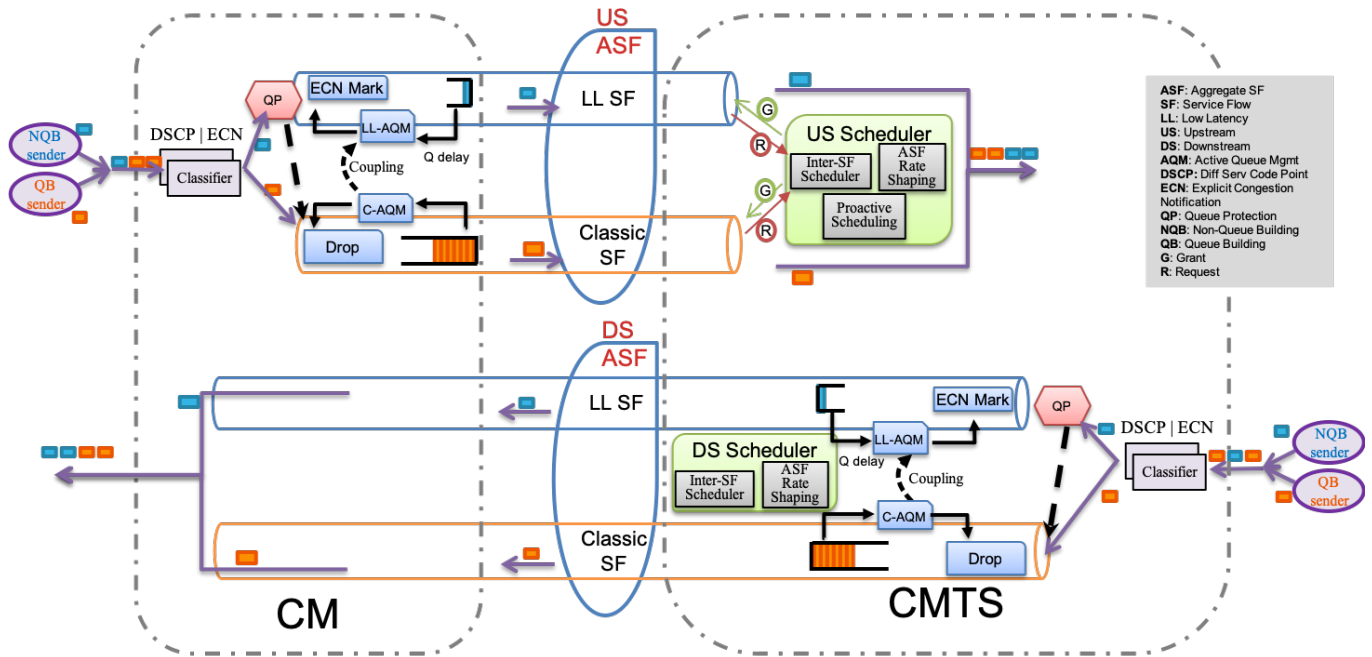
Figure 10. ASFs, SFs, and the Low Latency DOCSIS Architecture
