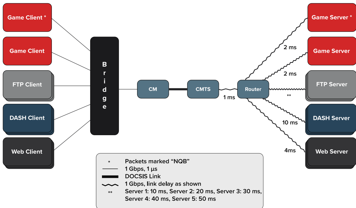
Figure 13. NS3 Network Topology
