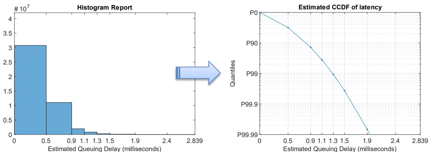
Figure 11. Example of Using a Latency Histogram Report to Estimate Latency Quantiles
