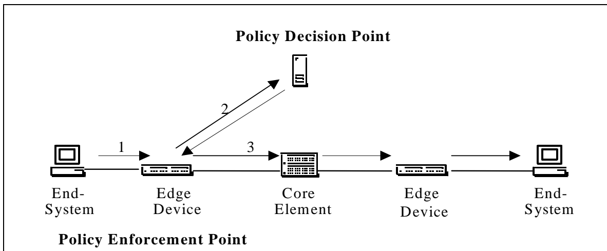
Figure 19. COPS Protocol
