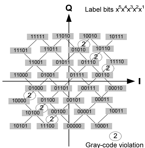
Figure 6-24 - 32 QAM Symbol Mapping 9
