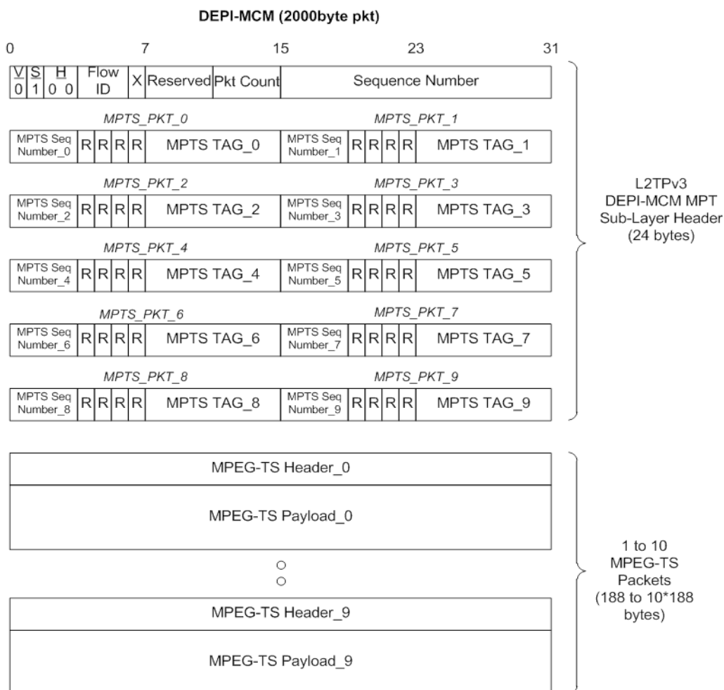
Figure 55 - MCM Sublayer Header and Payload
