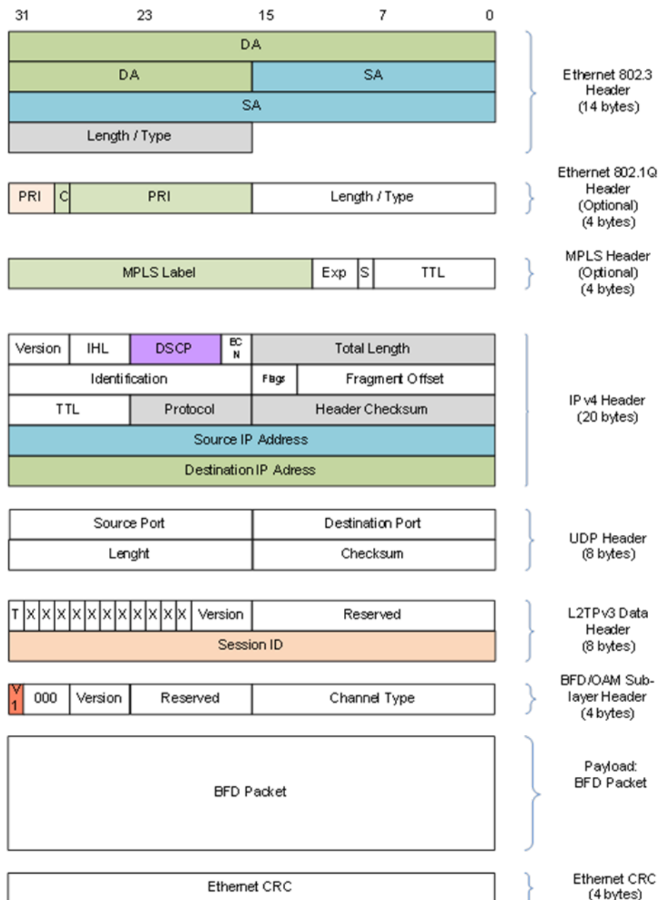
Figure 61 - BFD Sublayer (with UDP)
