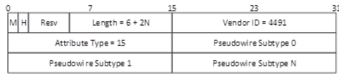
Figure 36 - DEPI Pseudowire Subtype Capabilities List AVP
