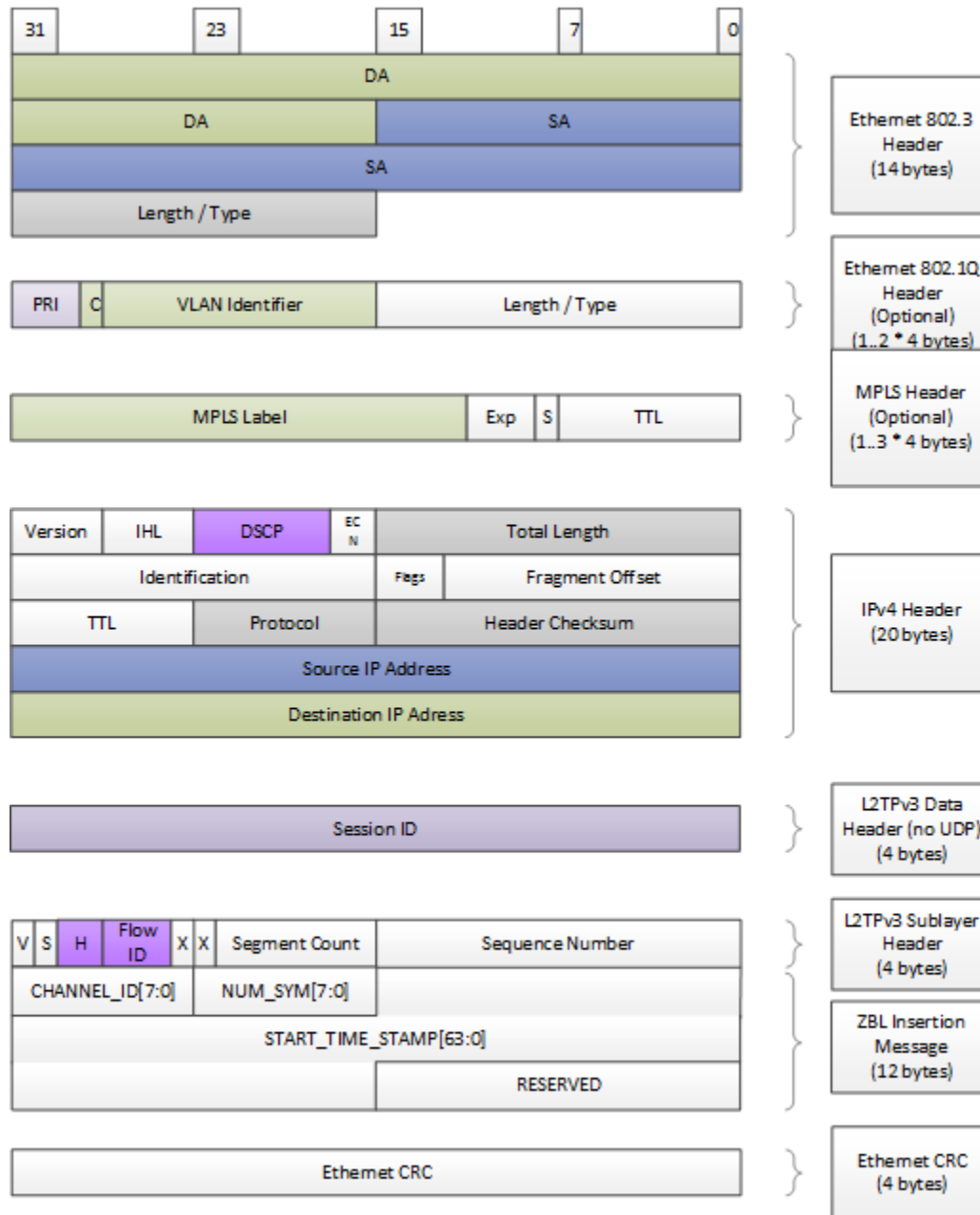
Figure 62 - L2TPv3 Packet Format for ZBL Insertion Message
