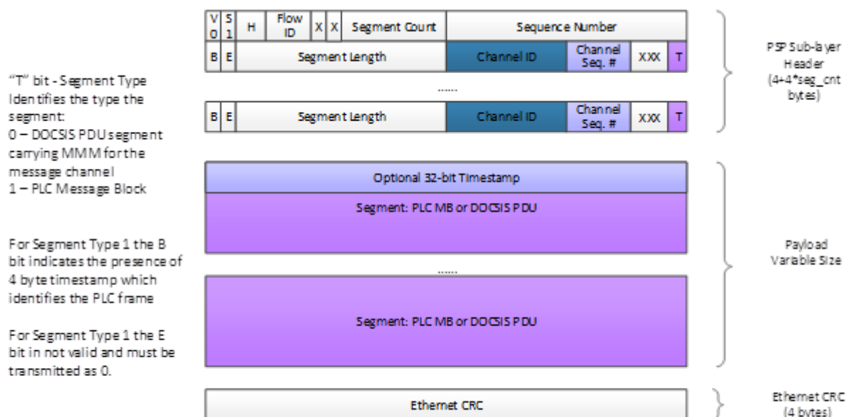
Figure 57 - Use of DEPI PSP Sublayer Header for PLC Subchannel
