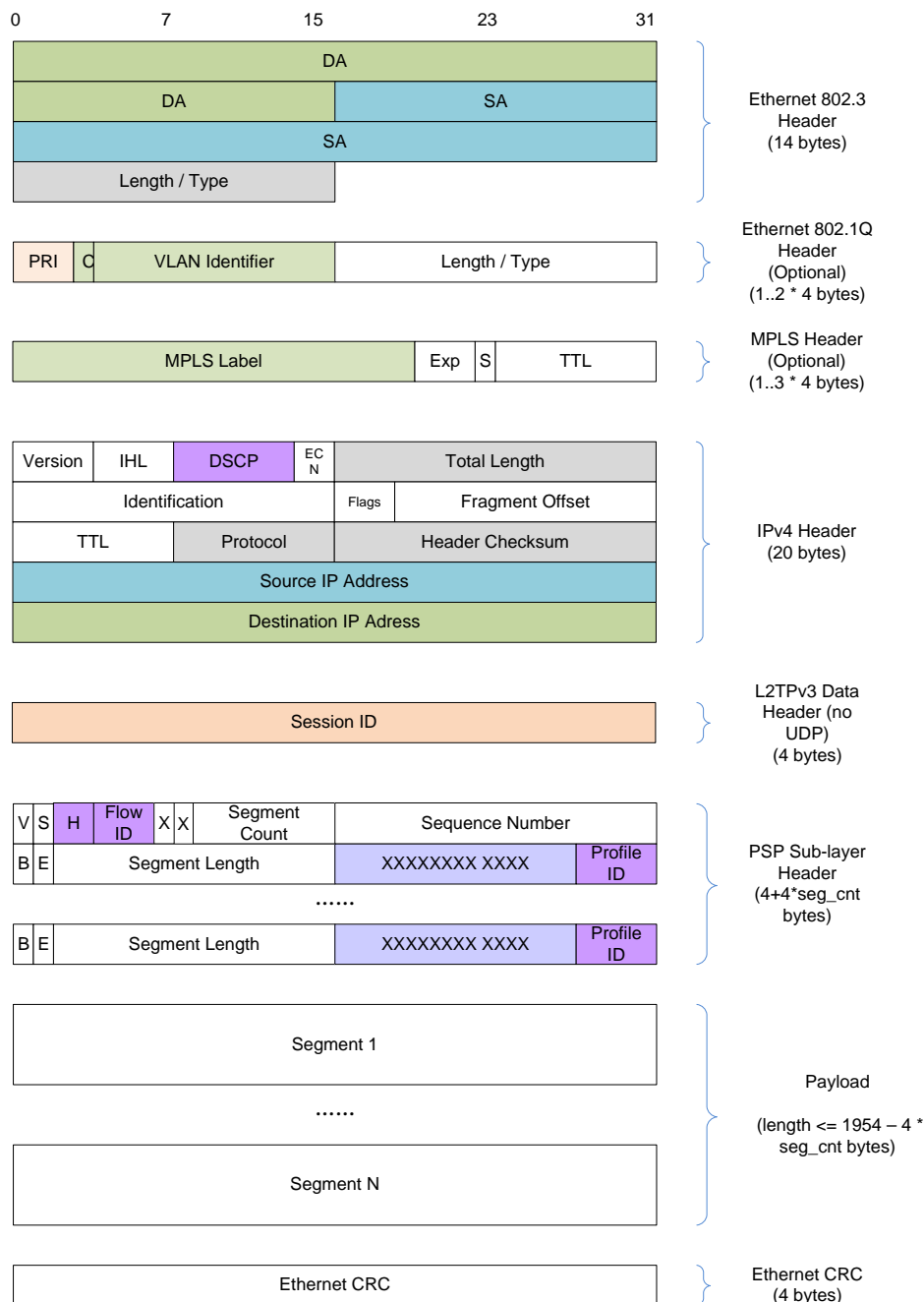
Figure 58 - Example of a Complete DEPI Packet Format (IPv4) with Extras
