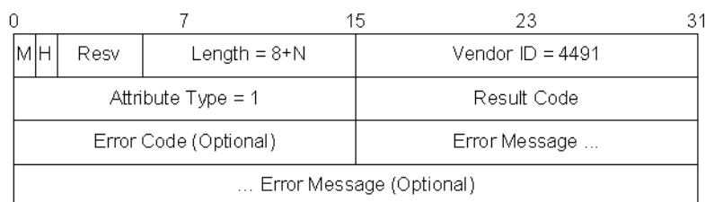
Figure 38 - DEPI Result and Error Code AVP
